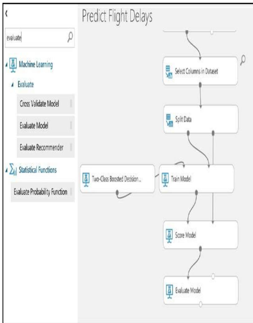
Figure 2-74 Evaluate a model with Evaluate Model
