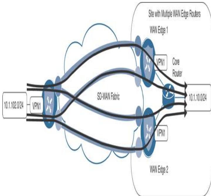
Figure 6-42 Four Paths to 10.1.10.0/24
