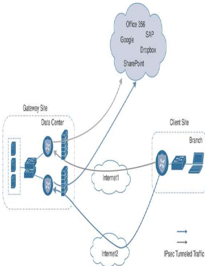
Figure 11-4 Cloud Access Through a Gateway
