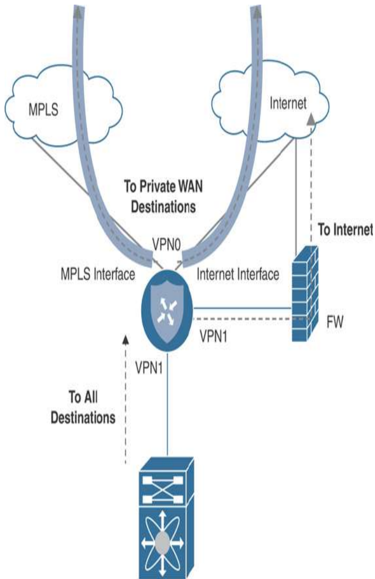
Figure 12-18 DIA Through Firewall
