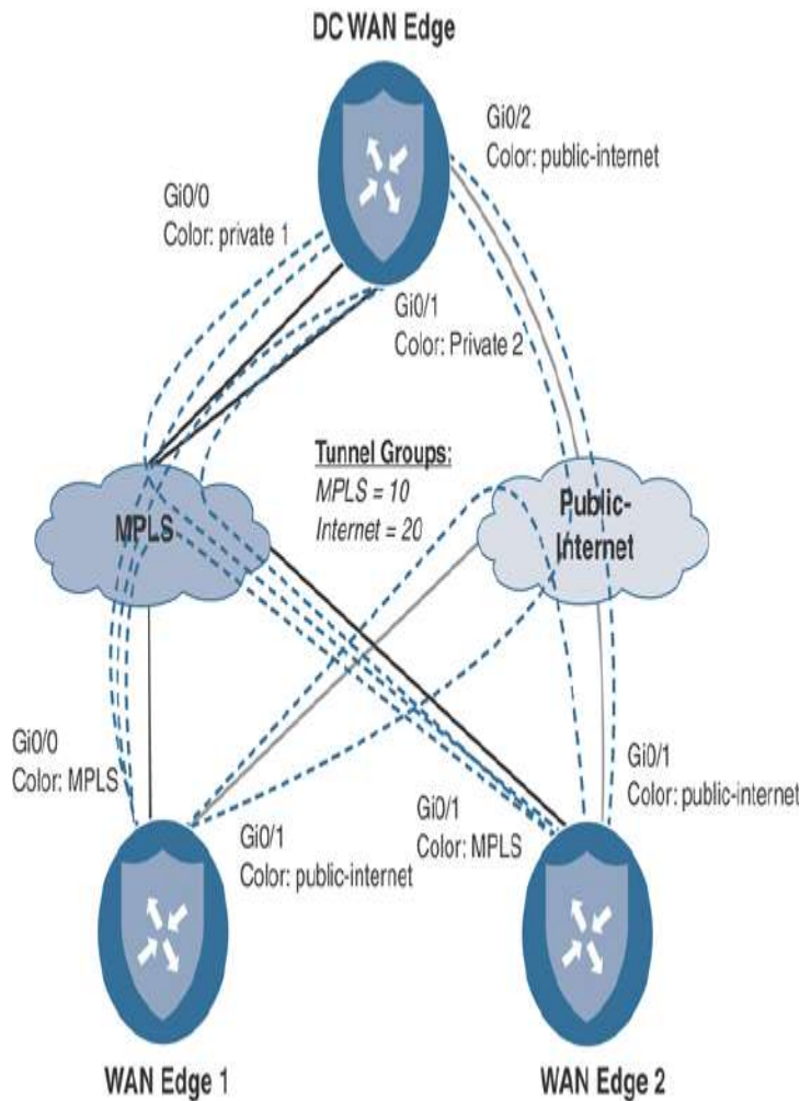
Figure 3-18 TLOC Colors with Tunnel Groups
