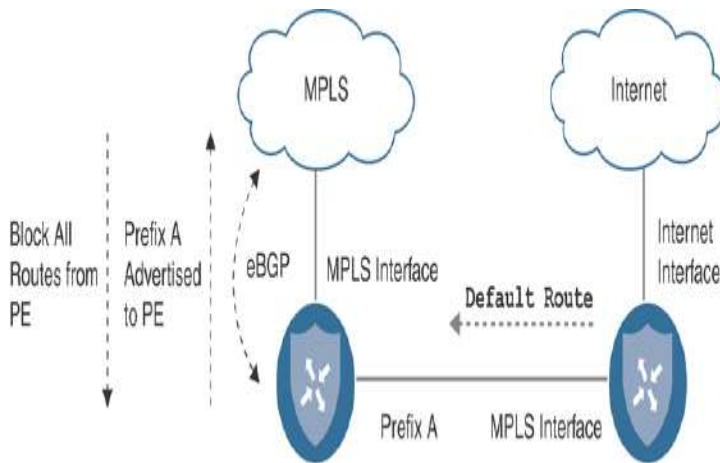
Figure 12-15 TLOC Extension Private
