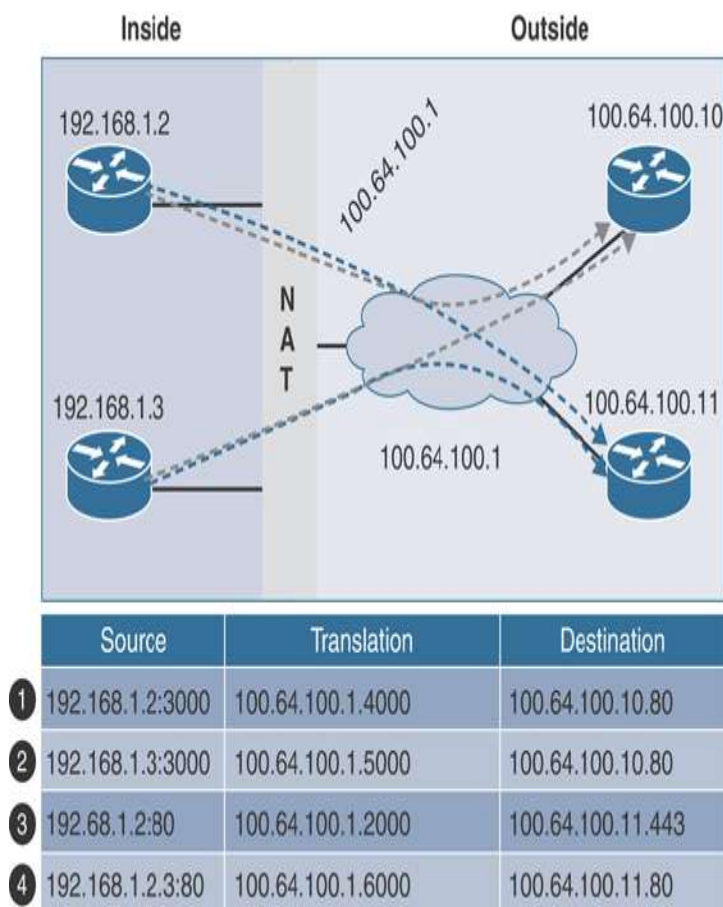
Figure 3-20 Symmetric NAT
