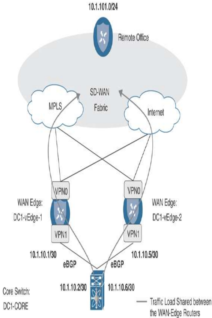
Figure 9-2 Data Center Topology
