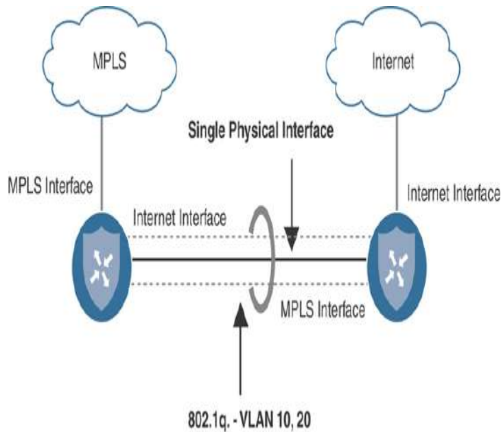
Figure 12-14 TLOC Extension Sub-Interfaces
