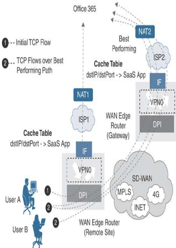
Figure 11-9 Cloud onRamp for SaaS and NAT
