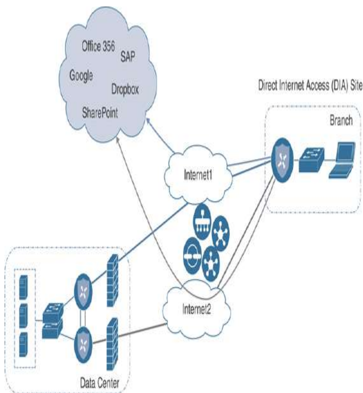
Figure 11-3 Direct Cloud Access/Direct Internet Access
