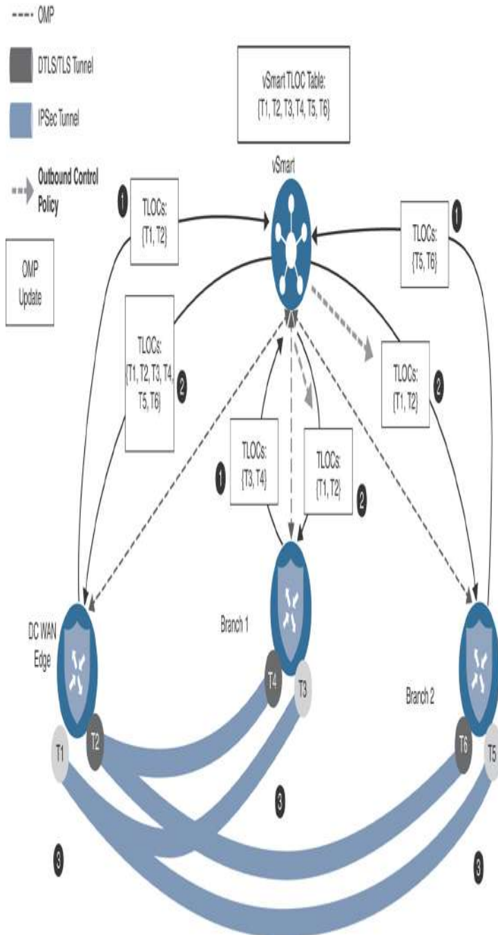
Figure 6-5 Illustration of Control Policies Filter TLOCs
