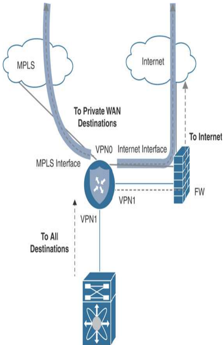
Figure 12-19 Transport and DIA Through Firewall
