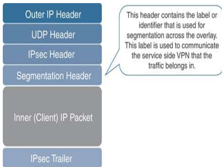
Figure 2-2 Cisco SD-WAN Packet Format
