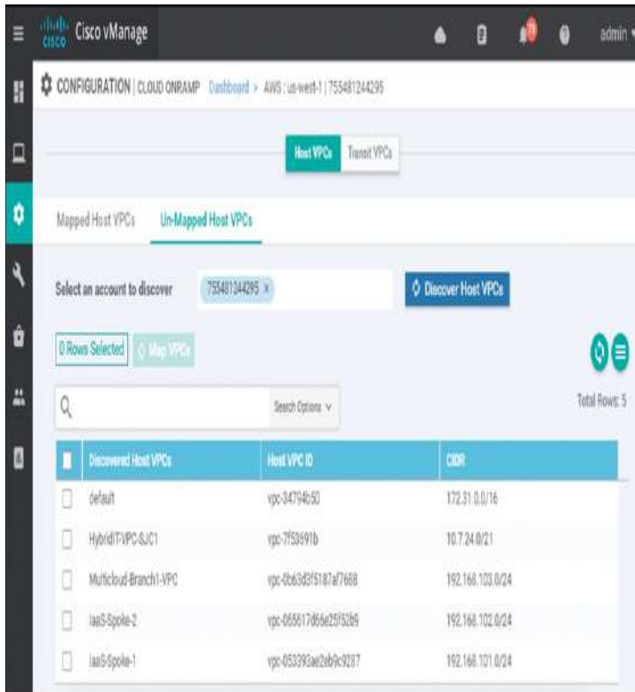
Figure 11-40 Discovered VPCs
