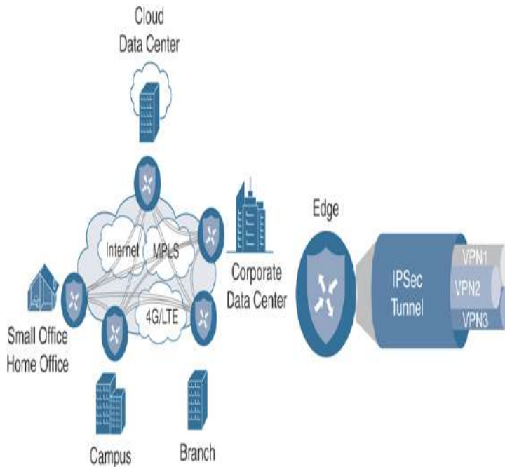
Figure 1-10 End-to-End Segmentation
