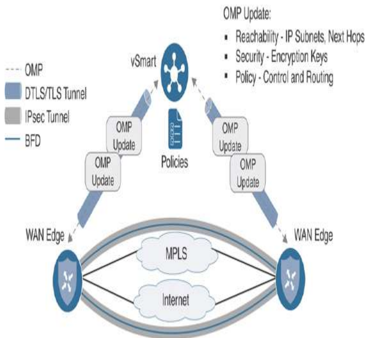
Figure 2-7 Cisco Control Plane and Data Plane Overview
