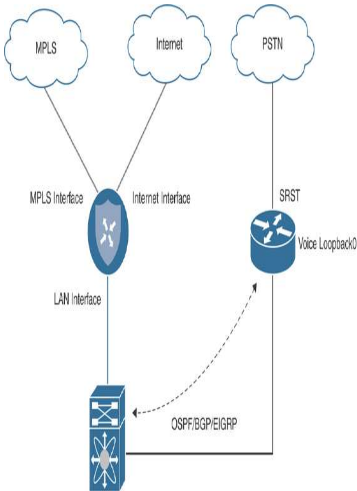
Figure 12-22 Voice Services Integration—L3
