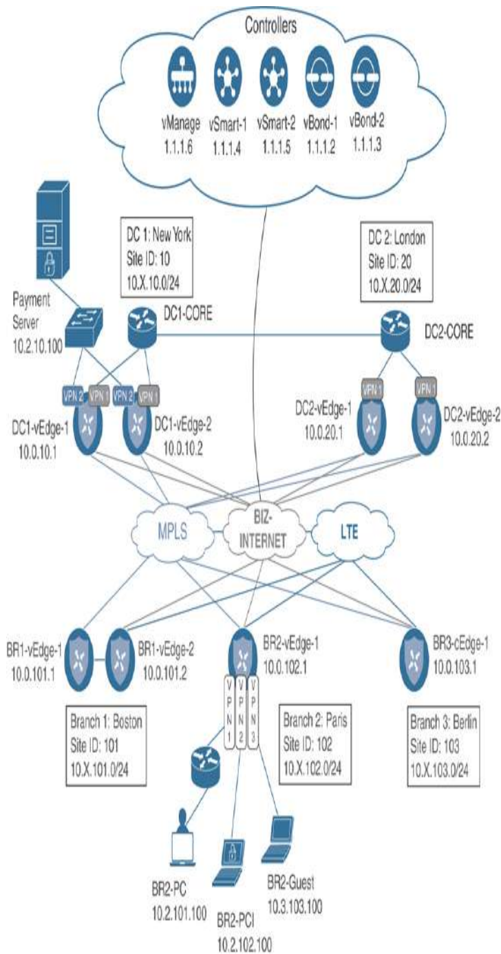
Figure 7-2 Network Topology for Chapter 7
