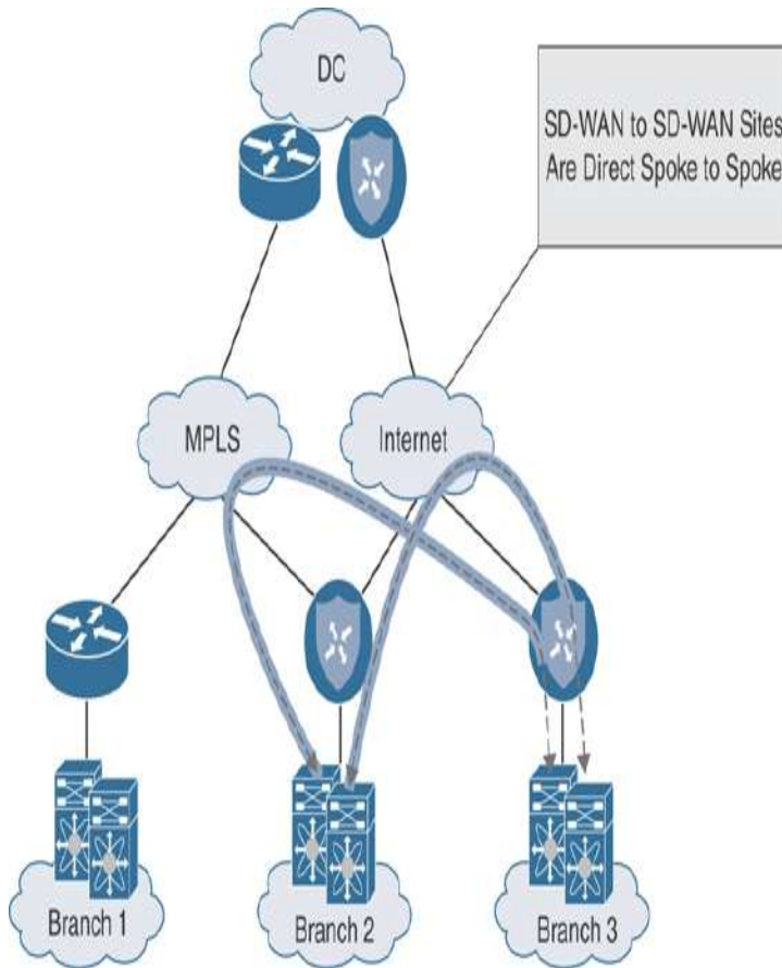
Figure 12-24 SD-WAN to SD-WAN Site Overlay-Only Traffic Flow
