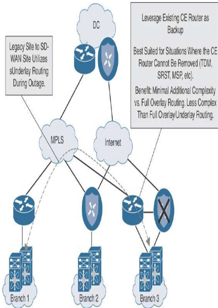
Figure 12-31 Overlay with Underlay Backup Traffic Flow During Failover
