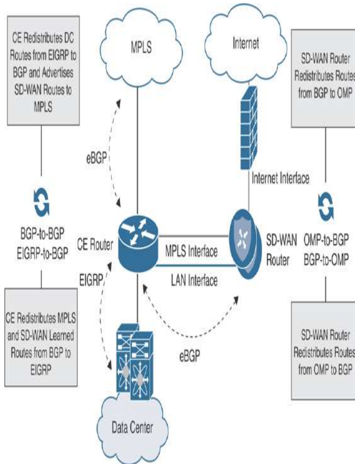
Figure 12-7 Service-Side CE Integration
