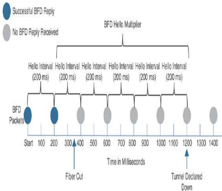
Figure 8-15 BFD Path Liveliness Detection
