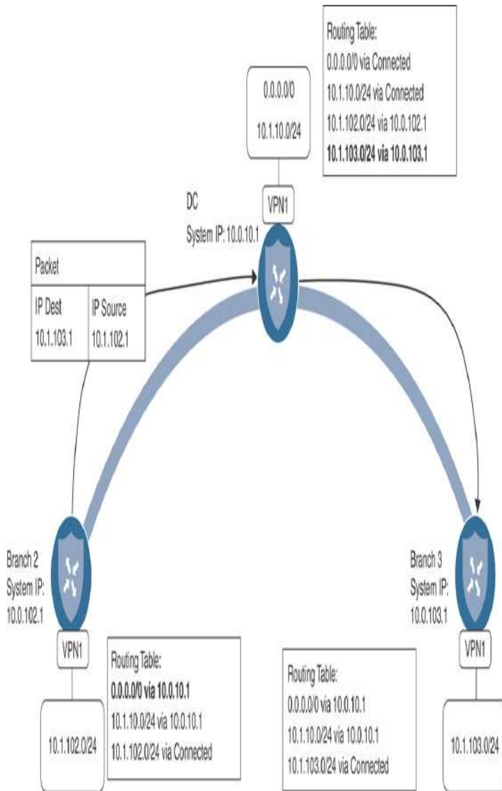
Figure 6-18 Enabling Branch-to-Branch Communication with Summarization
