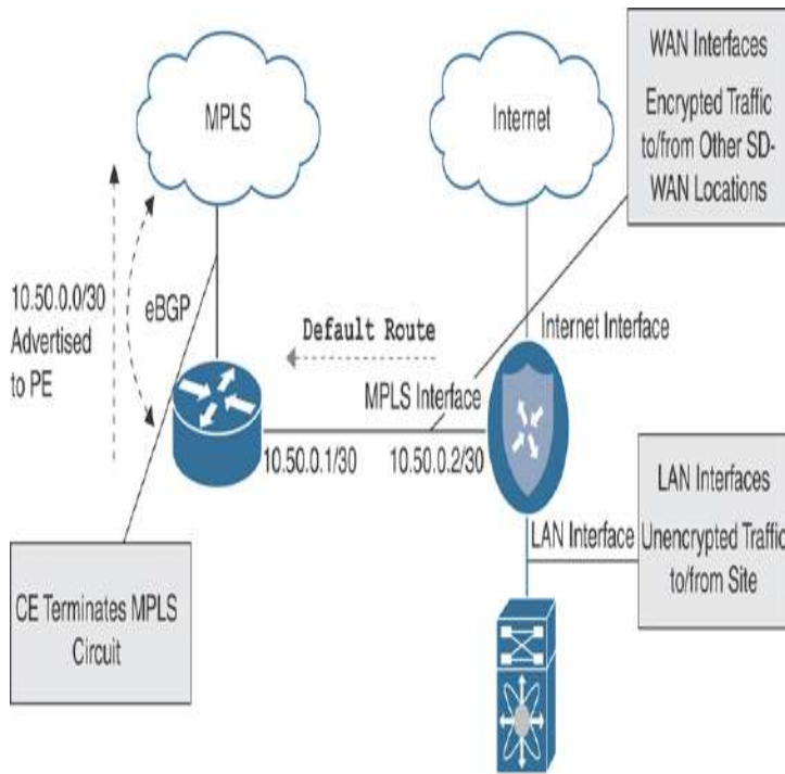
Figure 12-17 Branch CE Integration
