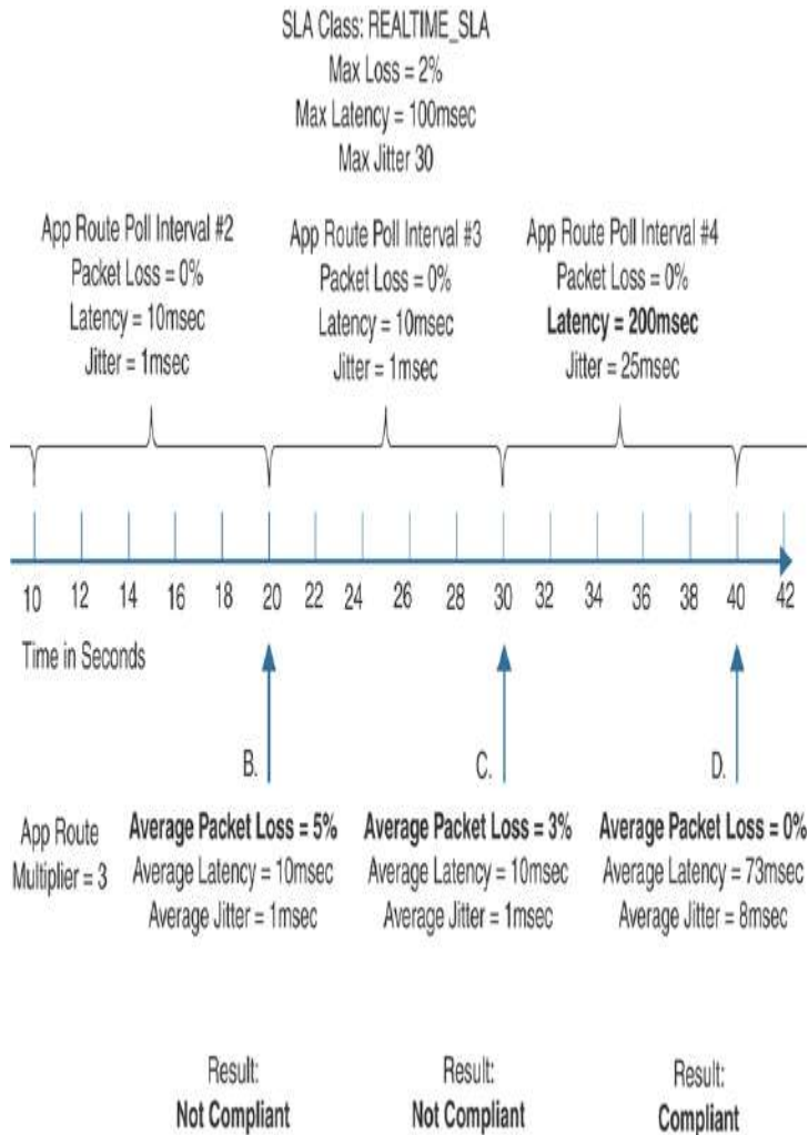
Figure 8-18 SLA Calculations with Multiple App-Route Poll Intervals
