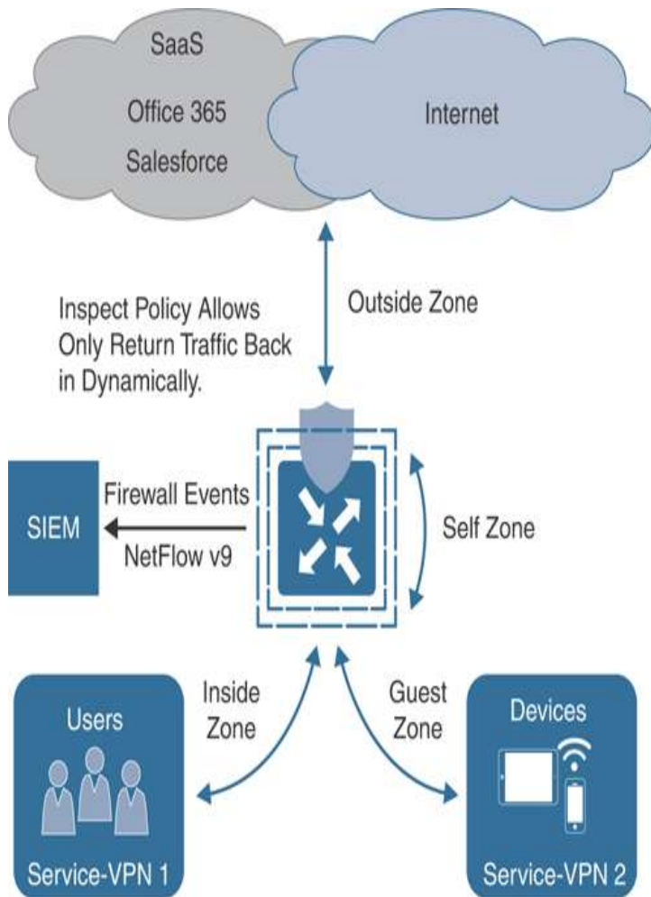
Figure 10-4 Application-Aware Enterprise Firewall
