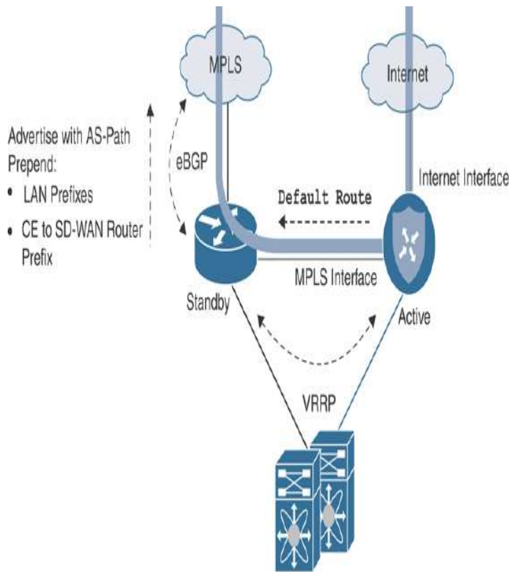
Figure 12-25 Overlay with Underlay Backup—L2 Design
