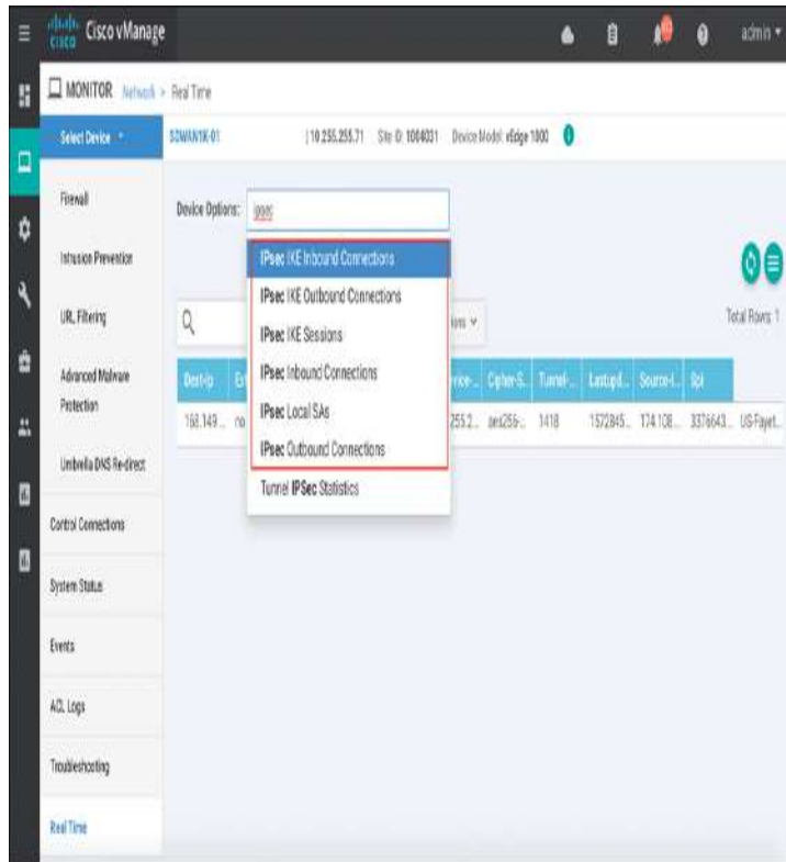
Figure 10-39 Real-Time Tunnel Information
