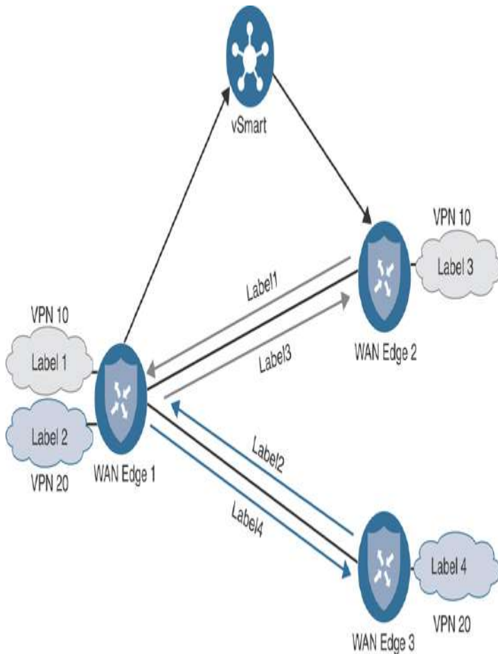
Figure 3-27 Overlay Label Switching
