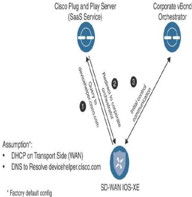
Figure 4-14 Plug and Play Workflow
