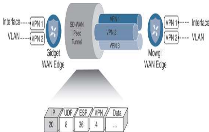
Figure 3-15 Cisco SD-WAN Segmentation
