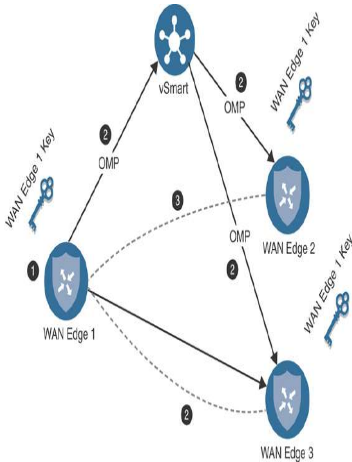
Figure 3-28 SD-WAN Key Exchange
