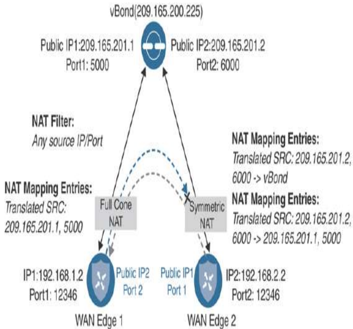
Figure 3-25 Symmetric and Full Cone NAT
