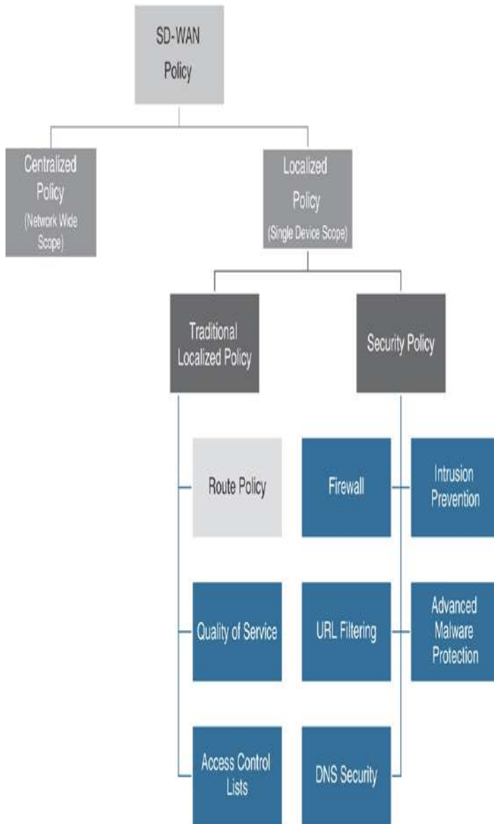
Figure 5-3 Types of Cisco SD-WAN Localized Policies
