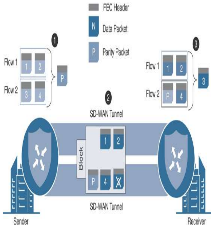
Figure 7-24 FEC Illustration
