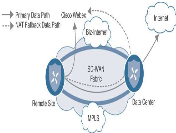
Figure 7-20 Illustrated NAT Fallback Data Path
