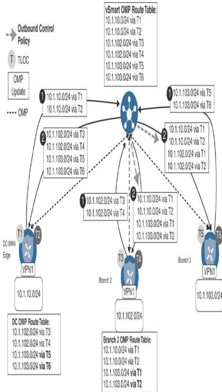
Figure 6-21 Enabling Branch-to-Branch Communication with TLOC Manipulation
