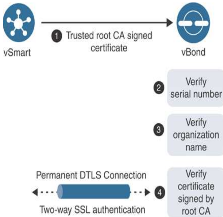
Figure 3-3 DTLS Tunnel Authentication
