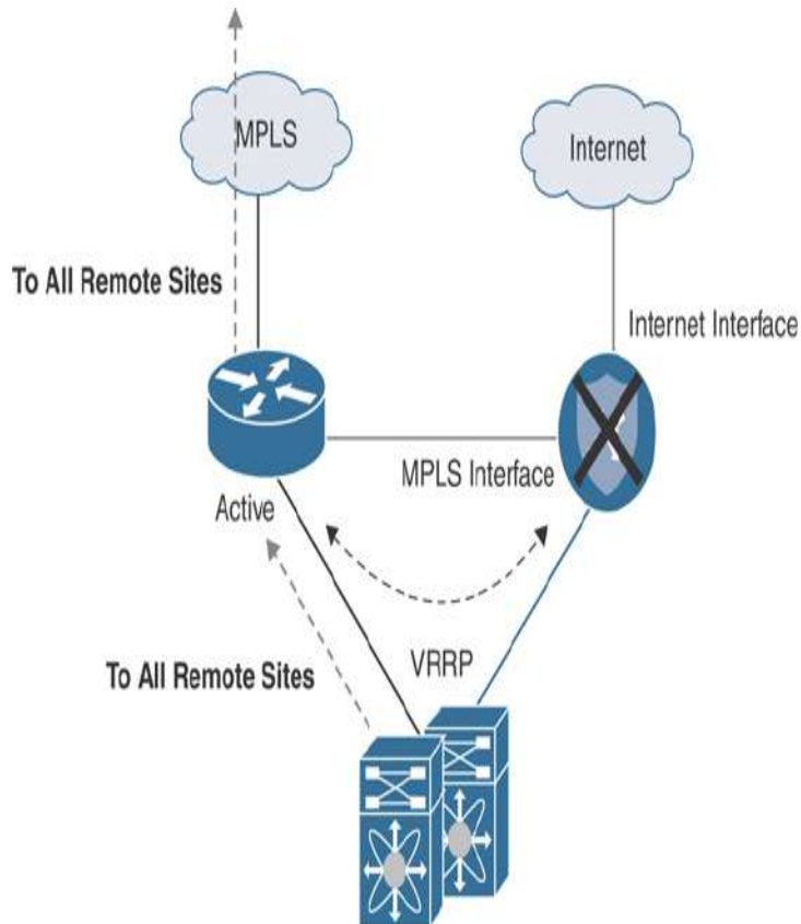
Figure 12-27 Overlay with Underlay Backup—L2 Design Traffic Flow During Failover
