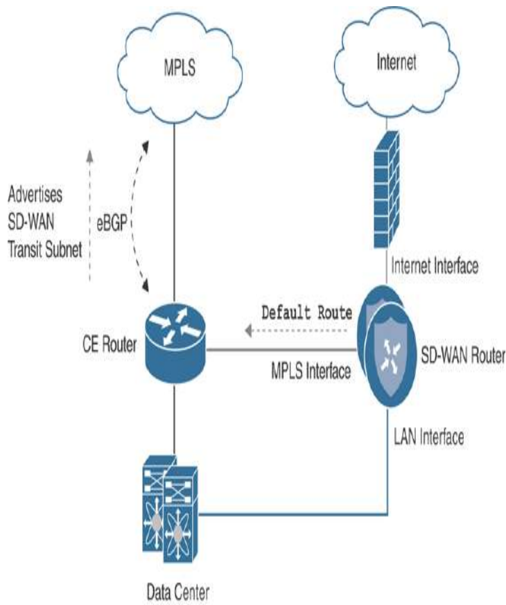
Figure 12-2 Data Center Direct Transport Side
