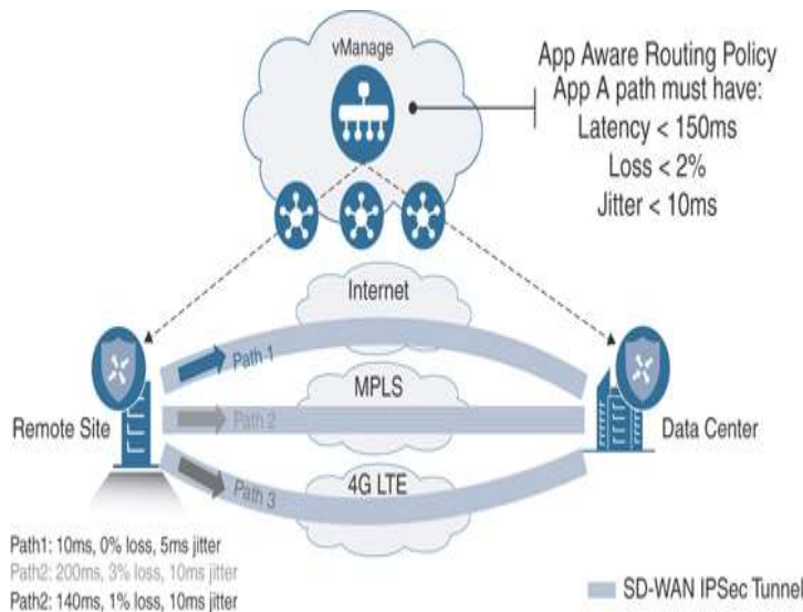
Figure 1-9 Routing Based on Application Performance
