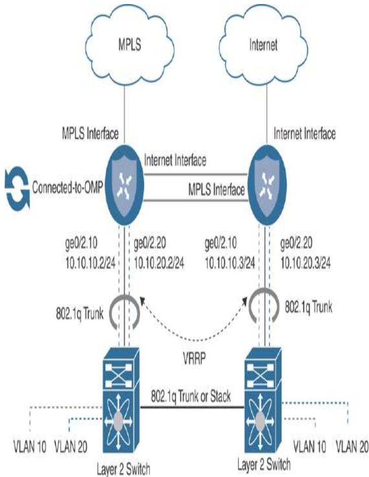
Figure 12-11 Complete CE Replacement—Dual Router L2 Branch
