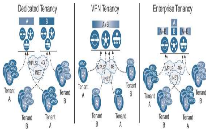
Figure 2-10 Cisco SD-WAN Multi-Tenancy Options
