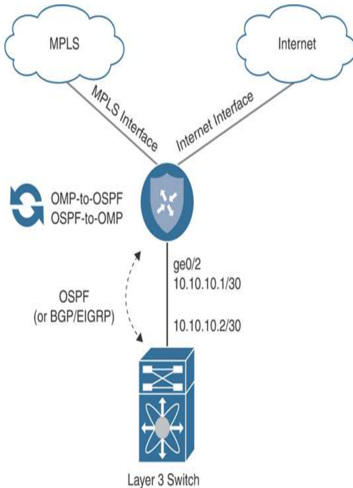
Figure 12-10 Complete CE Replacement—Dual Router L3 Branch
