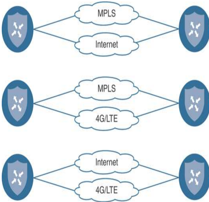
Figure 1-5 Common Hybrid WAN Topologies
