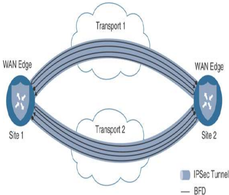
Figure 8-11 BFD Packets in the SD-WAN Fabric
