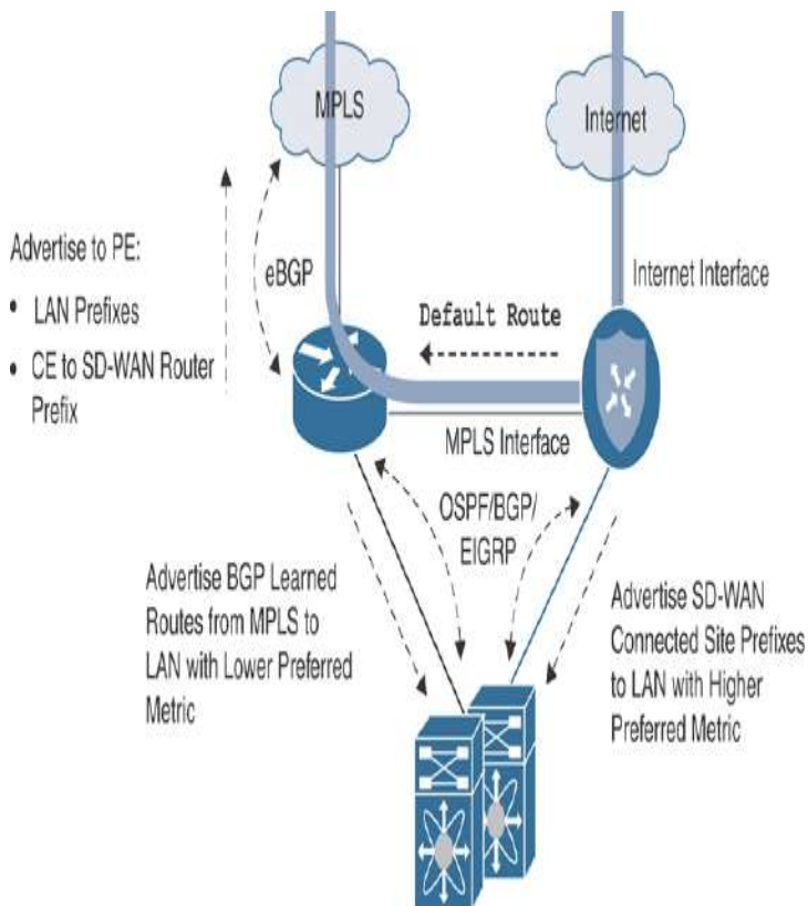
Figure 12-34 Full Overlay with Underlay Routing CE Integration
