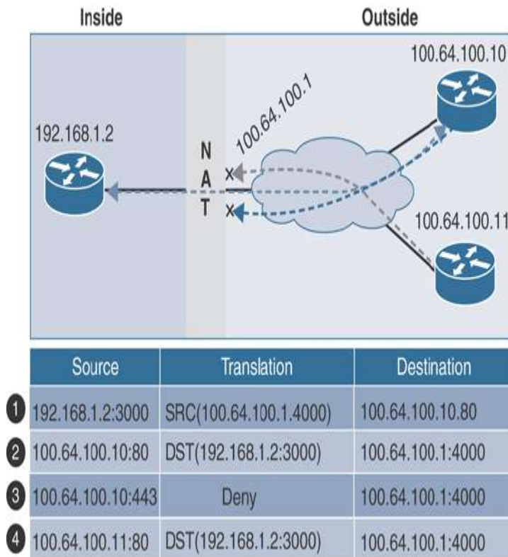
Figure 3-22 Port Restricted Cone NAT
