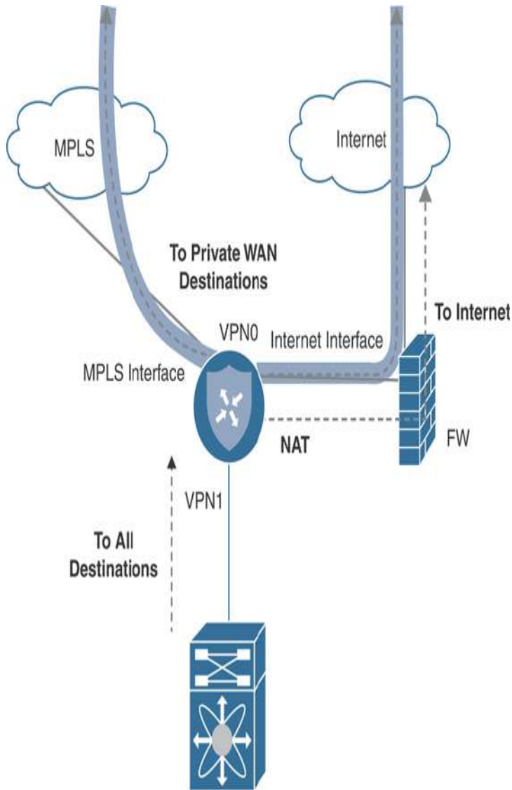
Figure 12-20 Transport and DIA Through Firewall Single Link
