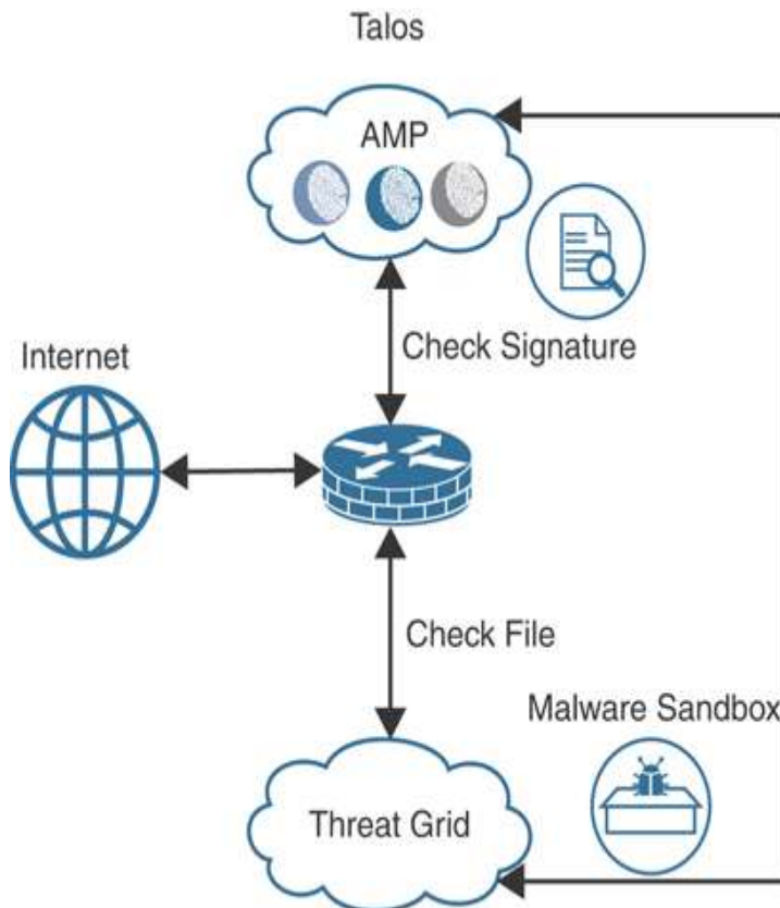
Figure 10-27 Advanced Malware Protection Process
