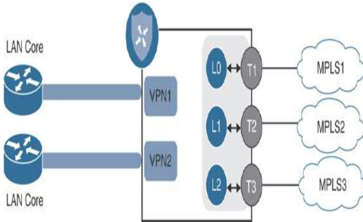
Figure 12-4 Loopback TLOC Bind Mode
