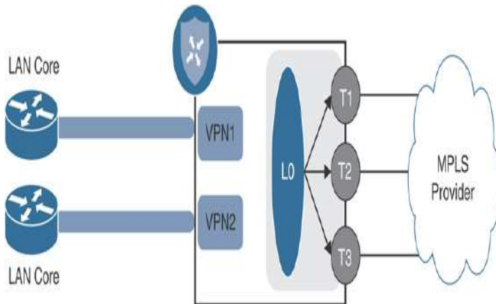
Figure 12-5 Loopback TLOC Standard Mode
