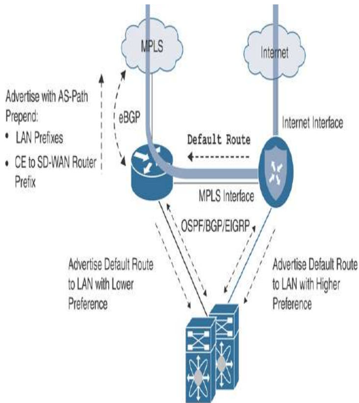
Figure 12-28 Overlay with Underlay Backup—L3 Design
