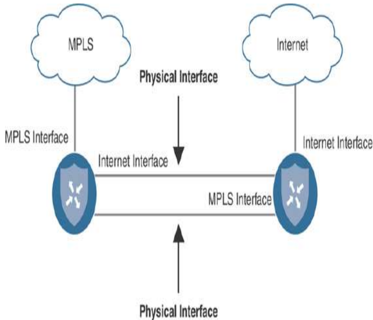
Figure 12-13 TLOC Extension Dedicated Interfaces
