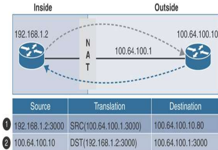
Figure 3-19 Full Cone NAT
