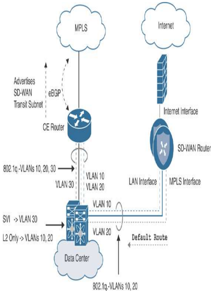
Figure 12-3 Data Center Indirect Transport Side
