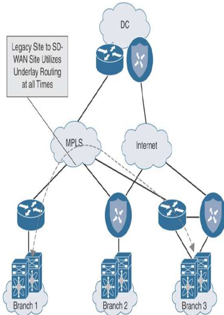
Figure 12-32 Full Overlay with Underlay Routing Legacy Site to SD-WAN Site Traffic Flow
