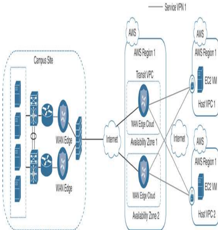
Figure 11-29 Cloud onRamp for IaaS Single Segment
