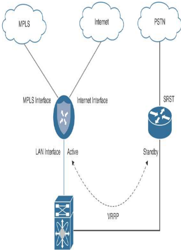
Figure 12-21 Voice Services Integration—L2
