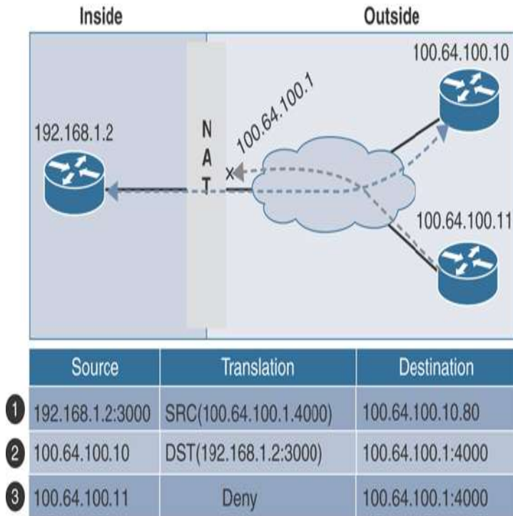
Figure 3-21 Address Restricted Cone NAT
