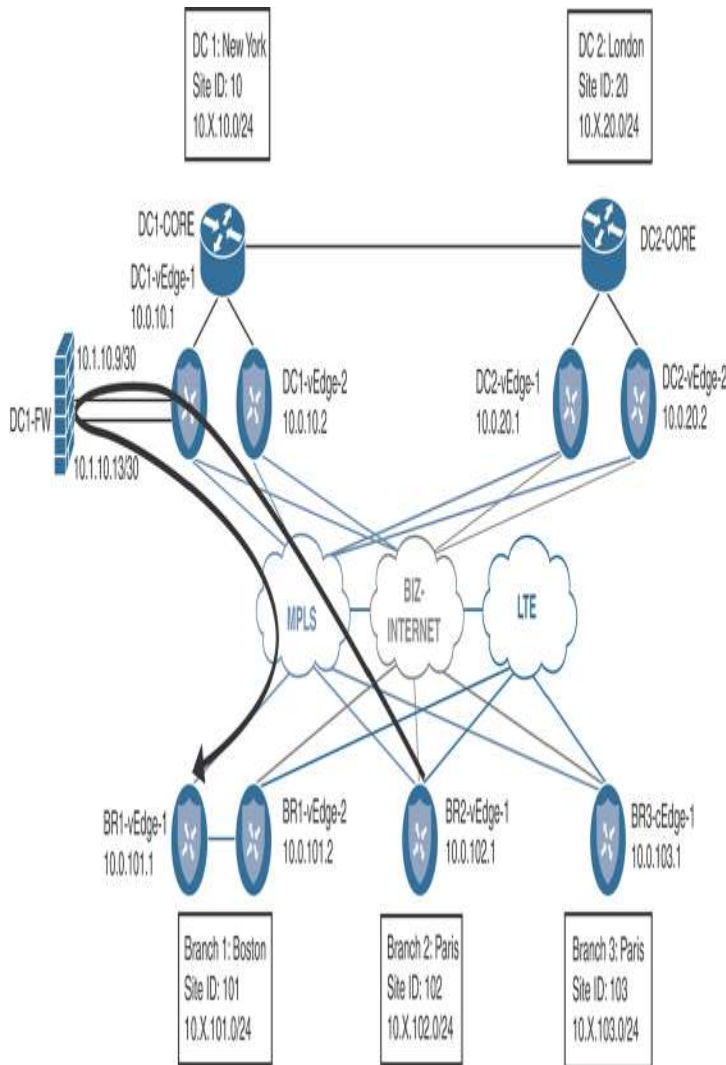
Figure 6-59 Using a Firewall at the Data Center to Inspect Flows Transiting Between Two Branch Sites
