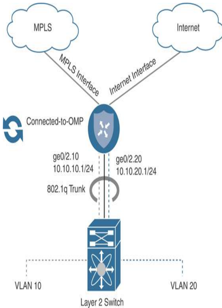
Figure 12-9 Complete CE Replacement—Single Router L2 Branch
