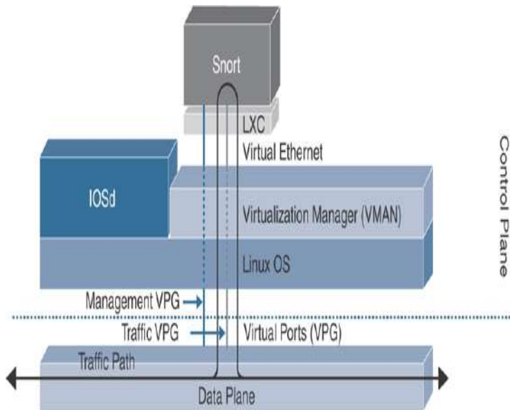
Figure 10-19 Snort Traffic Engine
