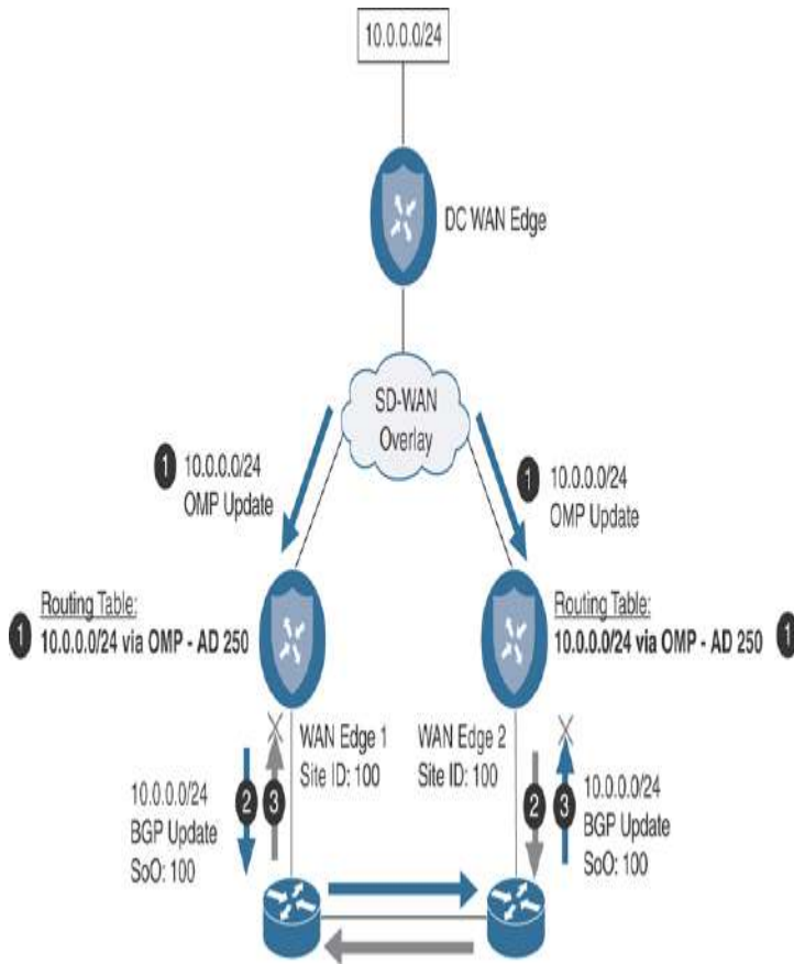
Figure 3-12 BGP Loop Prevention with Site of Origin
