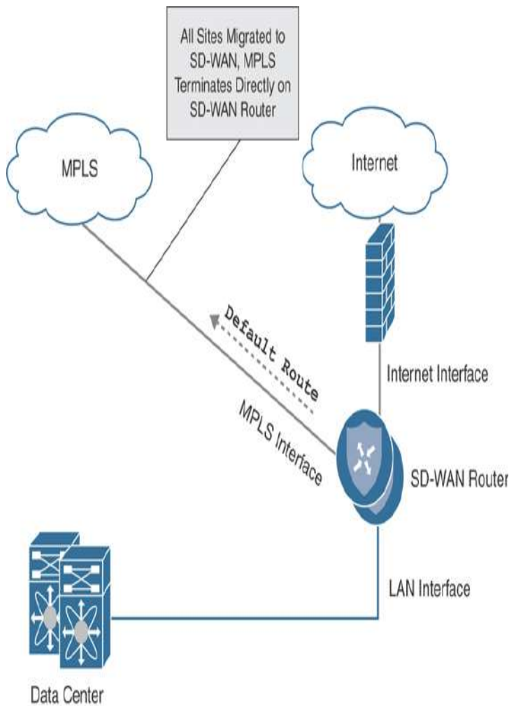
Figure 12-8 Direct Transport Termination
