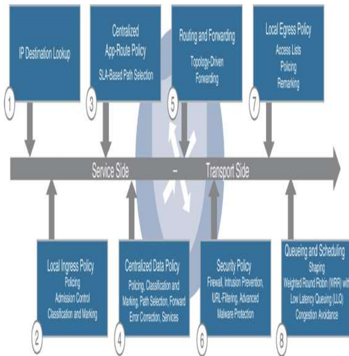
Figure 5-8 Packet Forwarding Order of Operations
