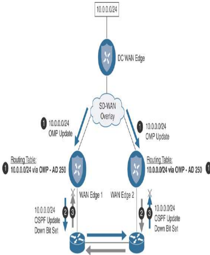
Figure 3-11 OSPF Loop Prevention with Down Bit
