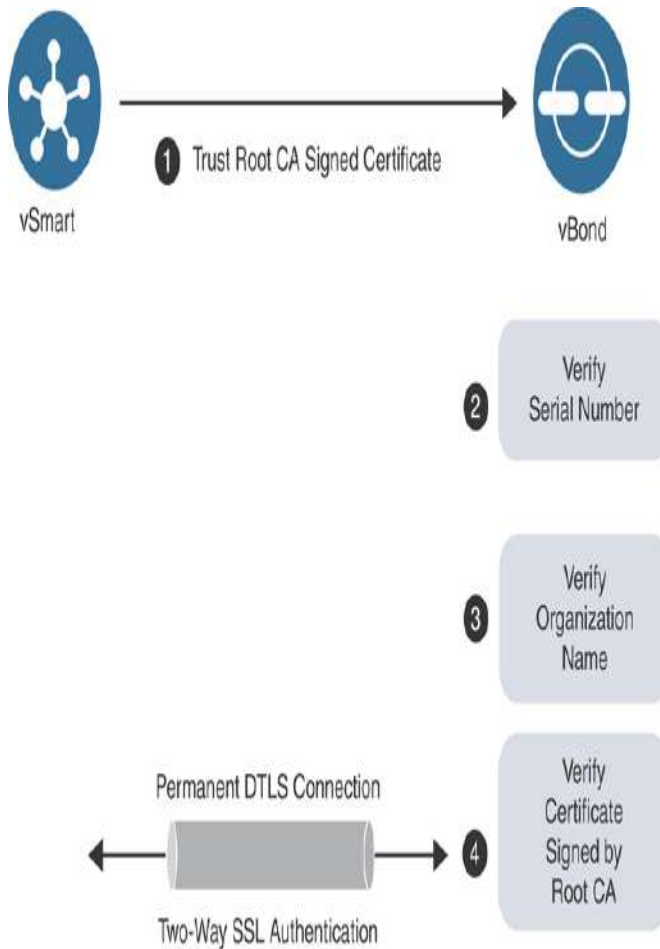
Figure 13-4 Certificate Authentication Process
