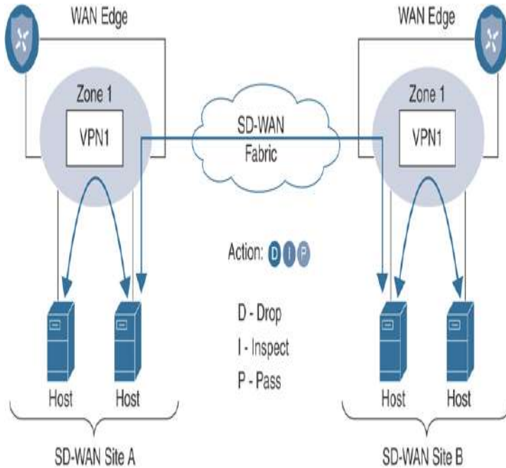
Figure 10-6 Intra-Zone Firewall Application
