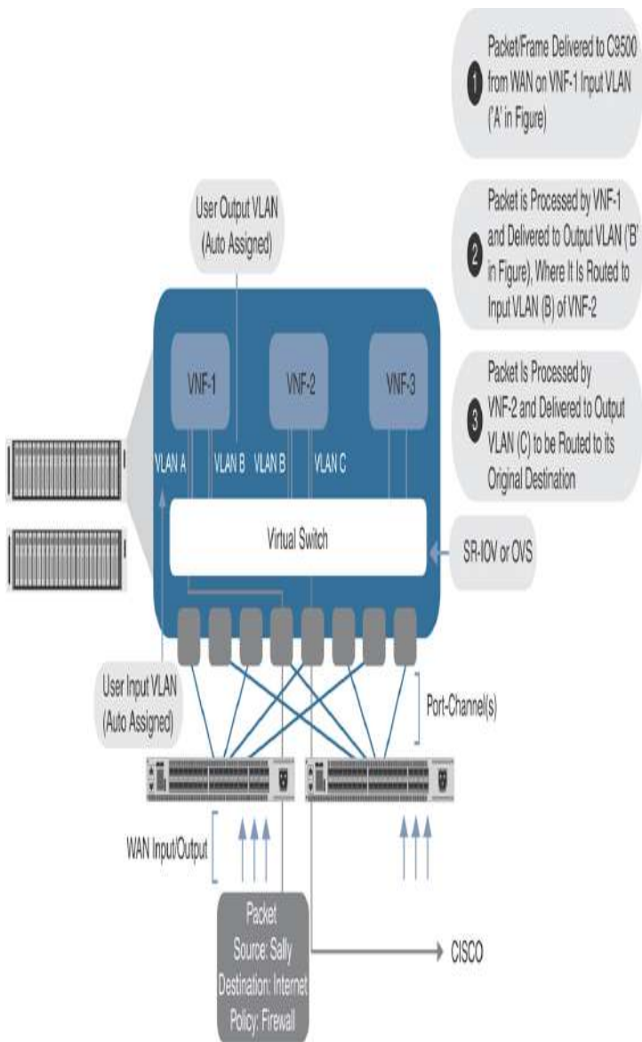
Figure 11-53 Detailed Packet Walkthrough
