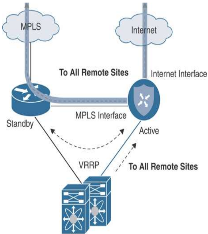
Figure 12-26 Overlay with Underlay Backup—L2 Design Traffic Flow
