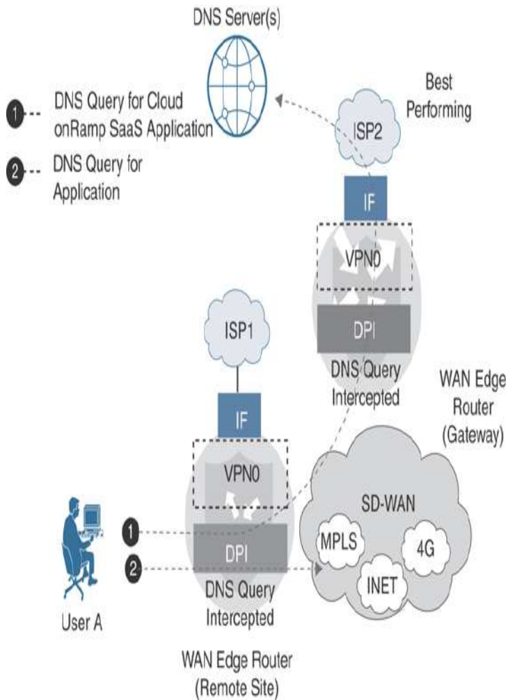
Figure 11-10 Cloud onRamp for SaaS DNS Interception
