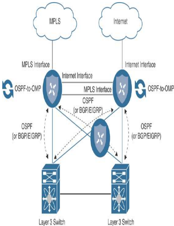
Figure 12-12 Complete CE Replacement—Dual Router L3 Branch
