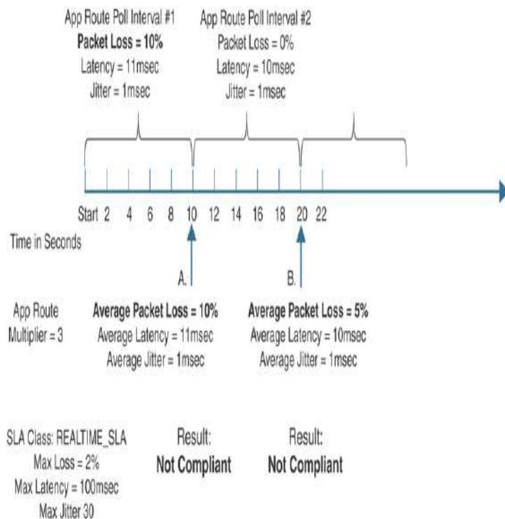
Figure 8-17 SLA Calculations with Two App-Route Poll Intervals
