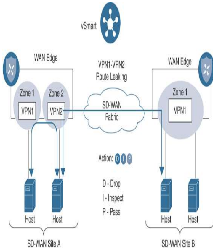
Figure 10-7 Inter-Zone Firewall Application
