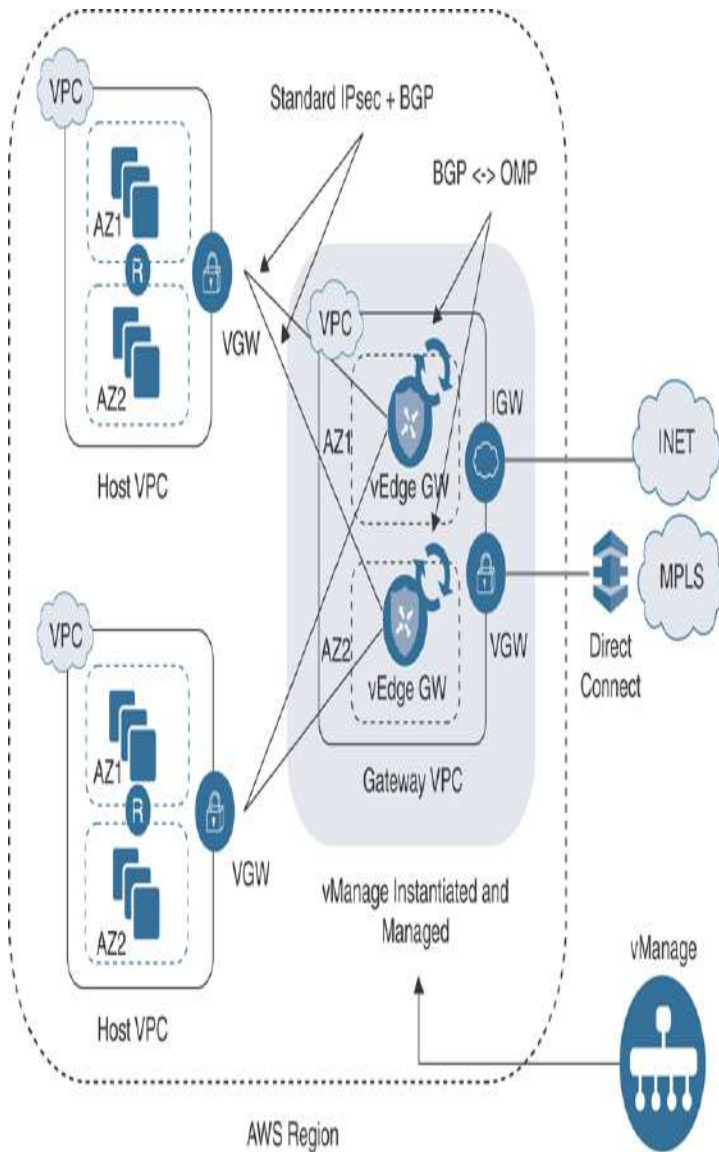
Figure 11-28 Cloud onRamp for IaaS Design
