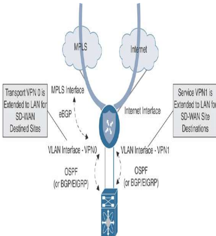
Figure 12-36 Full Overlay with Underlay Routing Without CE Integration
