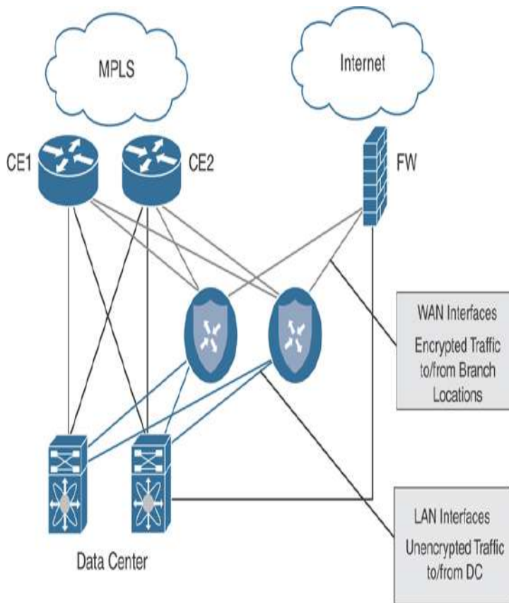
Figure 12-1 Data Center Dedicated Pod
