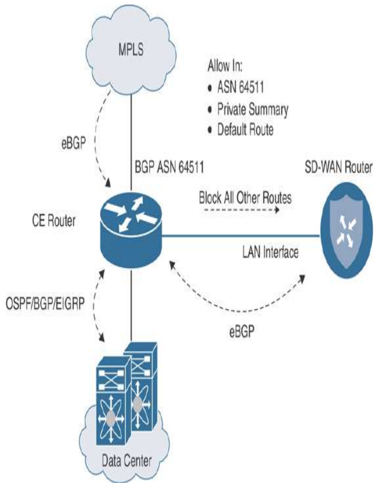
Figure 12-29 Overlay with Underlayer Backup—Data Center Considerations
