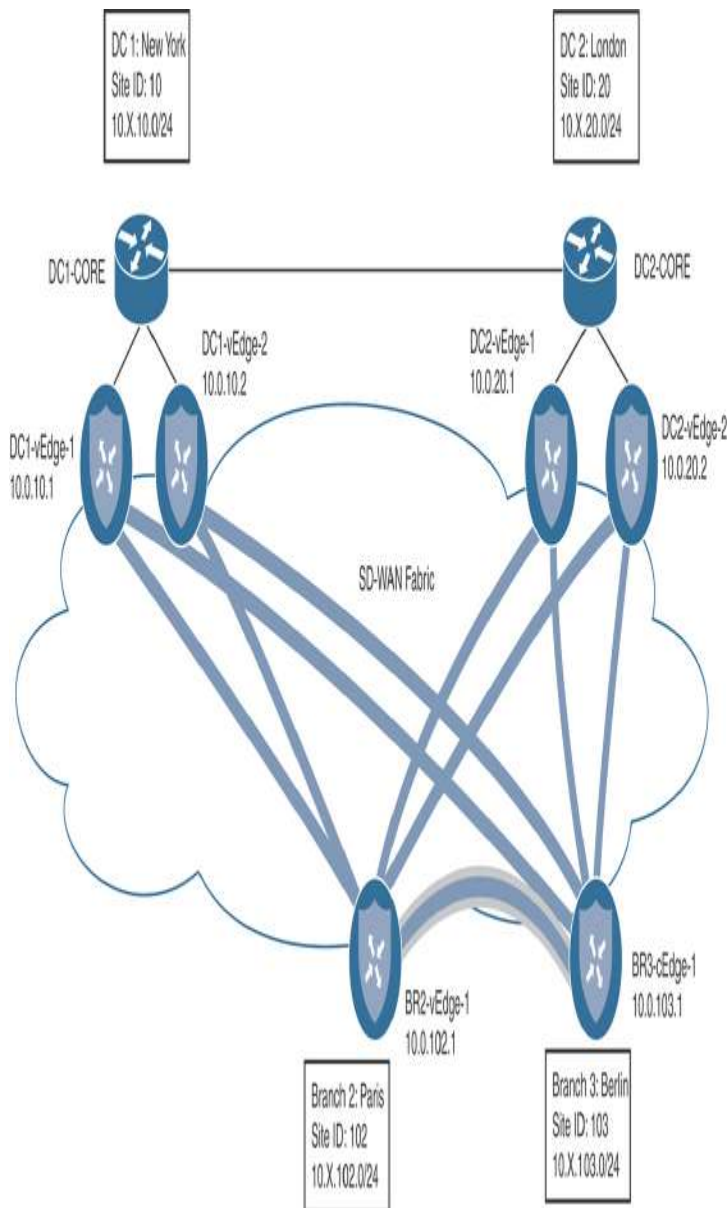
Figure 6-56 Network Topology with Regional Meshes
