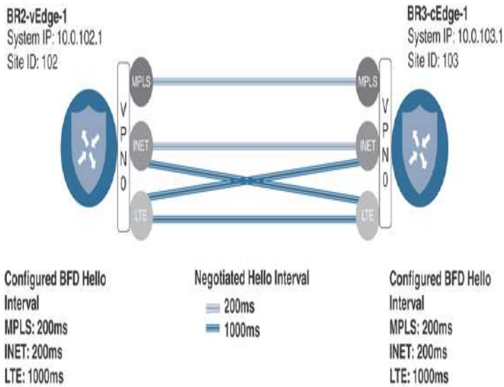
Figure 8-13 BFD Hello Interval Negotiation
