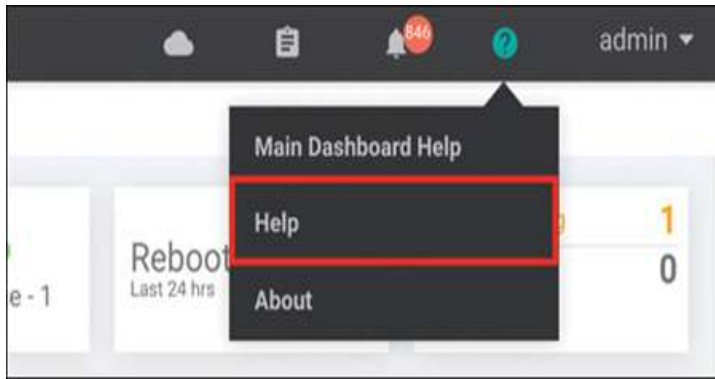
Figure 11-57 vManage Help
