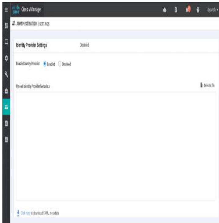
Figure 10-47 SSO Configuration
