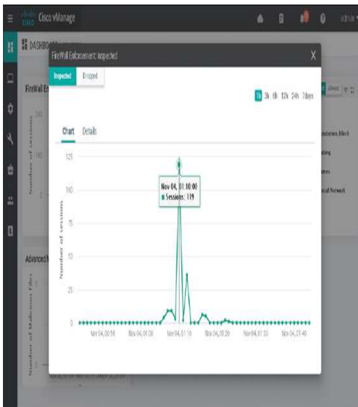
Figure 10-13 Security Dashboard
