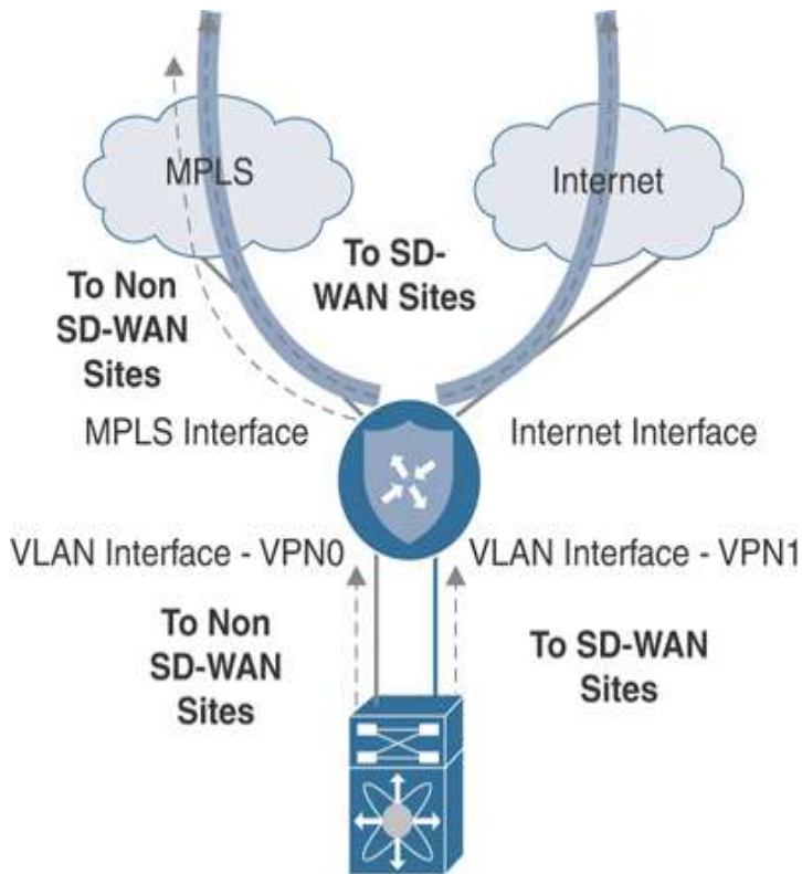
Figure 12-37 Full Overlay with Underlay Routing Without CE Integration Traffic Flow
