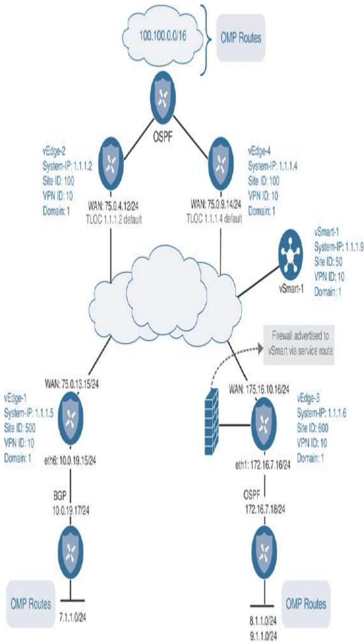
Figure 3-5 Examples of the Three Types of OMP Routes
