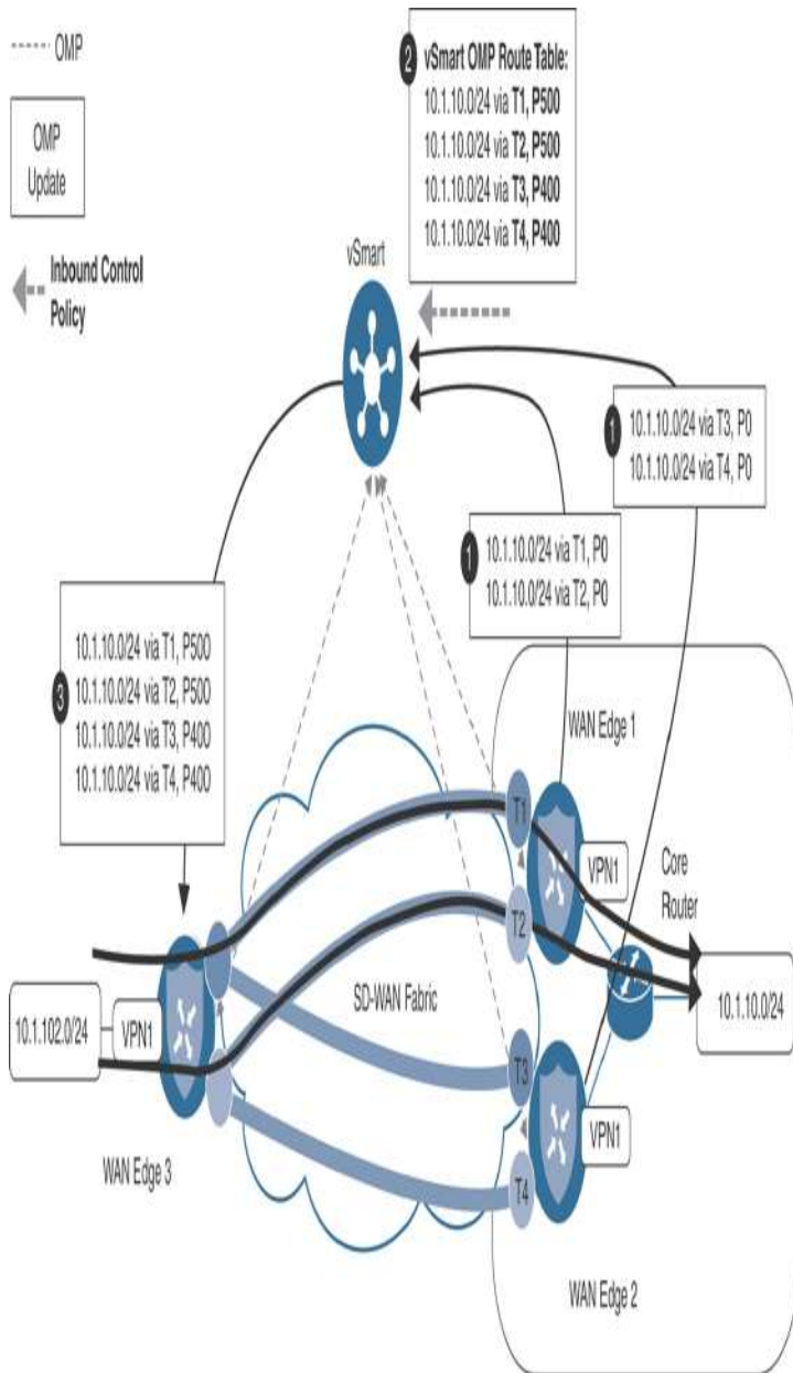
Figure 6-48 Illustration of the Effects of Different Preference Values on the Forwarding Plane
