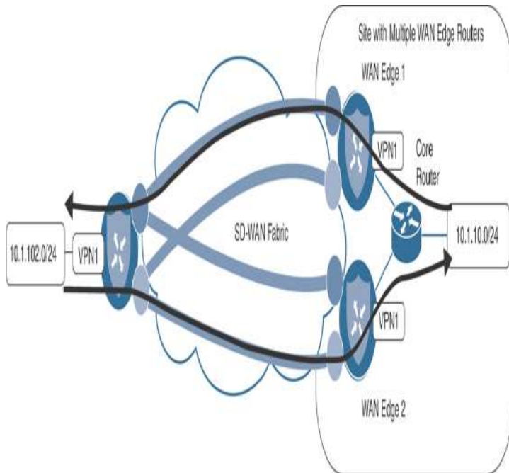
Figure 6-43 Multipathing on the Fabric May Use Multiple WAN Edge Routers for a Single Flow
