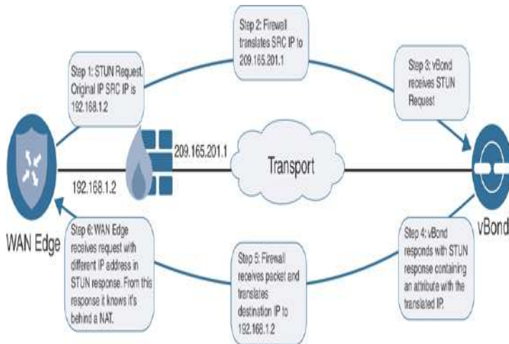
Figure 3-23 NAT Traversal with STUN
