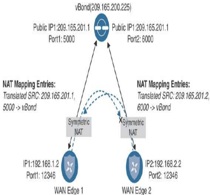
Figure 3-24 Symmetric NAT Restrictions
