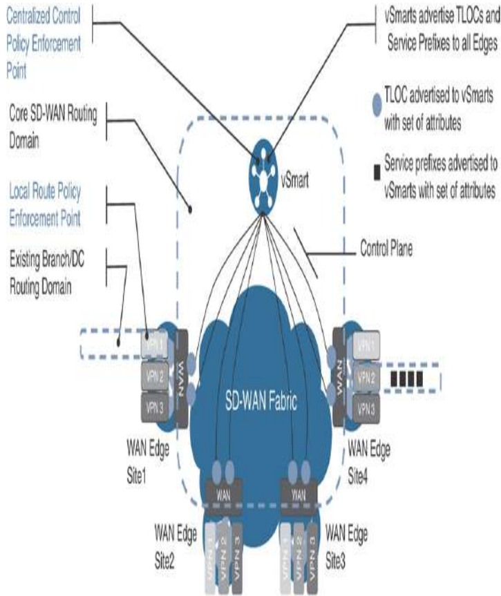
Figure 5-4 Manipulating the Control Plane with Centralized and Localized Control Policies
