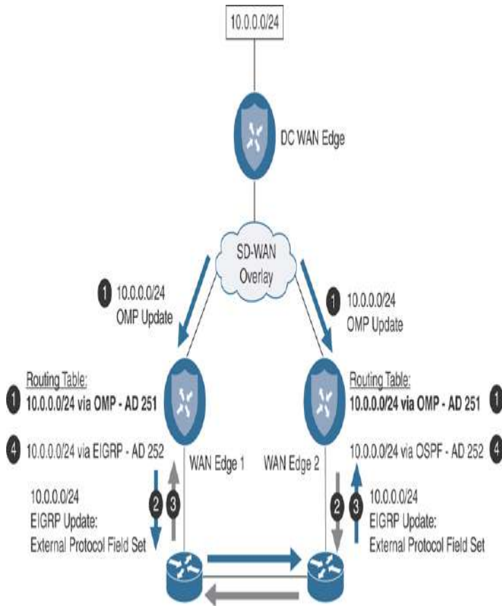
Figure 3-13 EIGRP Loop Prevention with External Protocol Field
