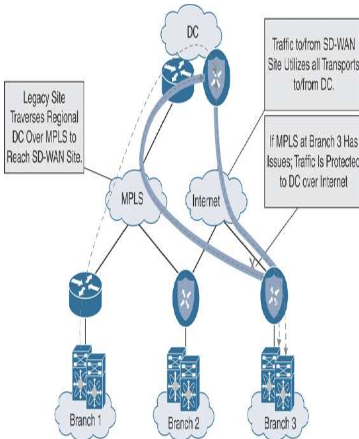
Figure 12-23 SD-WAN to Non-SD-WAN Site Overlay-Only Traffic Flow
