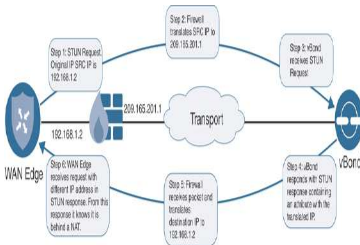
Figure 2-9 STUN NAT Detection Method
