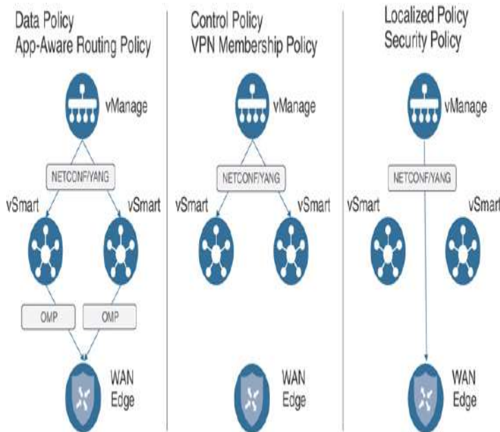
Figure 5-7 Policy Administration, Activation, and Enforcement
