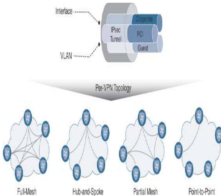
Figure 2-3 Segmentation and Per VPN Topologies
