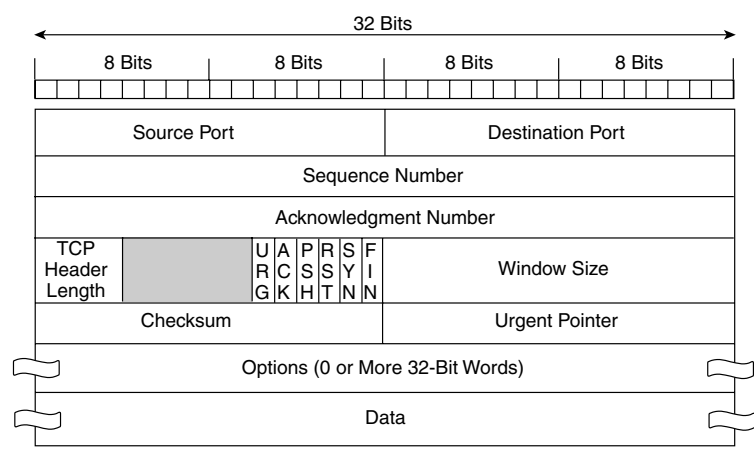
Figure 7-8 TCP Header
