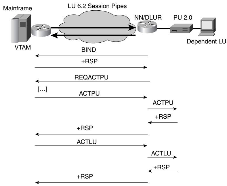
Figure 14-8 DLUR/DLUS
