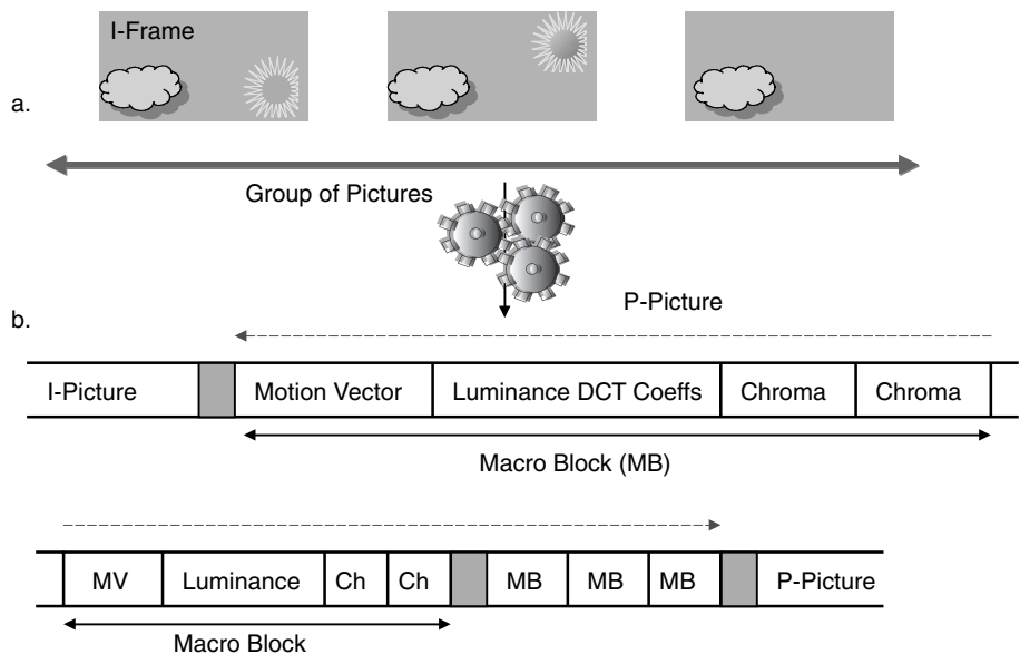
Figure C-3 MPEG Encoding
