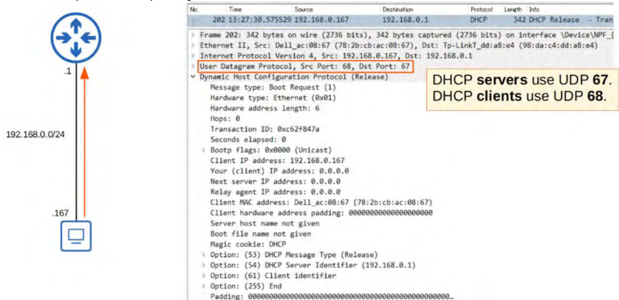
Wireshark capture of the ipconfig /release mechanism
