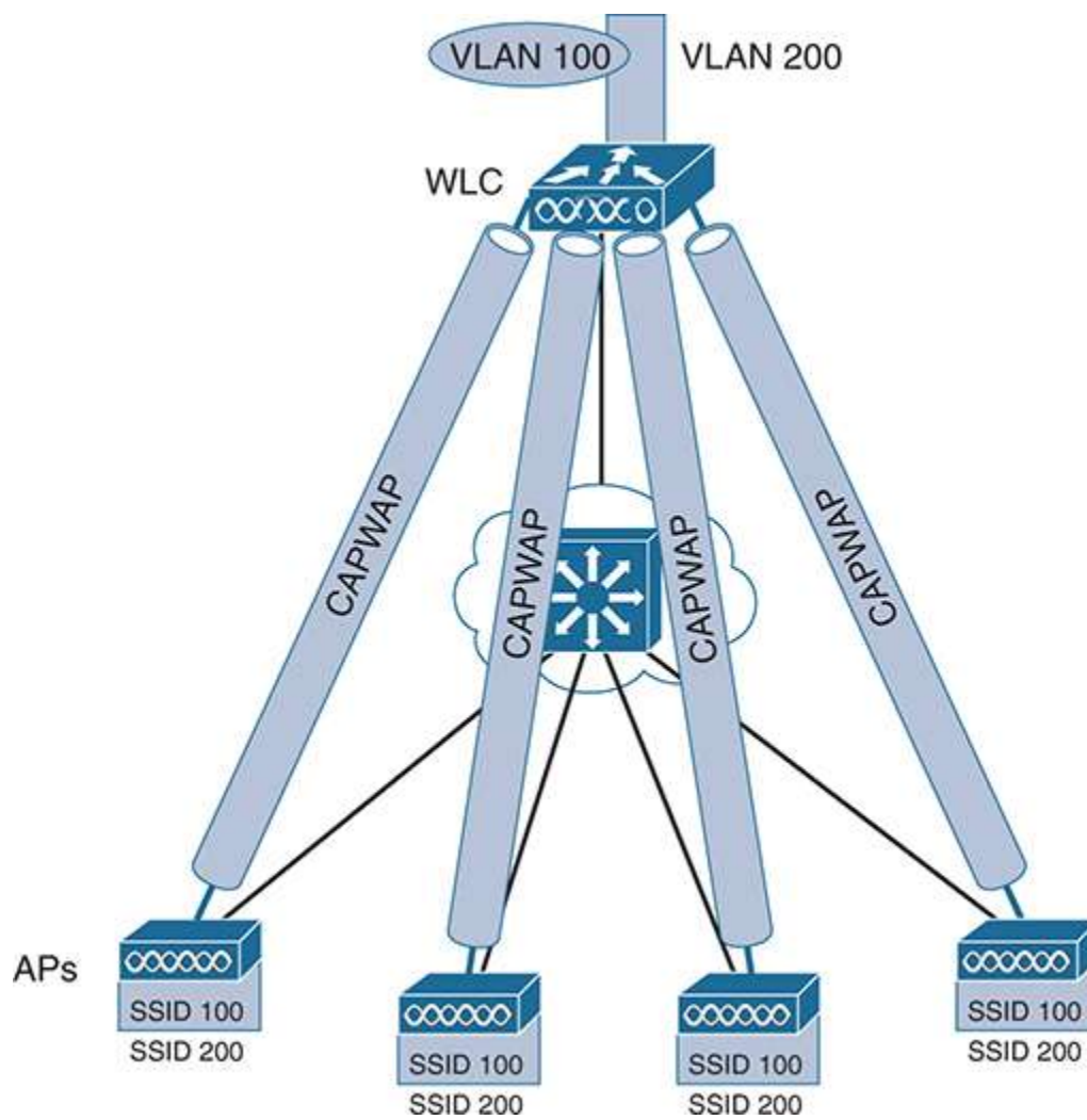
Figure 2-6 Extent of VLAN 100 in a Cisco Wireless Network
