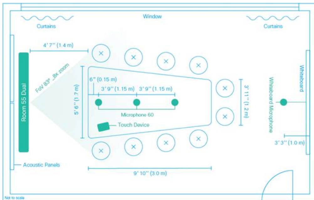
Figure 4-8 Project Workplace Meeting Room Design
