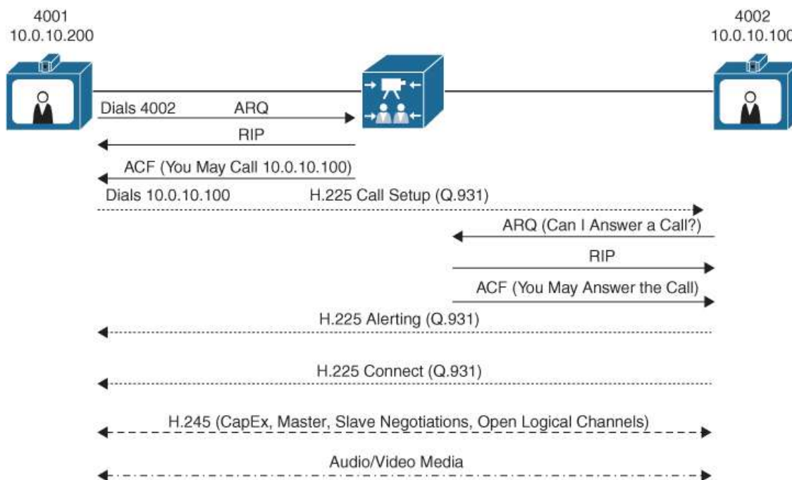
Figure 5-5 H.323 Call Setup Process with a Gatekeeper
