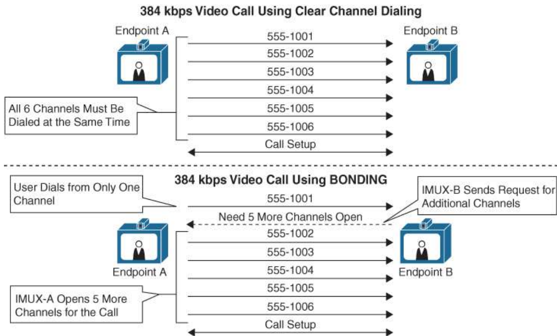
Figure 5-1 Clear Channel Dialing vs. BONDING
