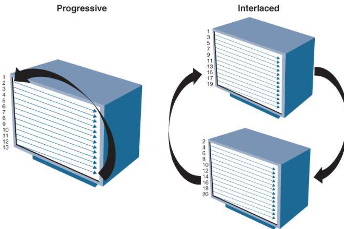
Figure 3-5 Progressive vs. Interlaced Scanning
