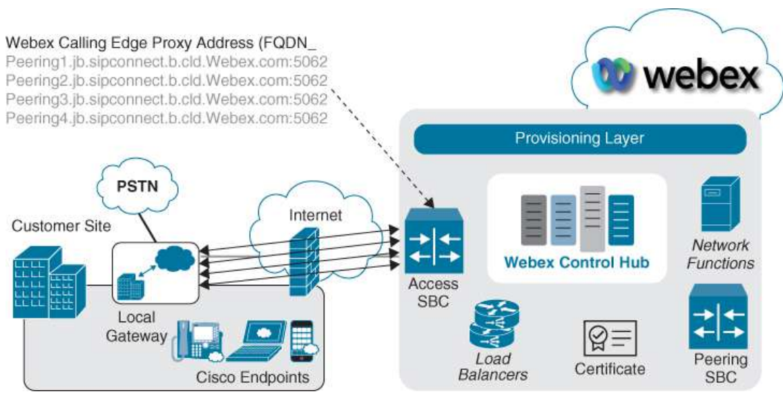
Figure 24-3 Certificate-Based Local Gateway
