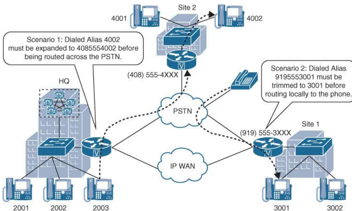
Figure 18-2 Digit Manipulation Scenarios
