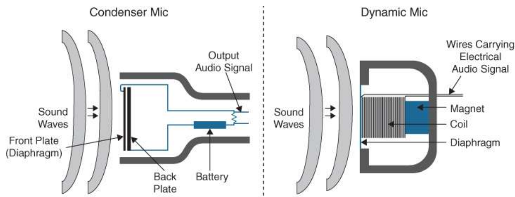
Figure 4-3 Condenser Mic and Dynamic Mic Physical Differences
