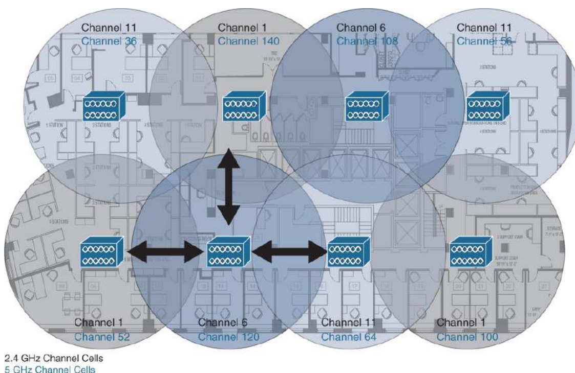
Figure 12-5 High Availability Deployment of WLANs Using Overlapping Channel Cells
