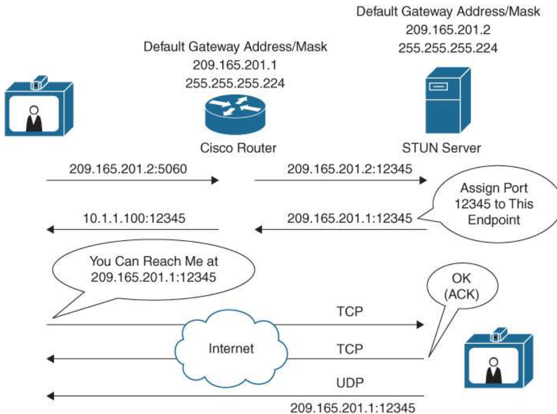
Figure 5-10 STUN Operation Within an Asymmetric Network
