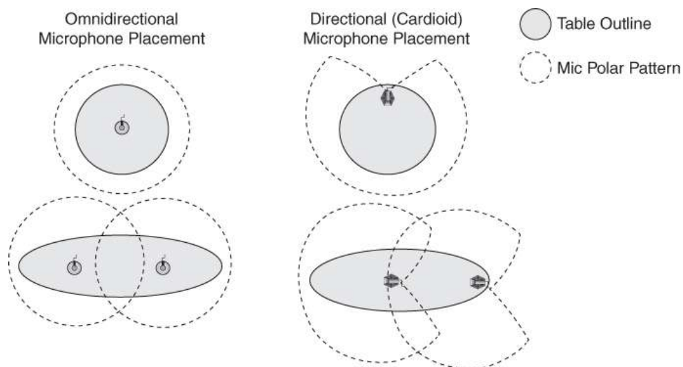
Figure 4-7 Microphone Placement in Meeting Rooms
