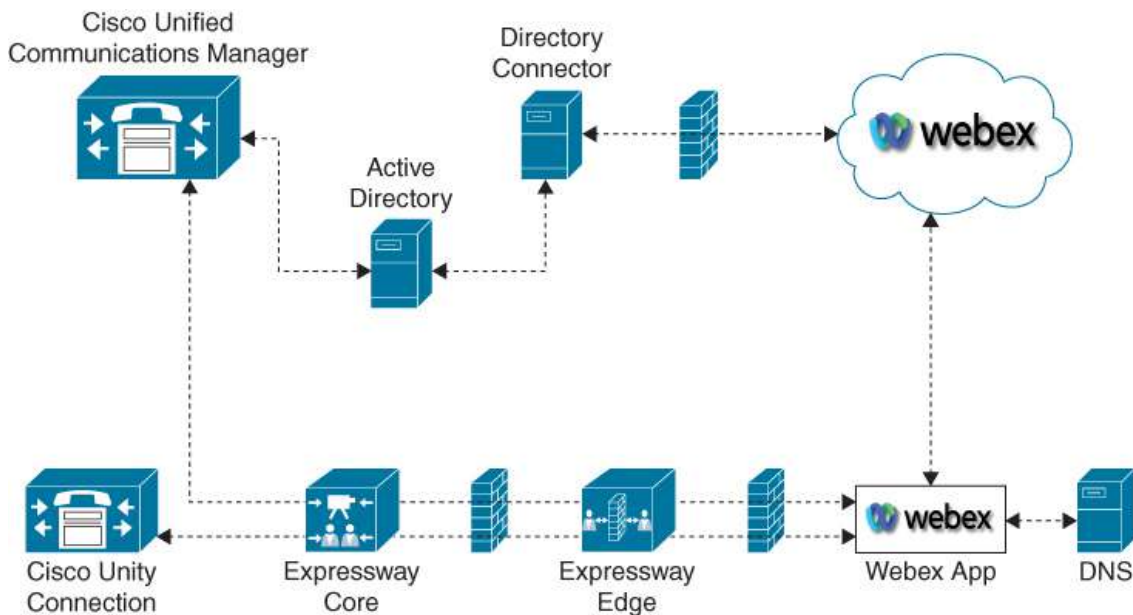
Figure 29-2 Architecture for Deploying Webex App Remotely
