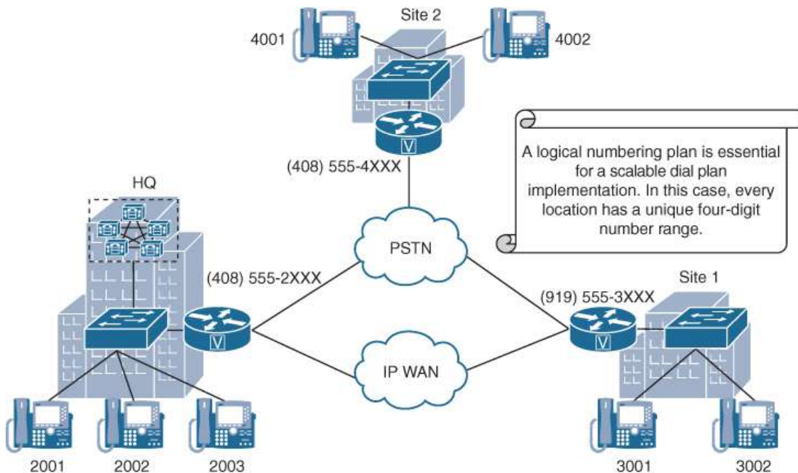
Figure 18-1 Dial Plan Components and Functions
