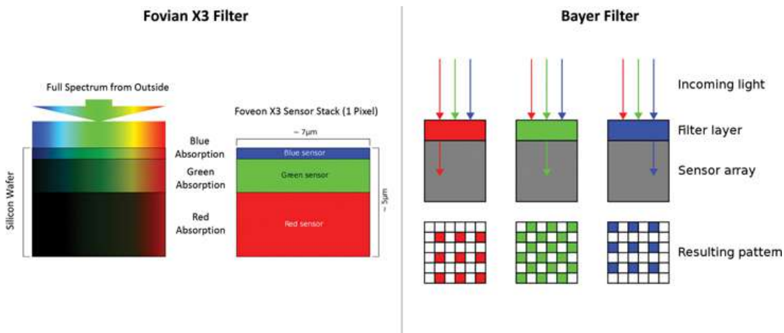
Figure 3-3 Foveon X3 Sensor vs. Bayer Sensor
