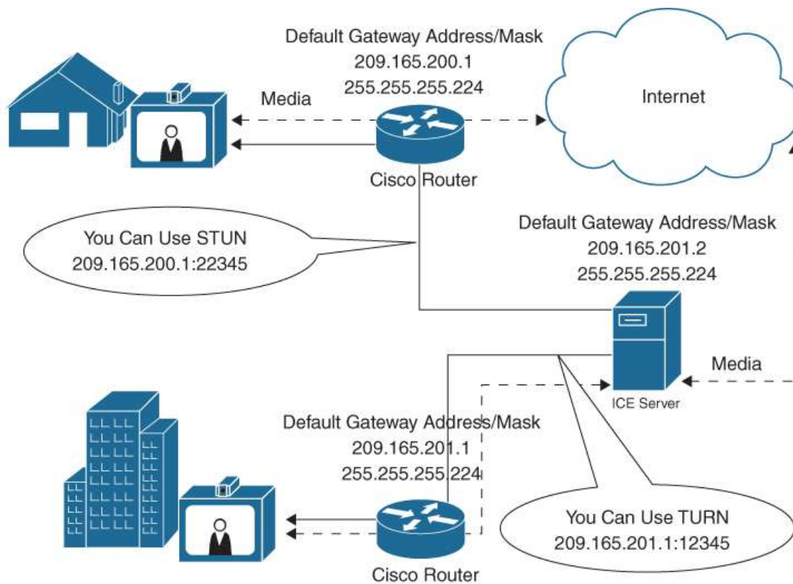
Figure 5-12 ICE Operation Within Asymmetric and Symmetric Networks
