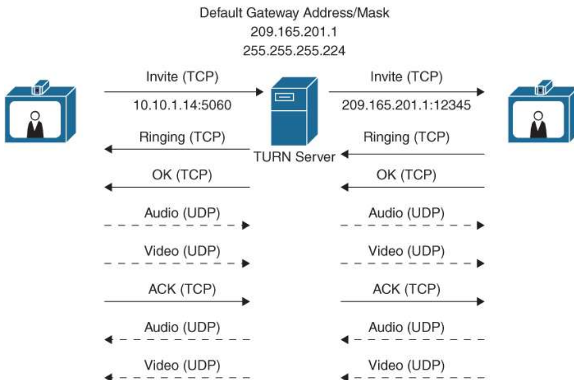
Figure 5-11 TURN Operation Within a Symmetric Network
