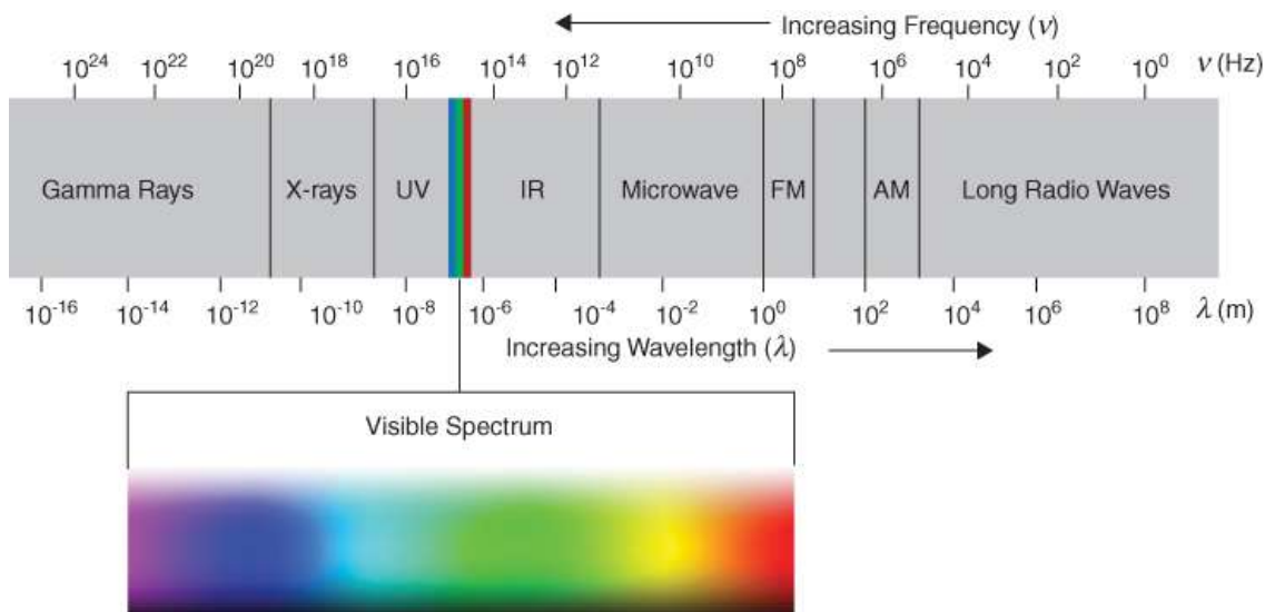
Figure 3-1 Light Spectrums
