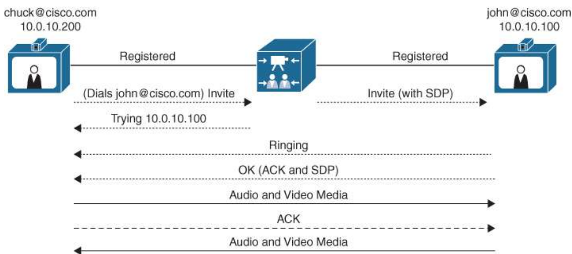
Figure 5-9 SIP Early Offer Call Setup Process
