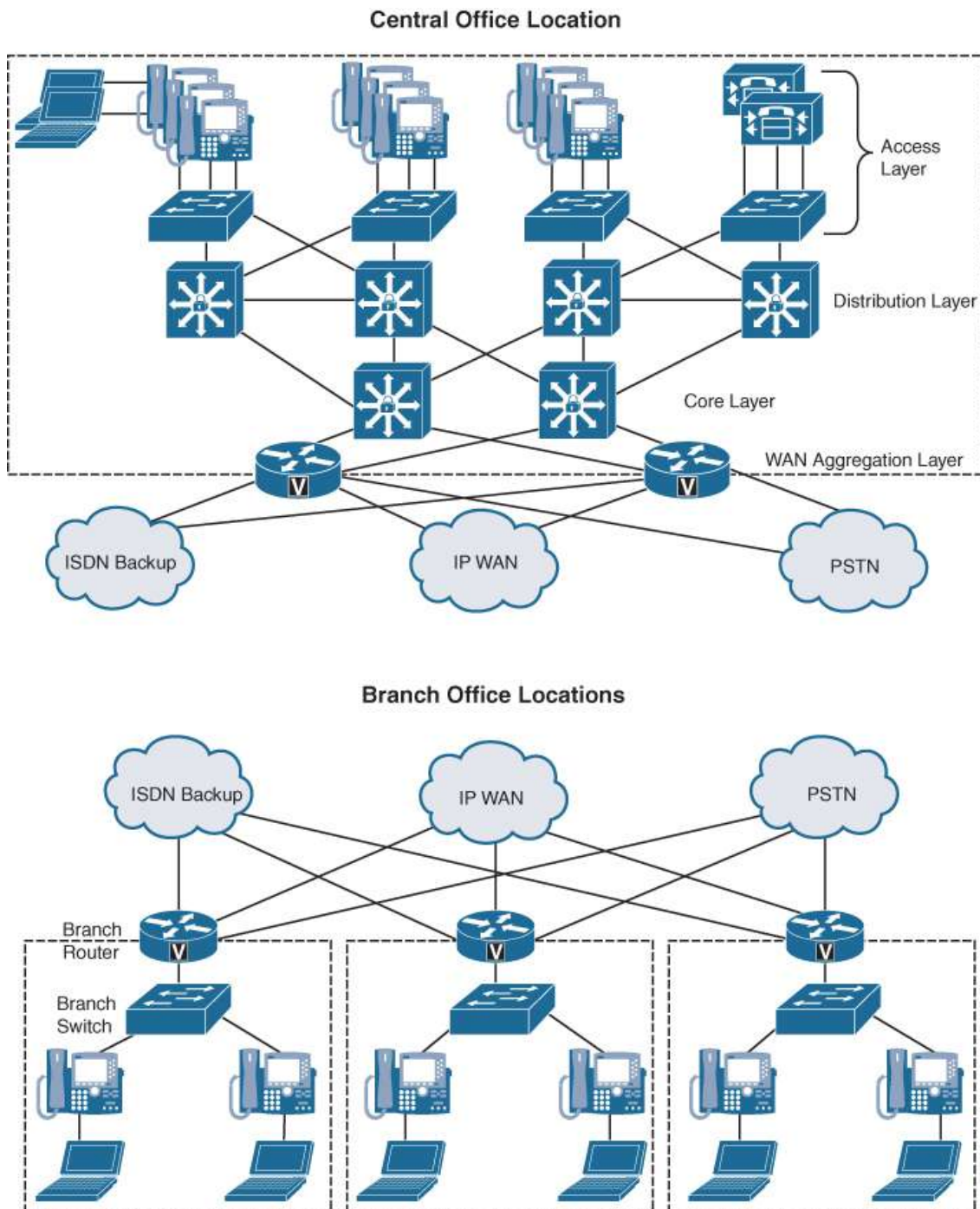
Figure 12-1 Typical Enterprise Network Infrastructure
