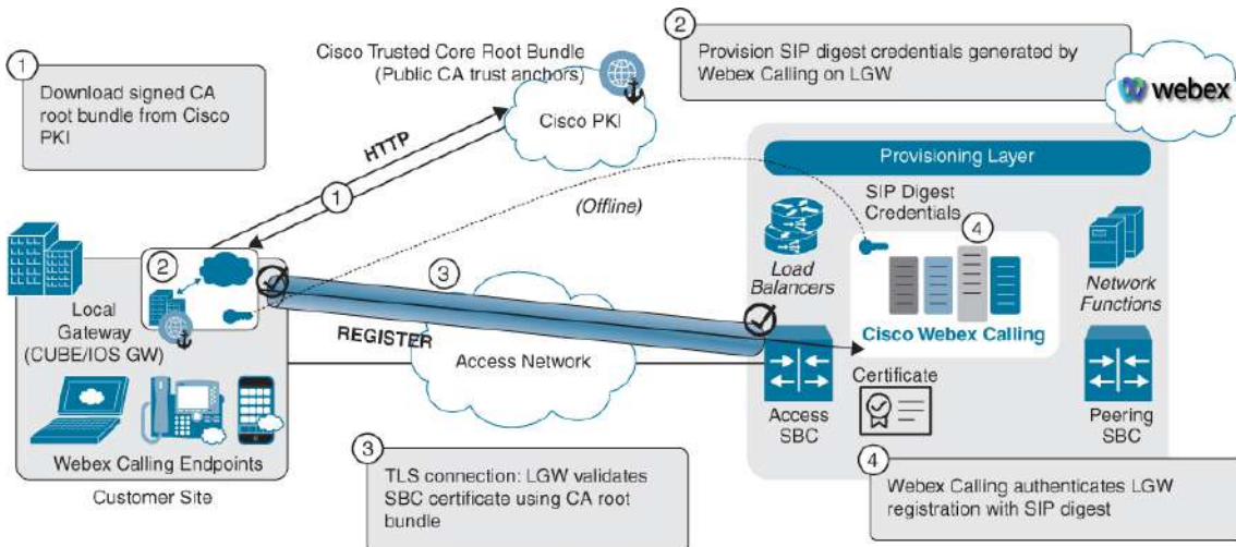
Figure 26-8 Security Handshake and Local Gateway Registration Process
