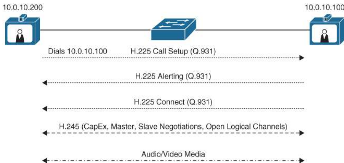
Figure 5-4 H.323 Call Setup Process Without a Gatekeeper
