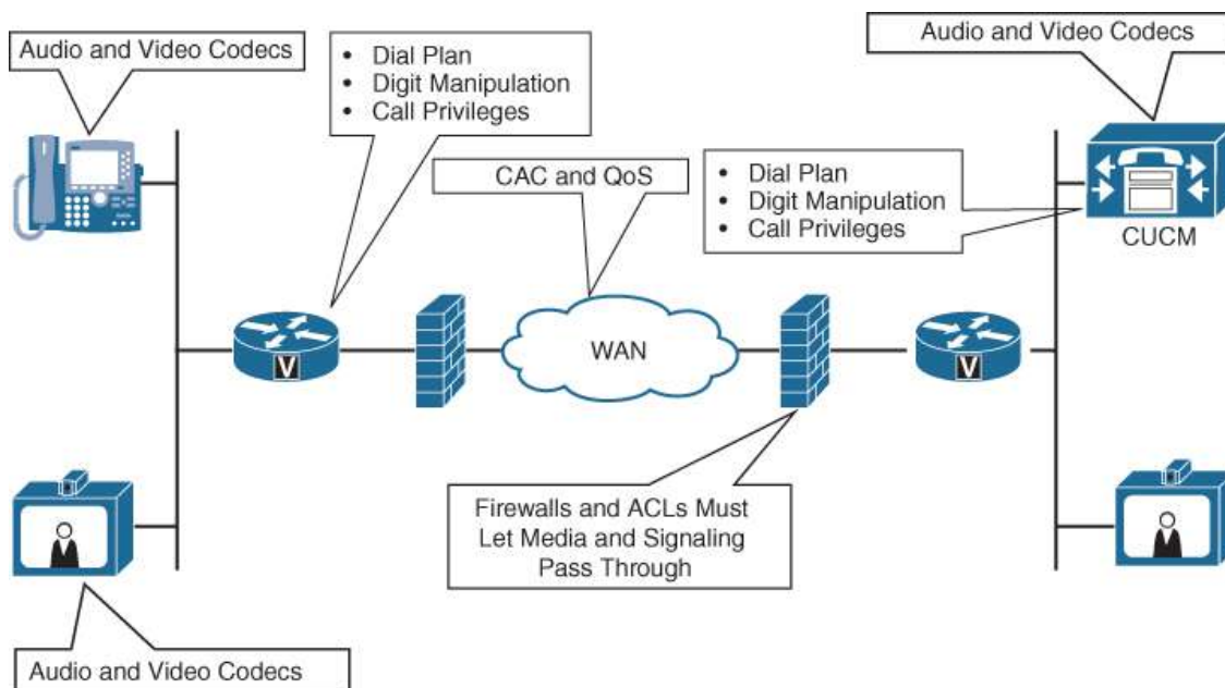
Figure 30-9 Cisco Collaboration Call Setup Components
