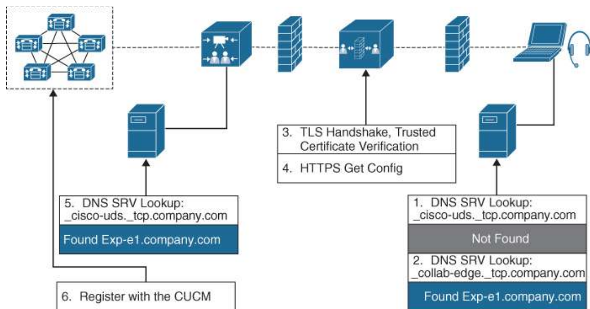
Figure 21-1 Cisco MRA Service Discovery Operation
