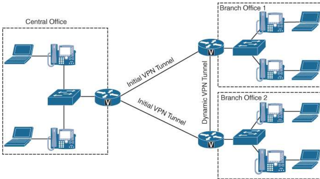
Figure 12-2 DMVPN Network Operations
