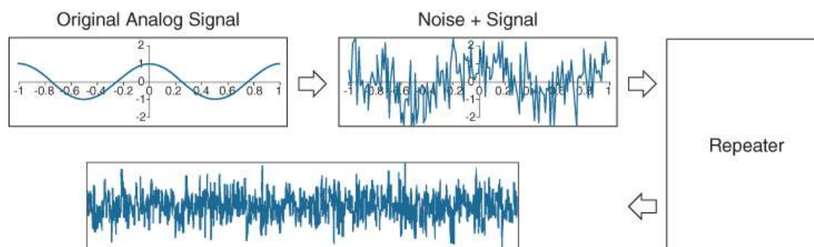
Figure 2-2 Amplification of Noise on an Analog Signal
