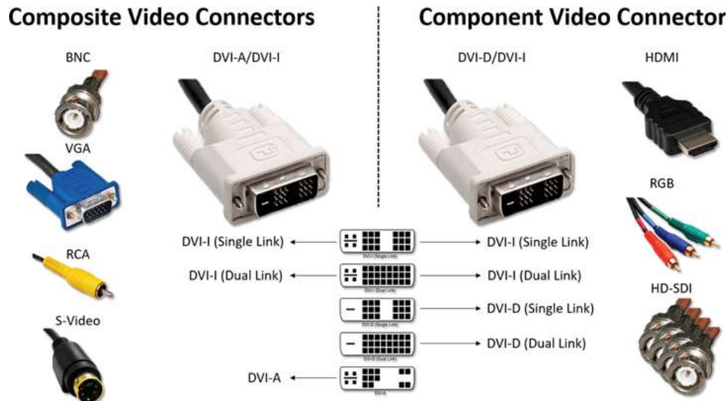
Figure 4-12 Composite and Component Video Connectors
