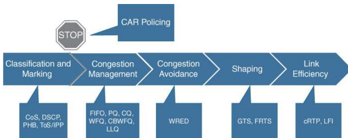
Figure 13-3 QoS Components
