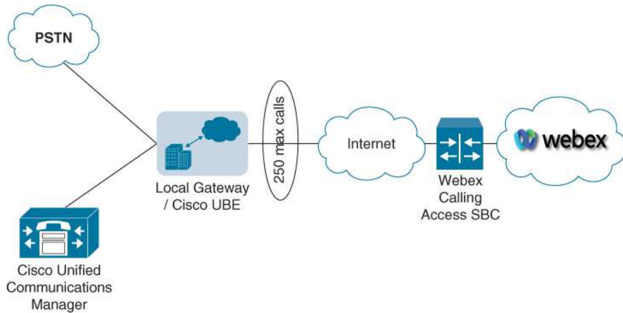
Figure 24-2 Registration-Based Local Gateway
