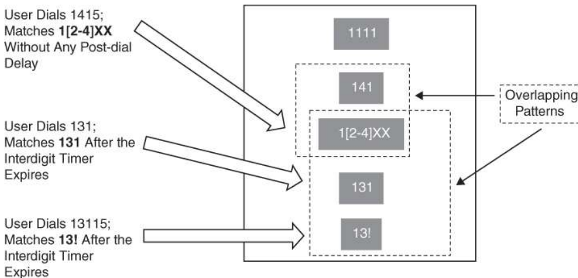
Figure 19-2 Overlaps and Interdigit Timeout
