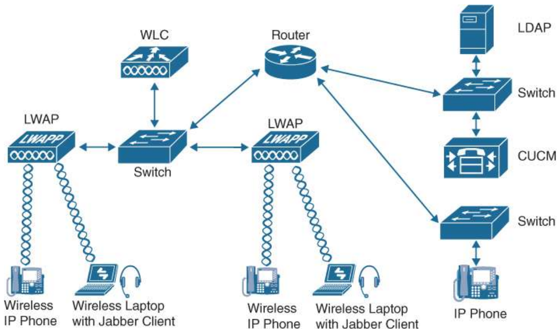
Figure 12-4 Components of a Full WLAN Deployment
