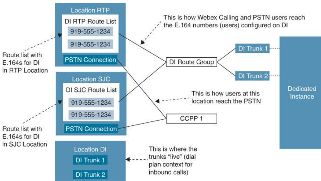
Figure 24-1 Route Lists for Cloud Connected PSTN
