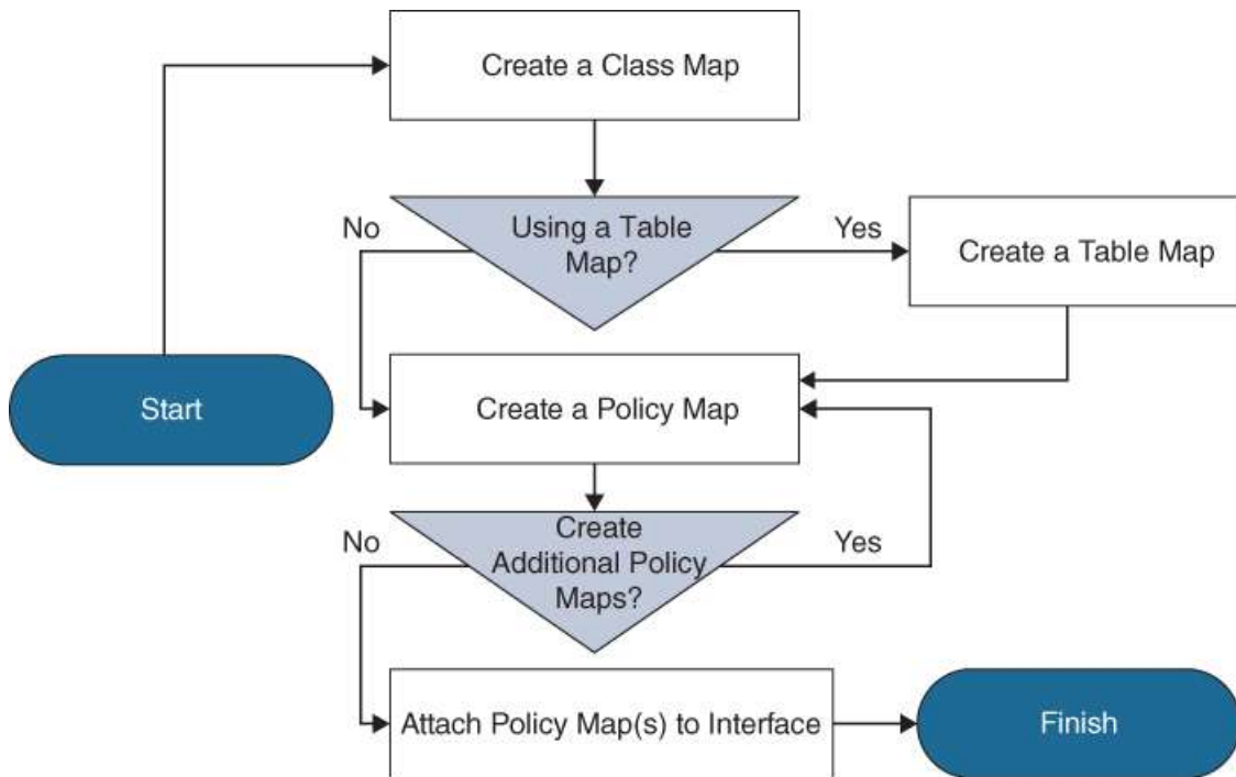
Figure 13-4 QoS Configuration Process
