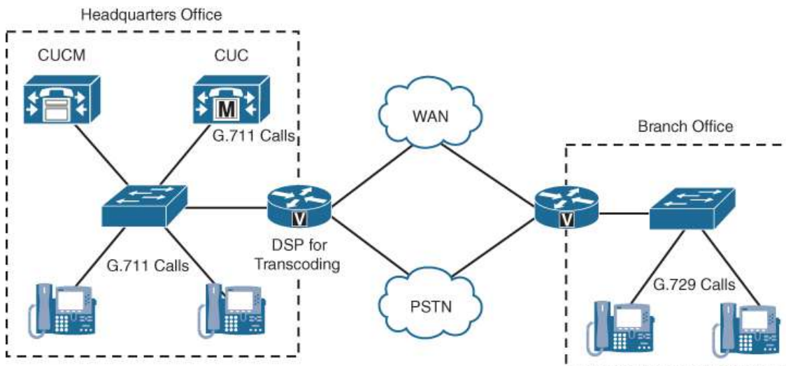
Figure 27-1 Centralized Deployment of CUC
