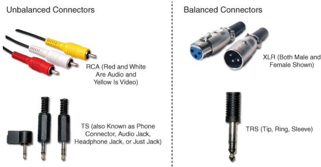
Figure 4-5 Balanced and Unbalanced Connectors
