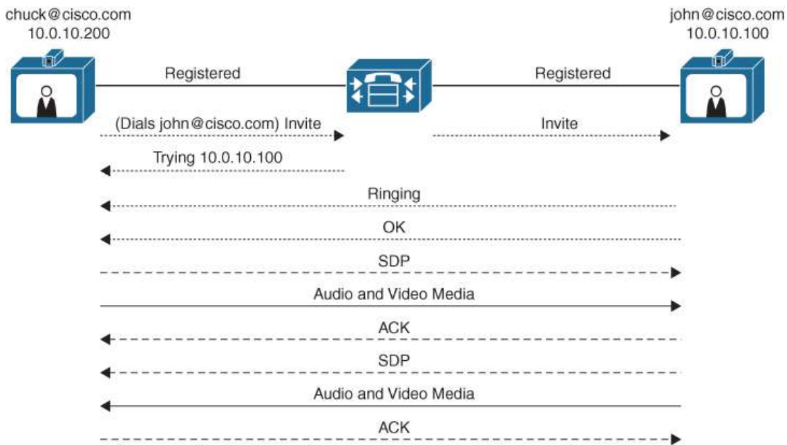
Figure 5-8 SIP Delayed Offer Call Setup Process
