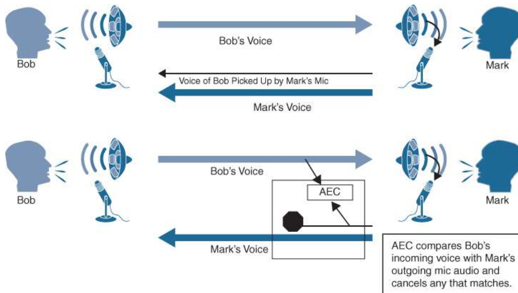
Figure 4-6 Acoustic Echo Cancellation (AEC)
