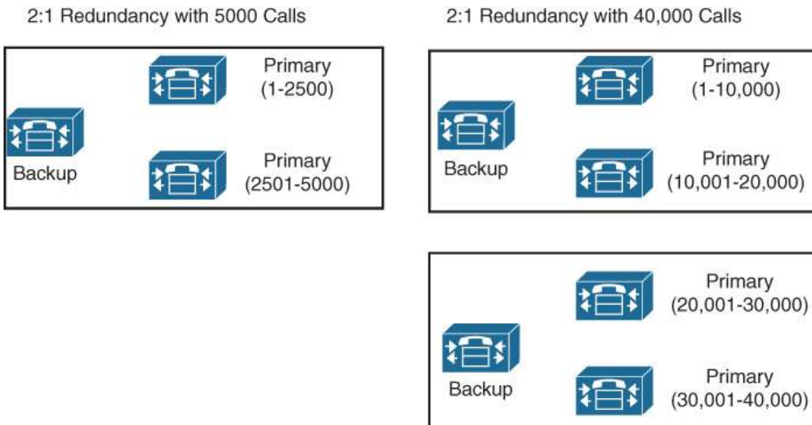
Figure 6-2 Call Processing Subscriber Groups in a 2:1 Deployment
