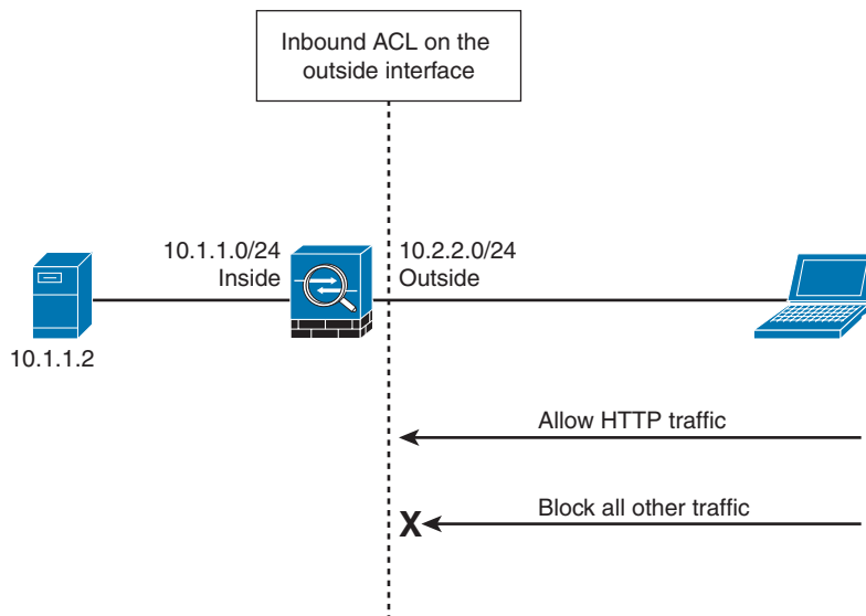
Figure 7-36 Inbound ACL Example
