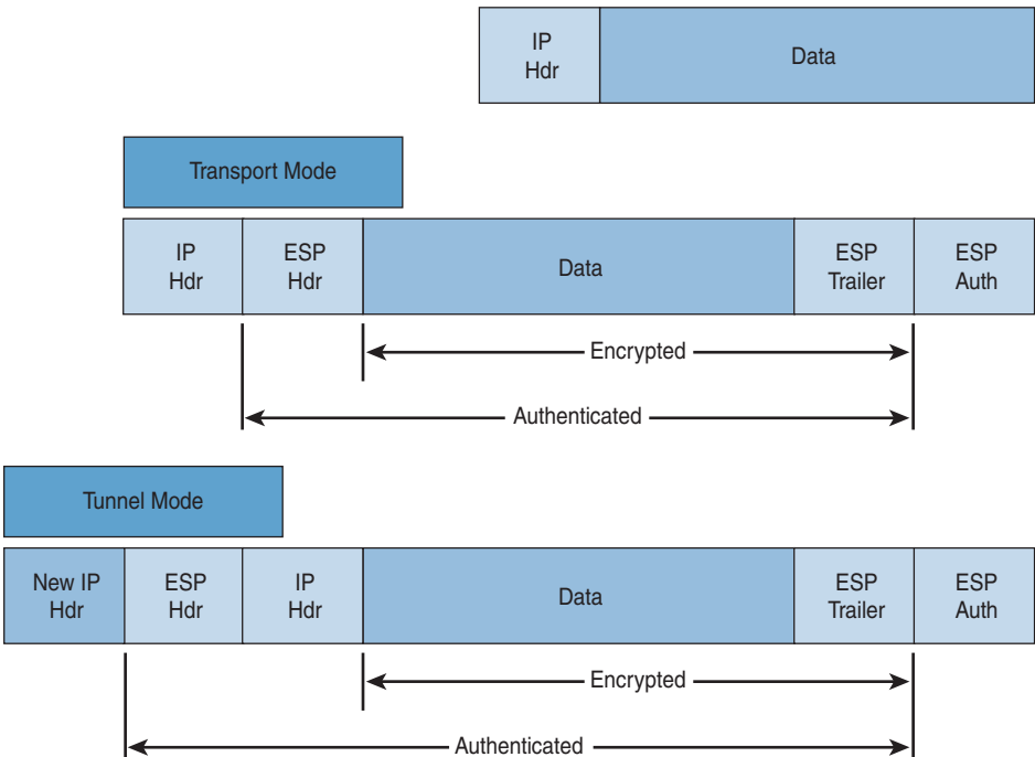
Figure 8-6 IPsec Transport Mode Versus Tunnel Mode
