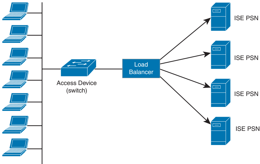
Figure 4-48 Cisco ISE PSNs Behind a Load Balancer
