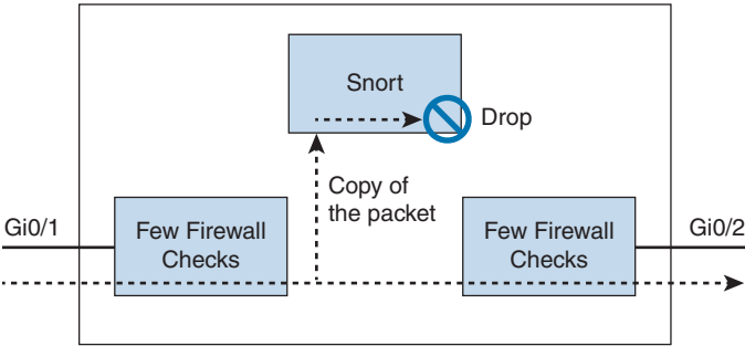
Figure 7-29 Example of Inline Pair with Tap
