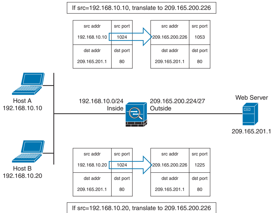
Figure 7-41 PAT Example
