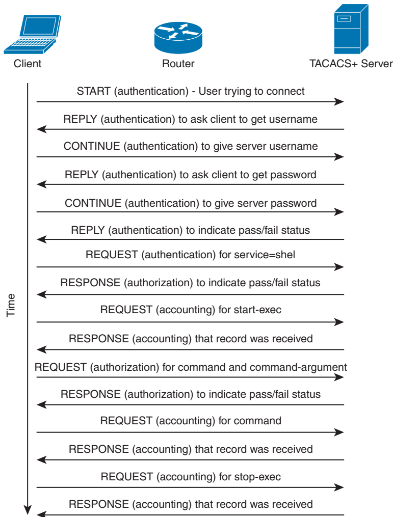
Figure 4-15 TACACS+ Message Exchange for Authentication, Authorization, and Accounting
