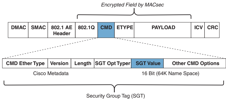
Figure 4-31 SGT Embedded Within a Layer 2 Frame
