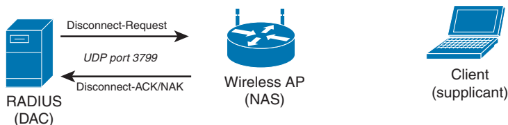
Figure 4-37 Disconnect-Request Sent from a DAC to a NAS
