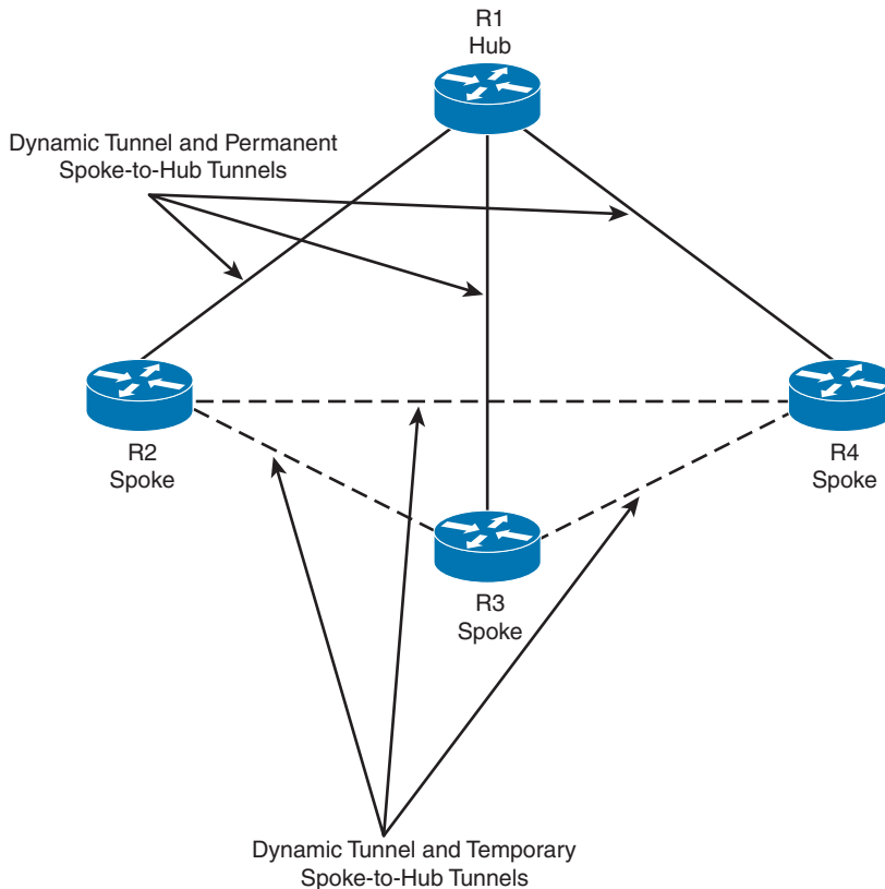
Figure 8-11 DMVPN Example
