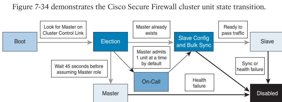
Figure 7-34 Cisco Secure Firewall Cluster Unit State Transition
