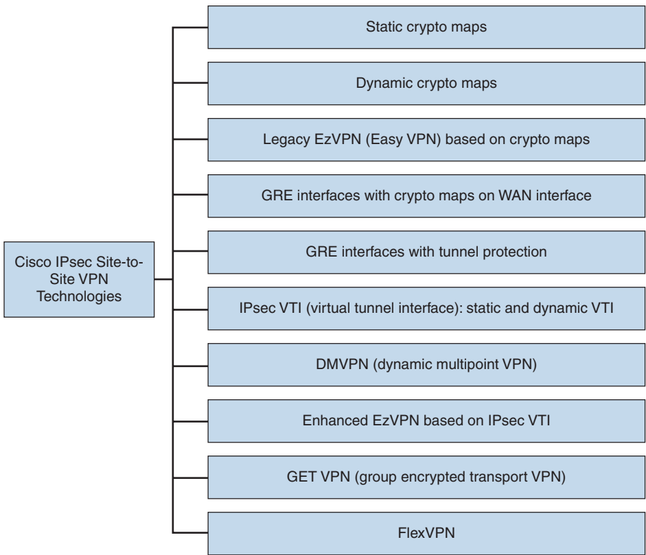
Figure 8-2 Site-to-Site VPN Technologies
