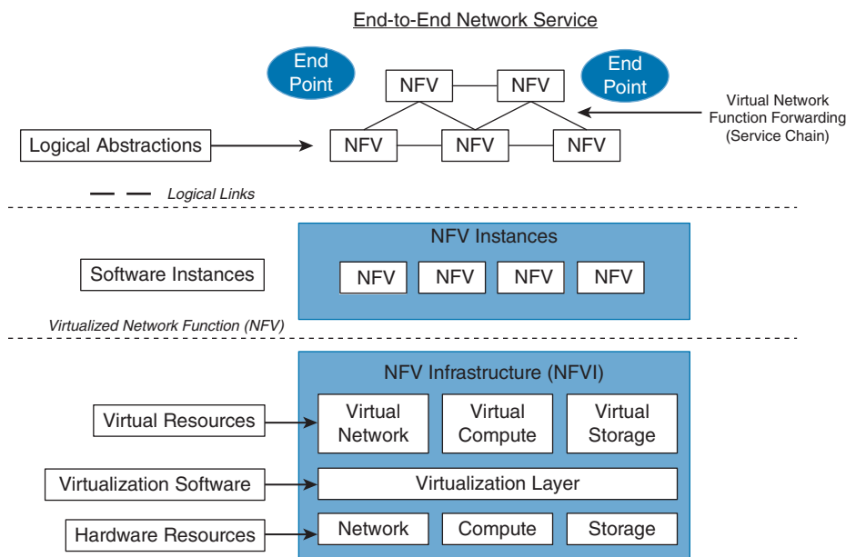
Figure 3-10 NFV Architecture
