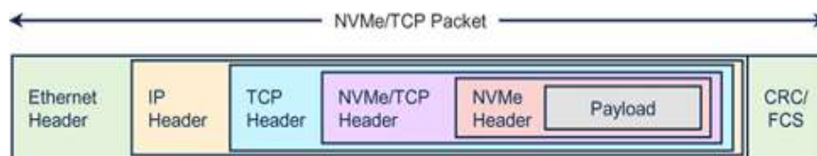
Figure 1-8 NVMe/TCP Packet Format
