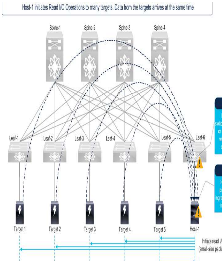
Figure 8-4 Congestion in TCP Storage Networks
