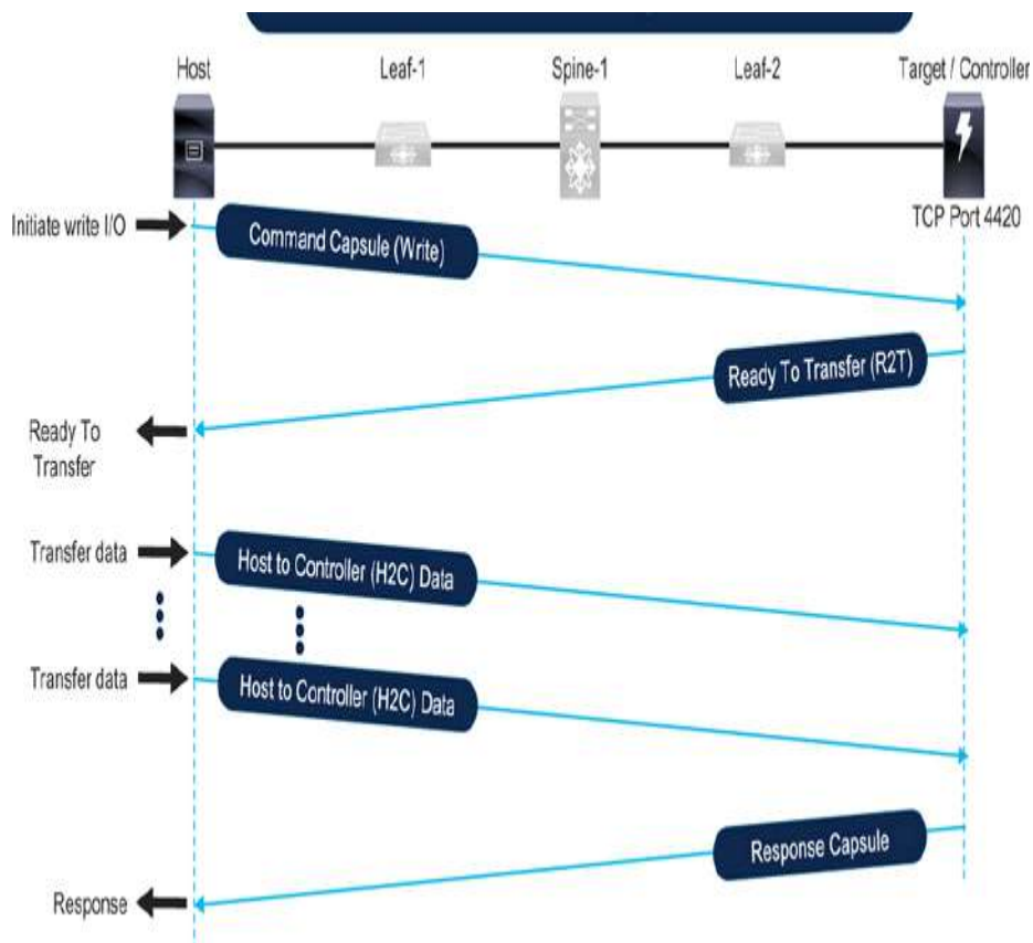
Figure 8-8 NVMe/TCP Write I/O Operation
