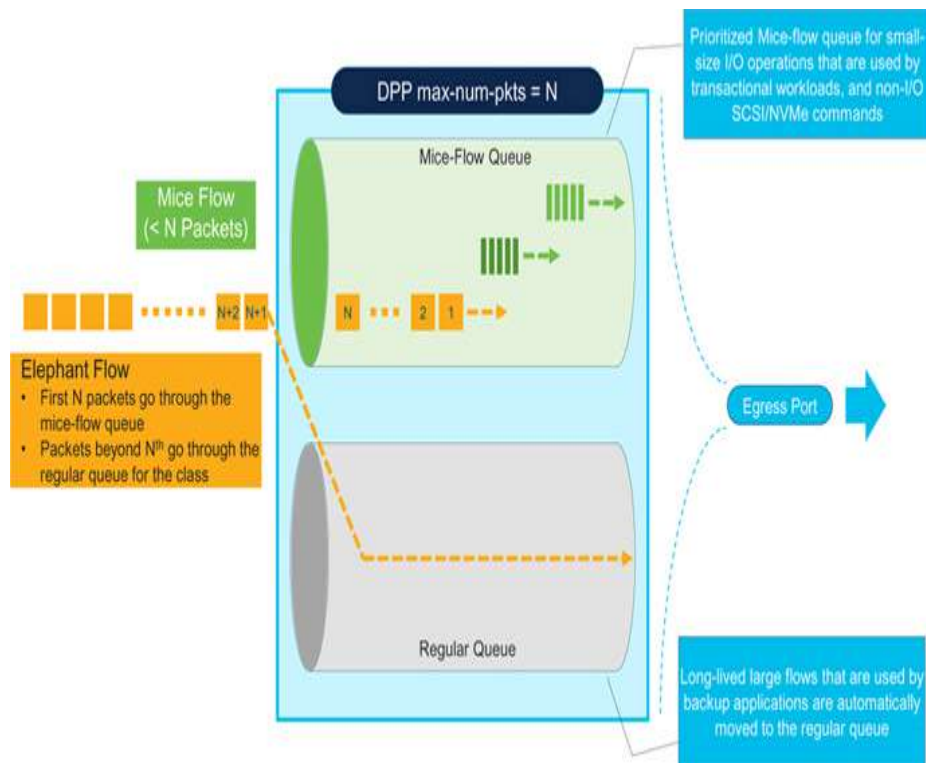
Figure 8-15 DPP mechanism
