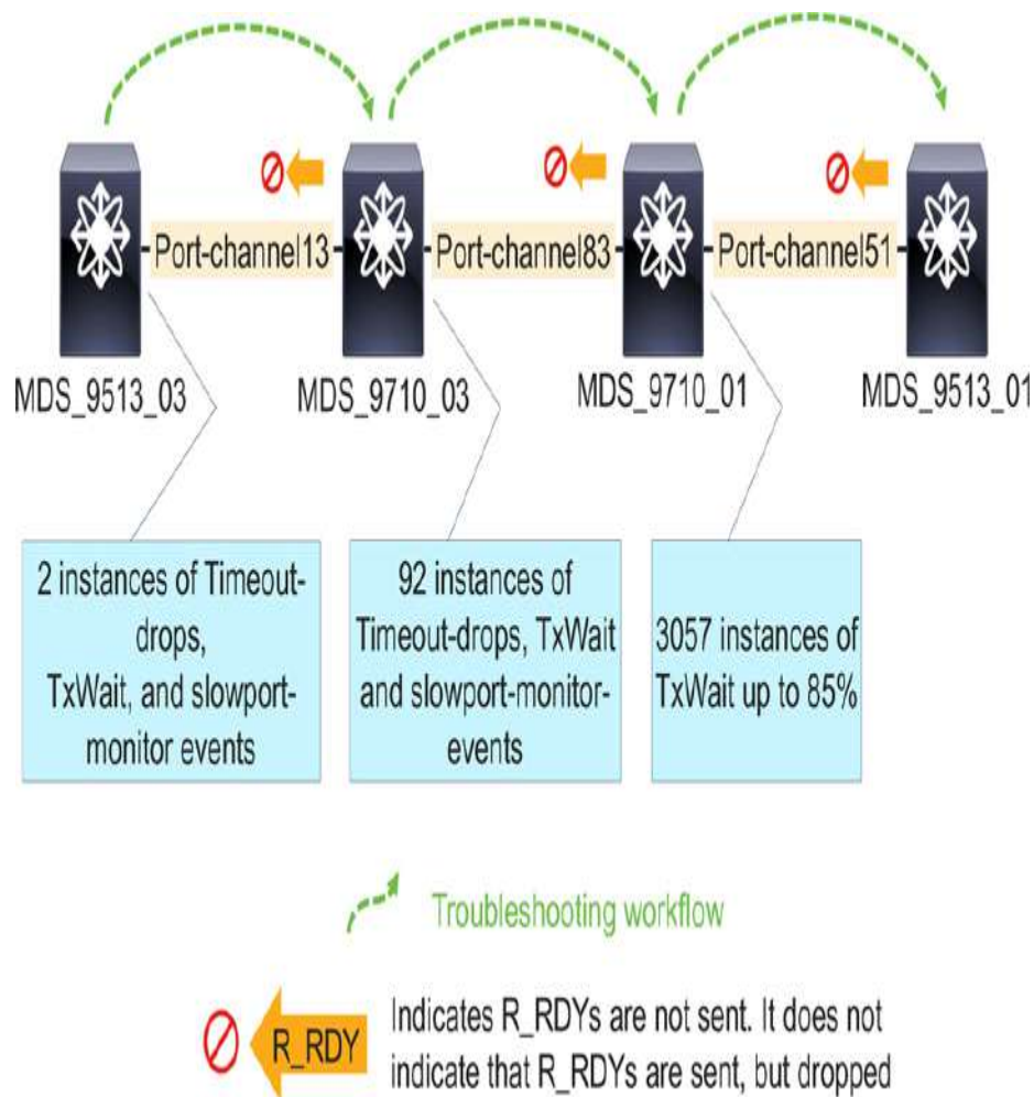
Figure 4-35 Congestion troubleshooting methodology and workflow
