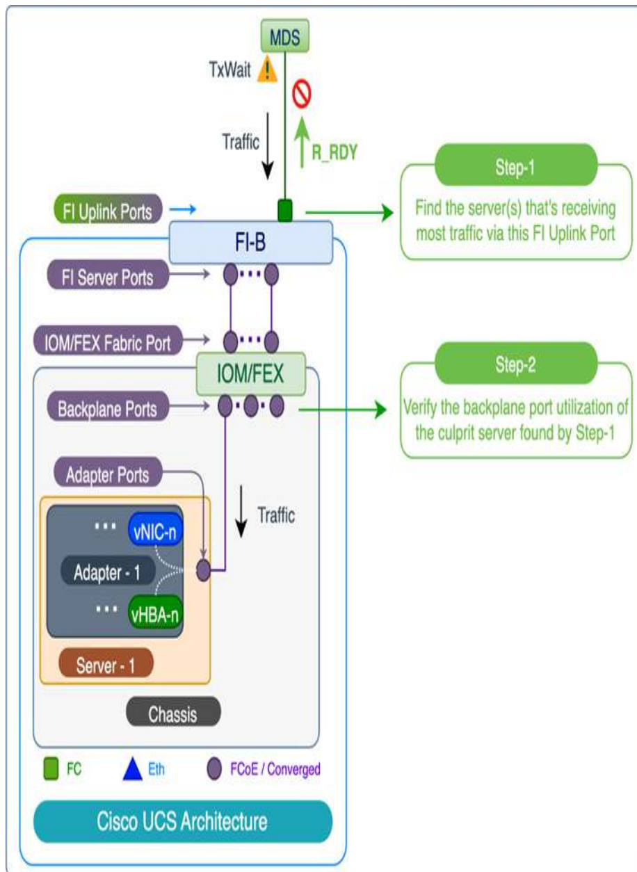
Figure 9-9 Simplified troubleshooting workflow using UTM
