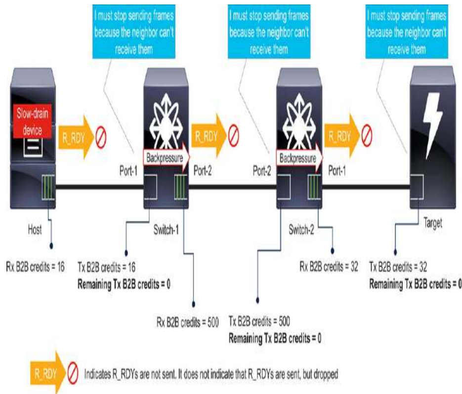
Figure 2-9 Multi-hop lossless fabric using B2B flow control
