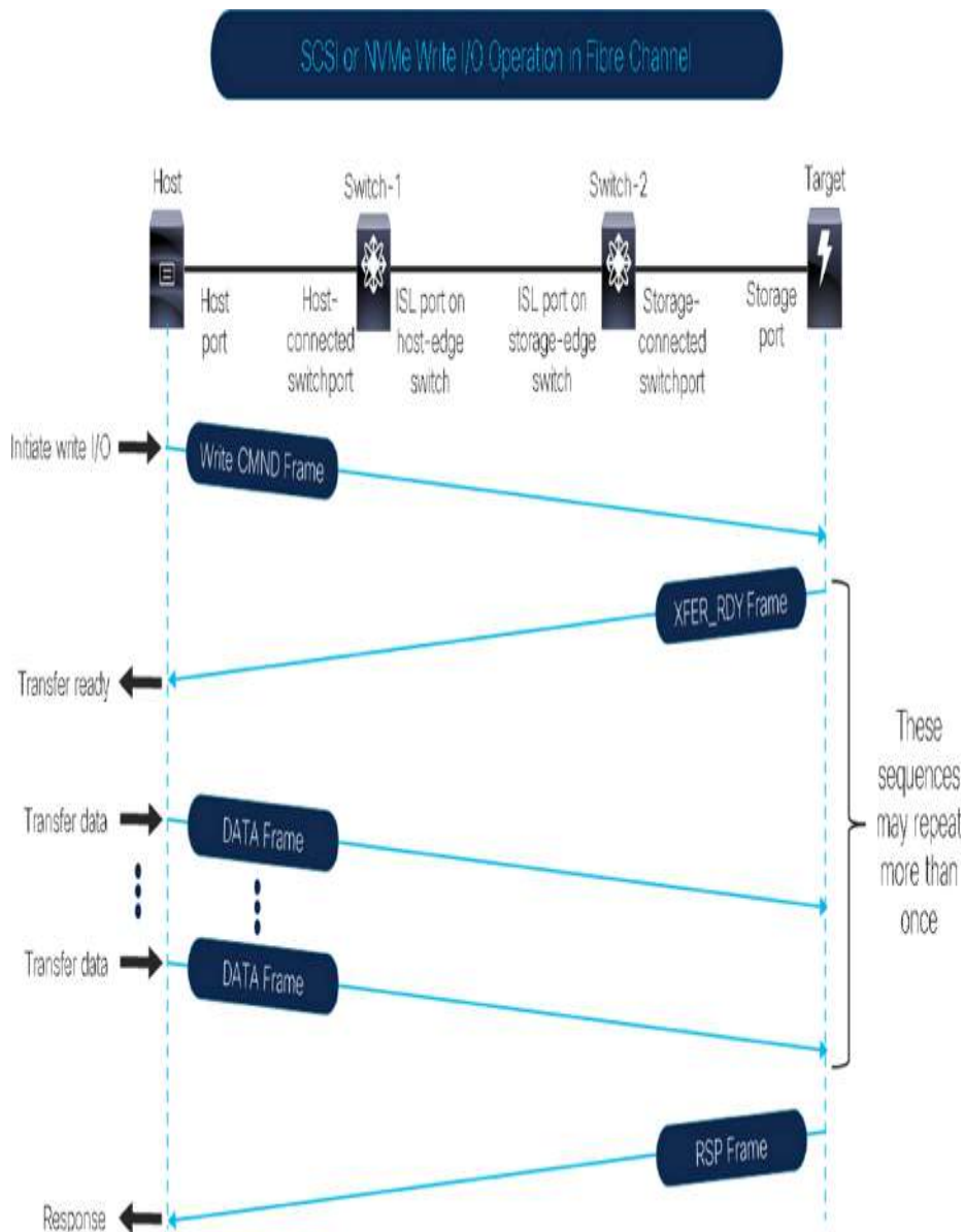
Figure 5-9 SCSI or NVMe Write I/O Operation in a Fibre Channel Fabric
