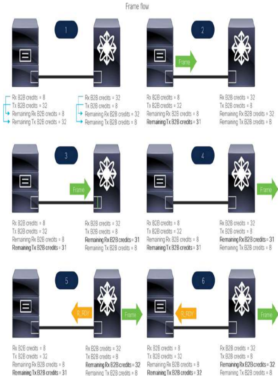
Figure 2-3 Return of B2B credits during frame flow
