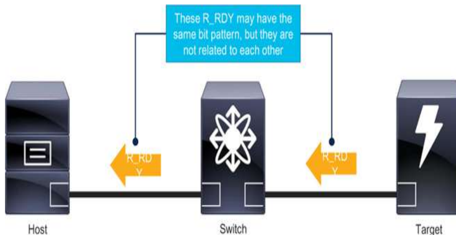
Figure 2-4 R_RDYs remain local to a link
