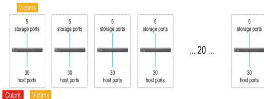
Figure 6-43 Smaller fabrics for reducing the spread of congestion
