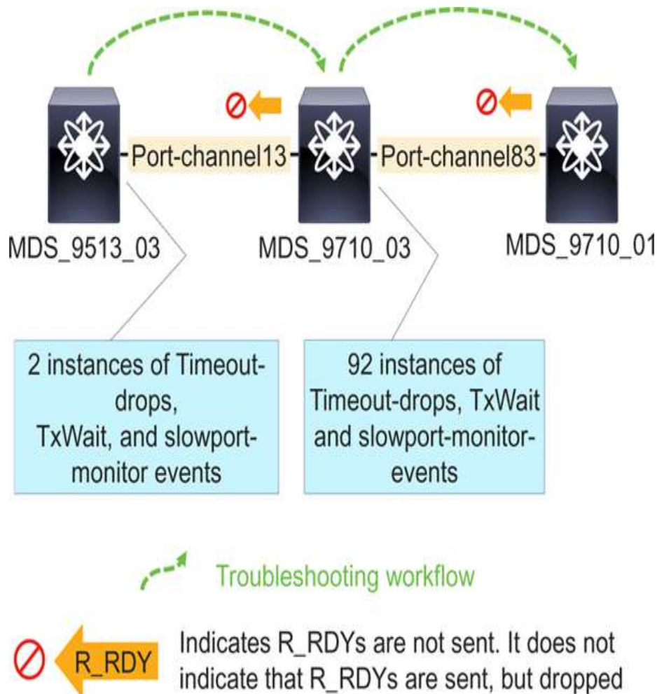
Figure 4-33 Congestion troubleshooting methodology and workflow
