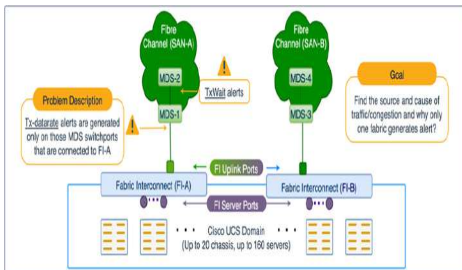
Figure 9-16 Traffic imbalance between FI-A and FI-B
