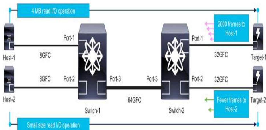
Figure 2-14 A typical edge-core storage network
