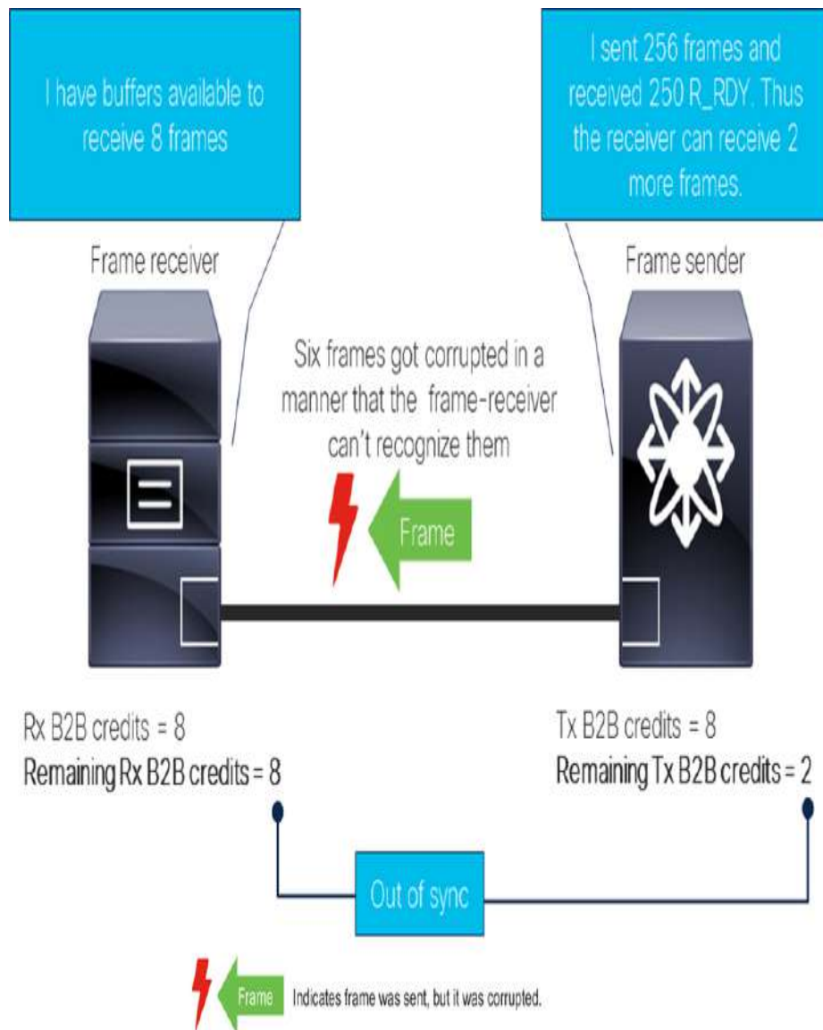
Figure 2-38 Loss of B2B credits due to a corrupted frame
