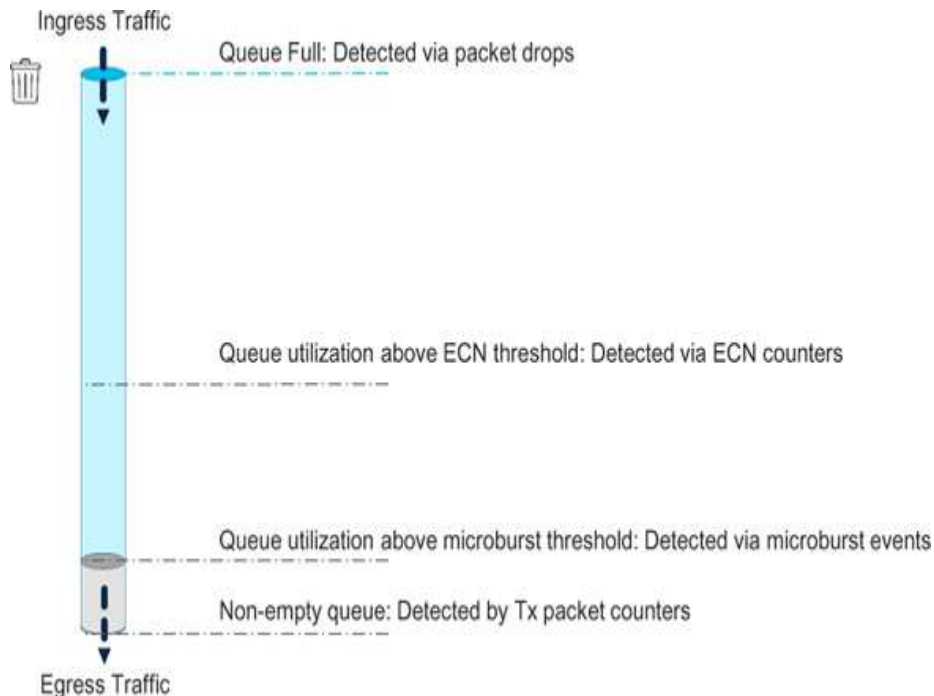
Figure 8-16 Queue utilization states and their detection mechanisms
