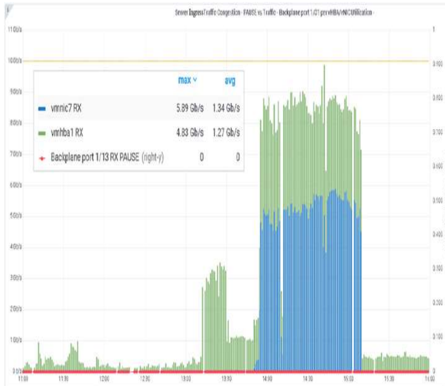
Figure 9-13 More traffic, but no Pause frames
