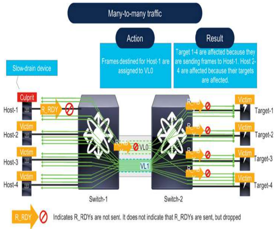
Figure 6-17 Congestion segregation using virtual links with many-to-many traffic
