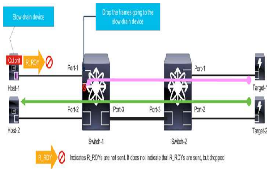
Figure 6-3 Congestion recovery by no-credit-drop timeout
