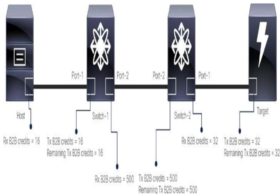
Figure 2-6 B2B flow control in a multi-hop fabric
