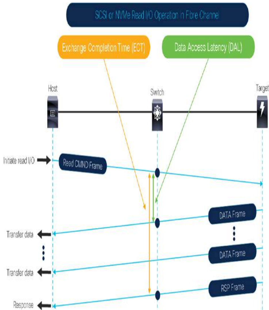
Figure 5-5 Latency metrics for a read I/O operation
