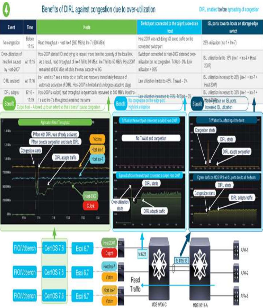
Figure 6-35 Port-Monitor detects congestion and instantly starts DURL
