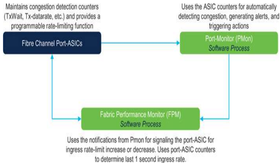
Figure 6-28 DIRM components in a Cisco MDS switch
