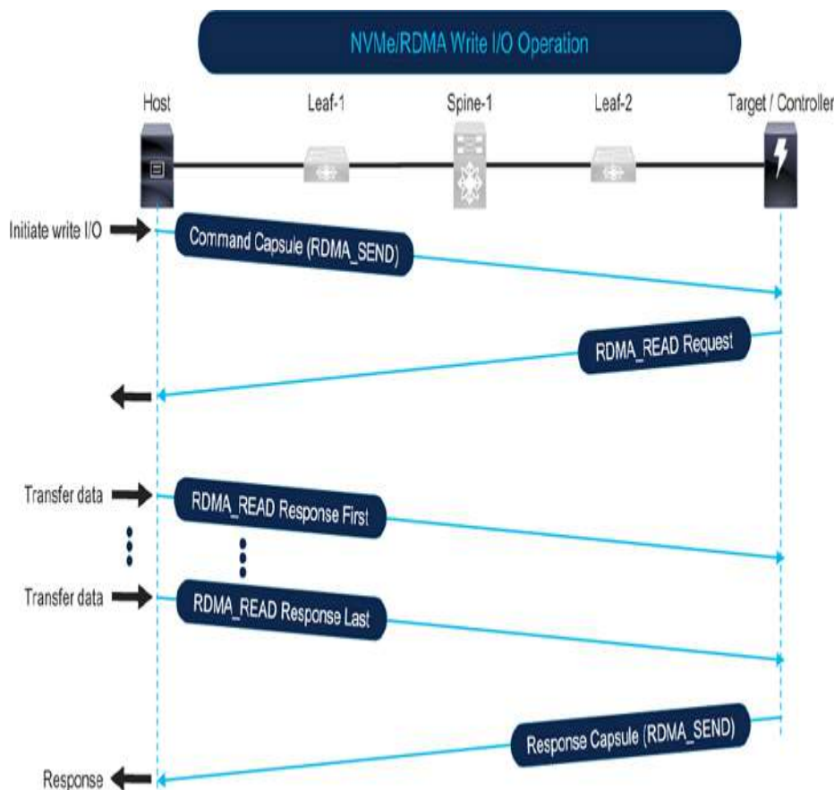
Figure 7-12 NVMe over RoCE write I/O operation
