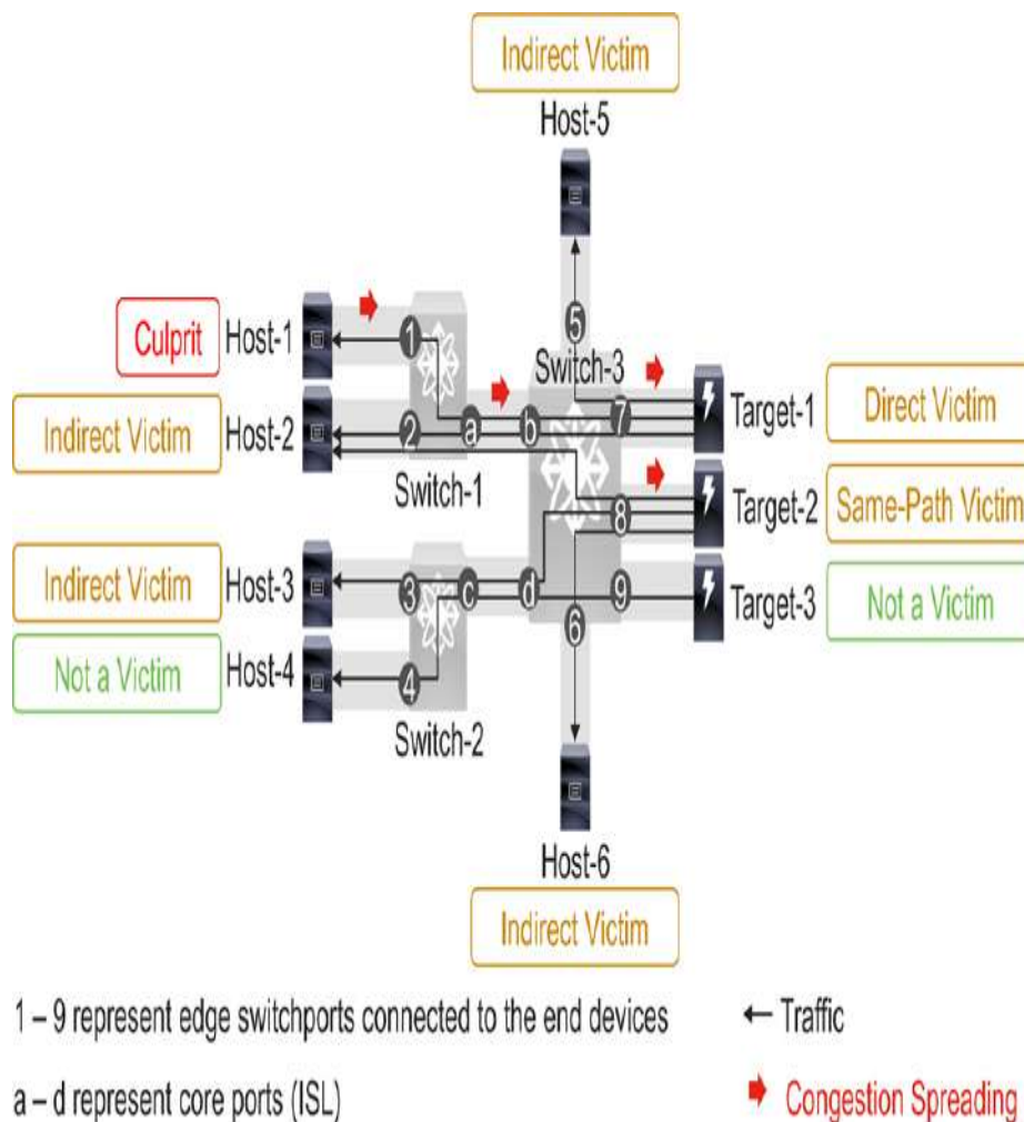
Figure 4-2 Types of Victims — Direct, Same-Path, and Indirect
