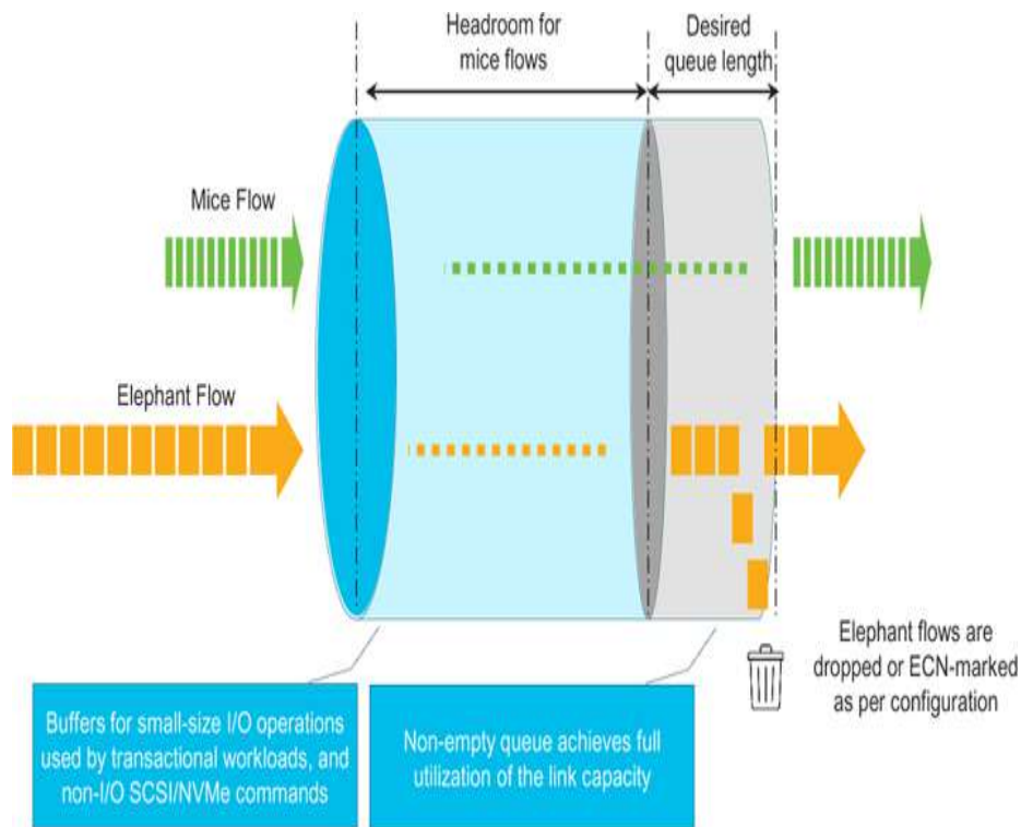
Figure 8-14 AFD mechanism
