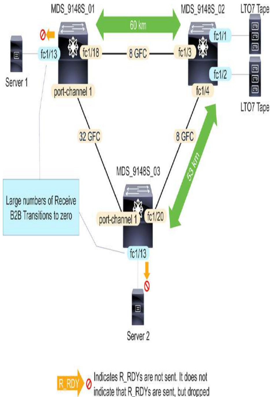
Figure 4-45 Receive B2B credit transitions to zero on the server-connected switchports
