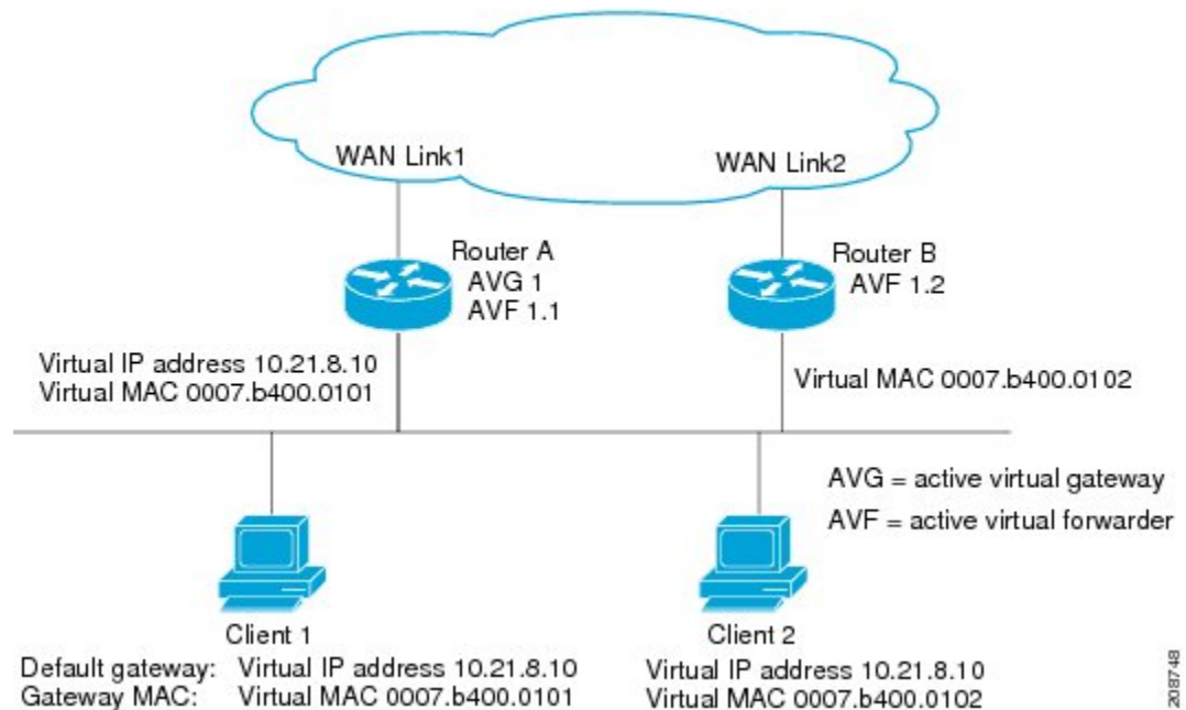
Figure 2: GLBP Topology
