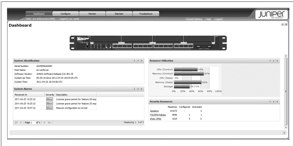
Figure 1-5. J-Web
