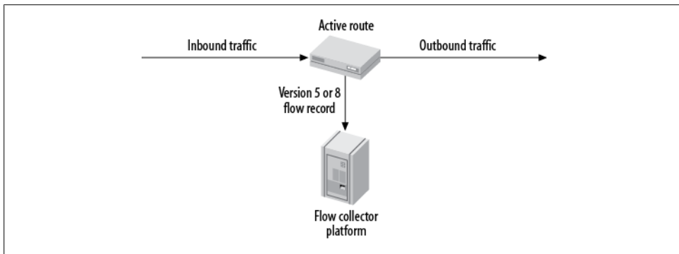
Figure 9-6. Active flow monitoring
