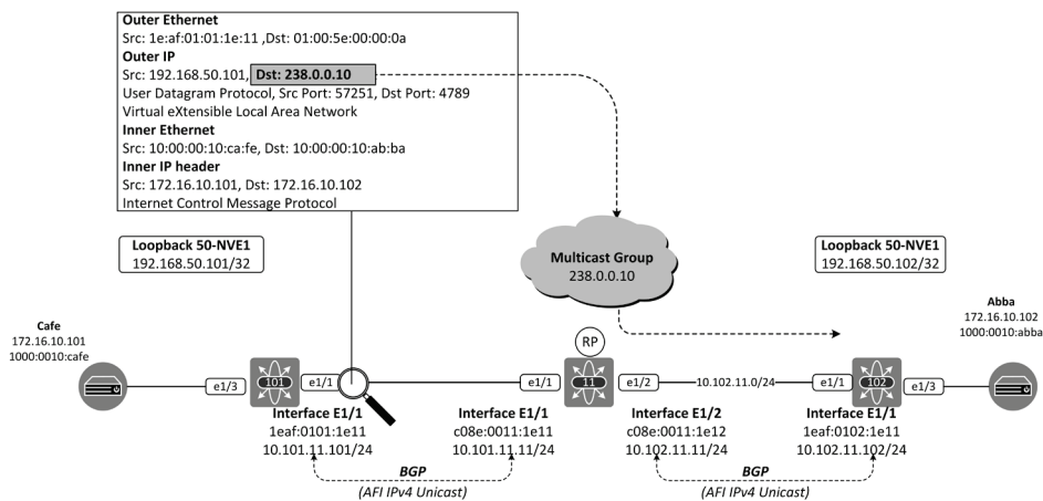
Figure 3-5: Spine-11 does not change the next-hop address 10.102.11.102.
