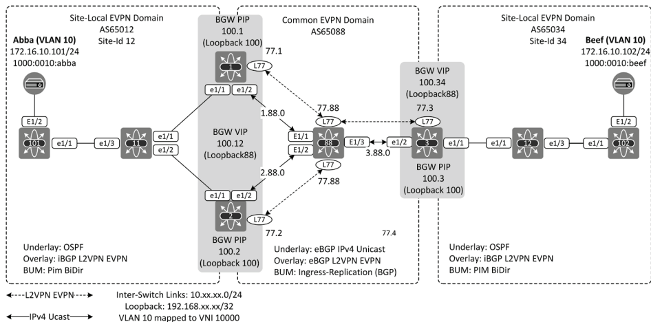
Figure 18-5: Common EVPN Domain Underlay and Overlay eBGP peering.
