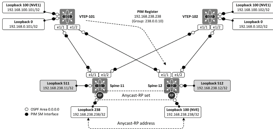
Figure 6-7: PIM Register message from VTEP-101 to MG 238.0.0.10.
