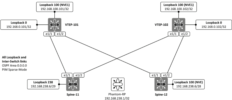
Figure 7-1: Example topology with Anycast-RP - IP addresses.
