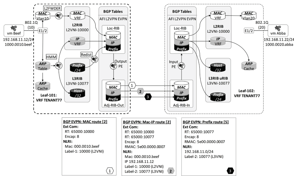
Figure 9-1: BGP EVPN Control Plane Operational Overview.
