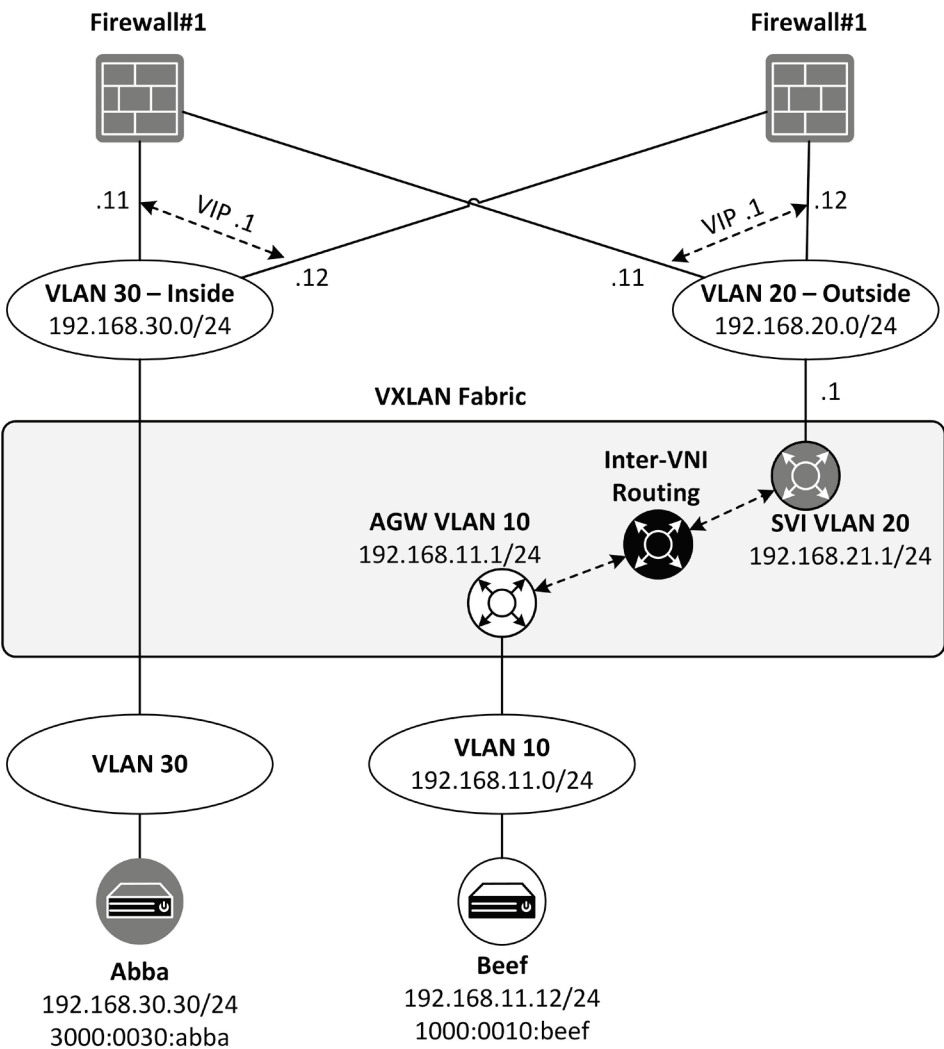
Figure 14-7: Simplified Topology
