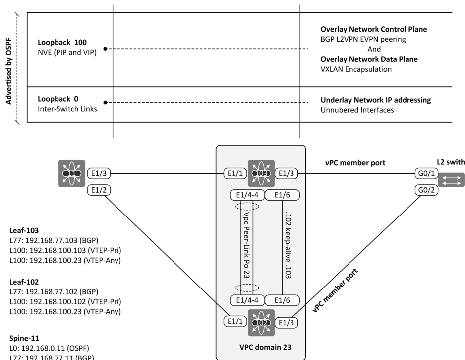
Figure 12-3: BGP EVPN peering and NVE1 interface are using same Loopback Interface
