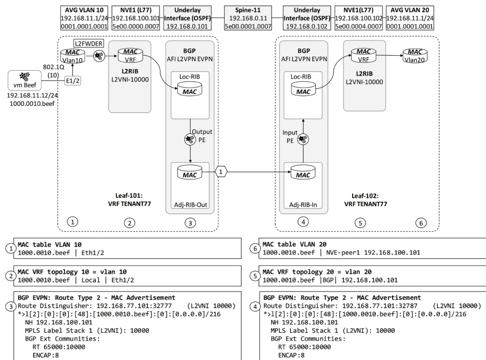
Figure 9-2: BGP EVPN Control Plane Operational MAC advertisement.
