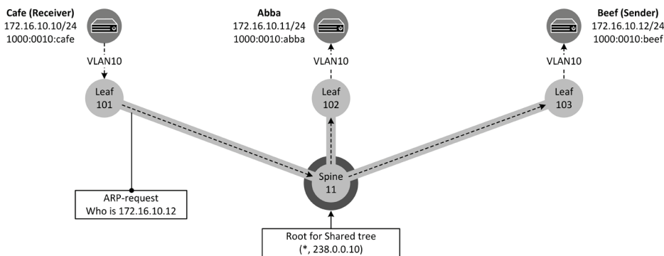
Figure 19-5: Underlay Network Shared tree rooted by Spine-11.
