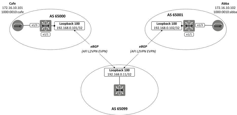
Figure 5-3: VXLAN Fabric Overlay Network eBGP L2VPN EVPN peering.
