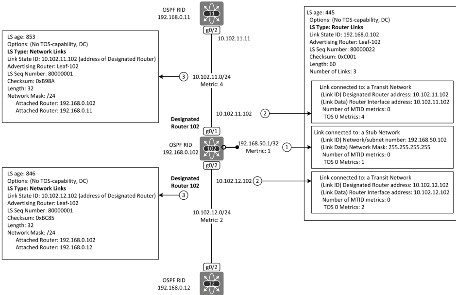
Figure 1-2: Router LSA and Network LSAs originated by Leaf-102 (DR).
