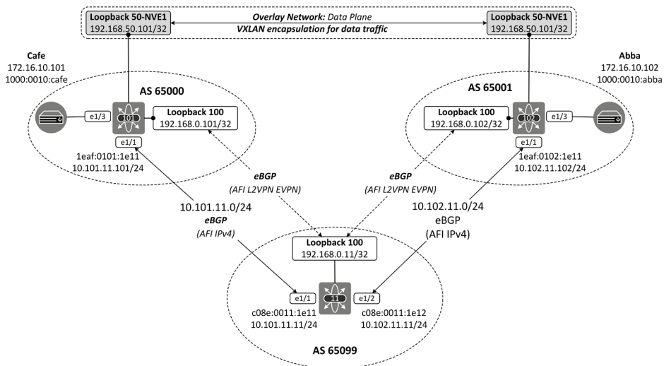
Figure 5-1: The MAC/IP addressing scheme and eBGP peering model.
