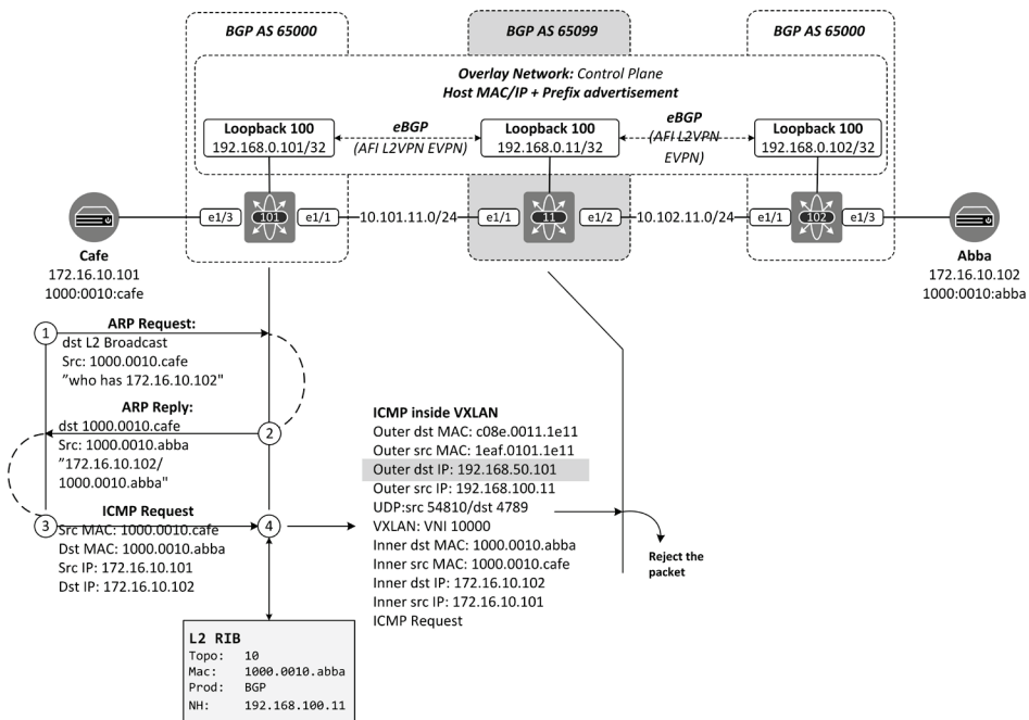
Figure 4-4: ICMP process.
