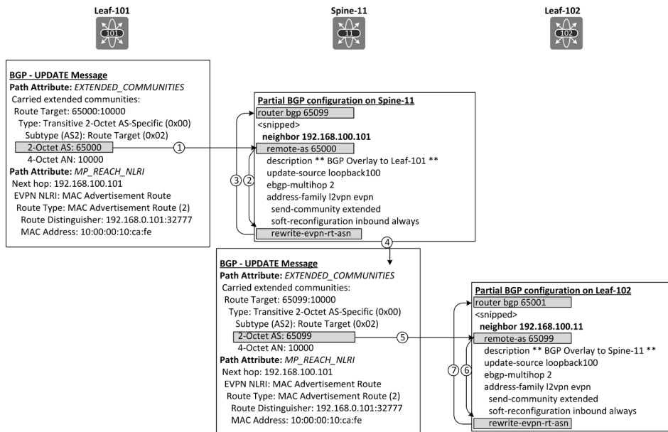
Figure 5-5: Route-Target rewrite process.
