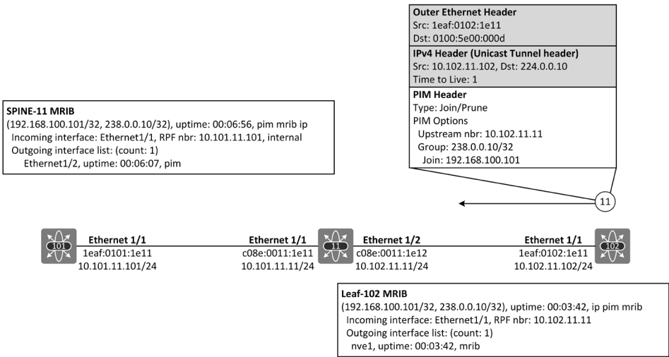
Figure 19-11: Source-Specific Tree join by Leaf-102.
