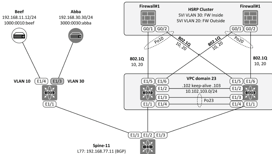
Figure 14-6: Physical topology
