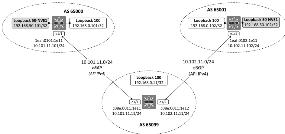
Figure 5-2: VXLAN Fabric Underlay Network eBGP IPv4 peering.
