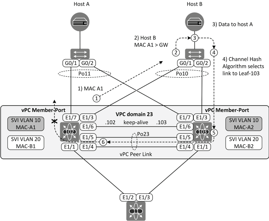
Figure 11-3: vPC peer-gateway
