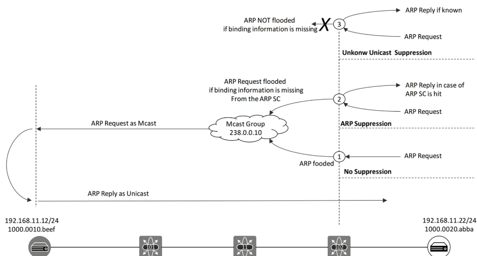
Figure 9-9: MAC-IP information in the ARP table and ARP Suppress Cache.
