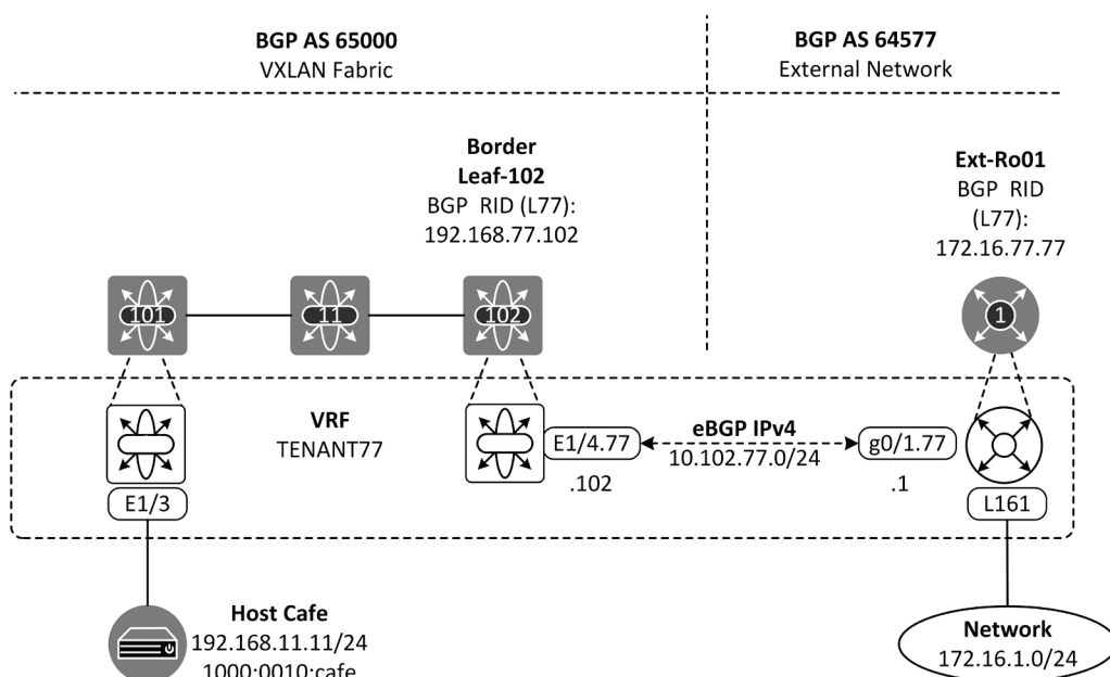
Figure 10-2: VXLAN Fabric external connection topology
