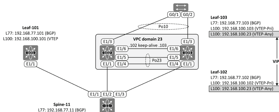
Figure 11-4: vPC PIP and VIP addressing
