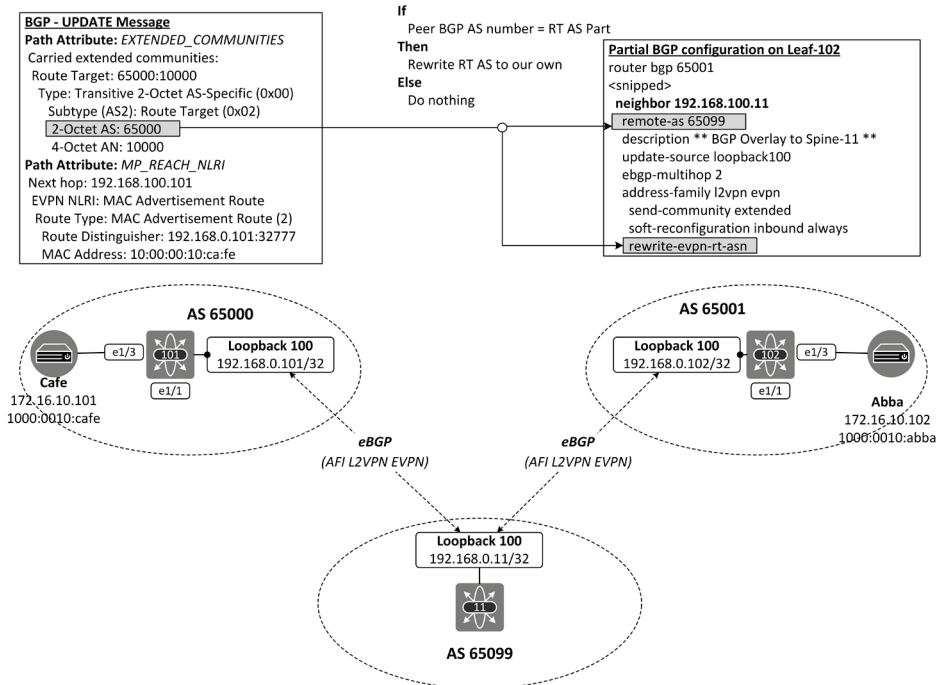
Figure 5-4: Route-Target rewrite process.
