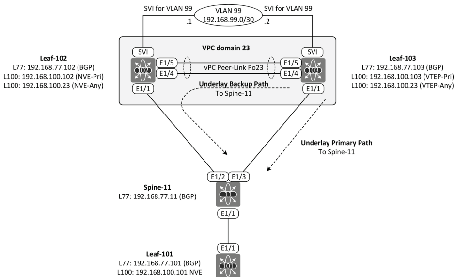
Figure 13-1: Example Topology and IP addressing
