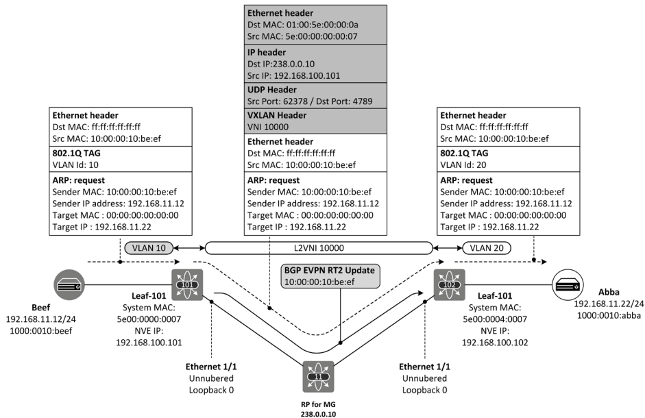
Figure 9-3: ARP request processing
