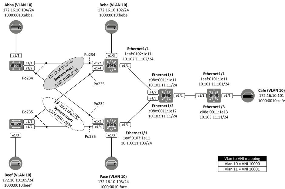
Figure 17-1: Topology an addressing scheme.
