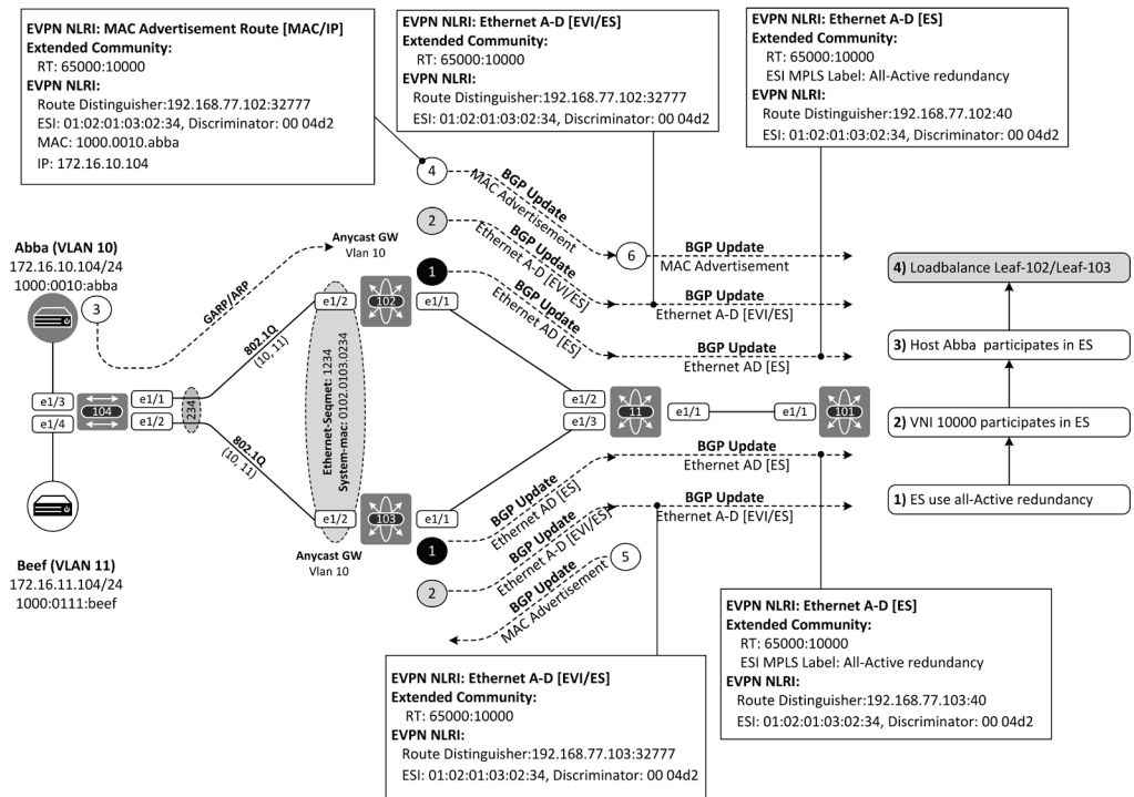
Figure 16-3: BGP EVPN ESI Multihoming Load Balancing (Aliasing).
