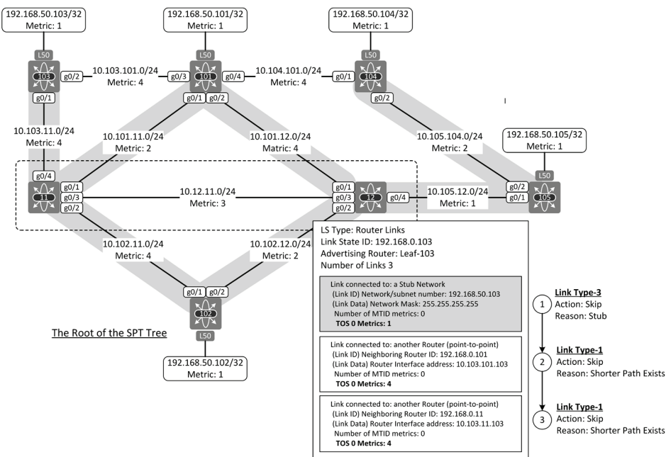
Figure 1-12: Shortest-Path Tree calculation: Seventh iteration round on Leaf-102.
