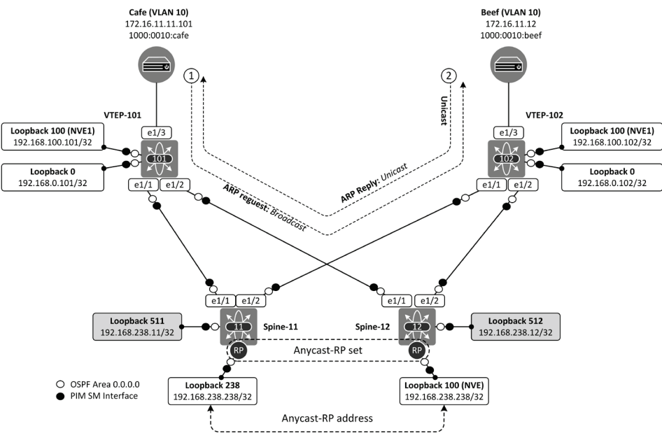
Figure 6-10: ARP Process.
