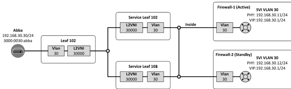
Figure 14-2: Protected network
