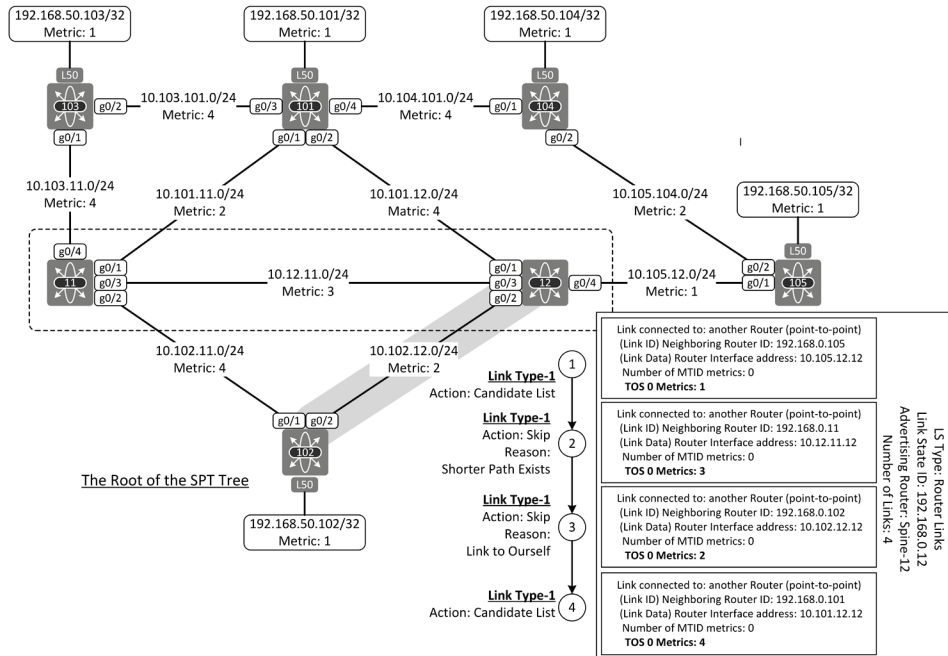
Figure 1-7: Shortest-Path Tree calculation: Second iteration round on Leaf-102.
