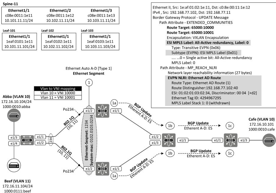
Figure 16-1: Ethernet A-D per Ethernet Segment (ES) route.
