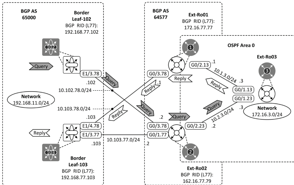
Figure 10-11: trace test#2
