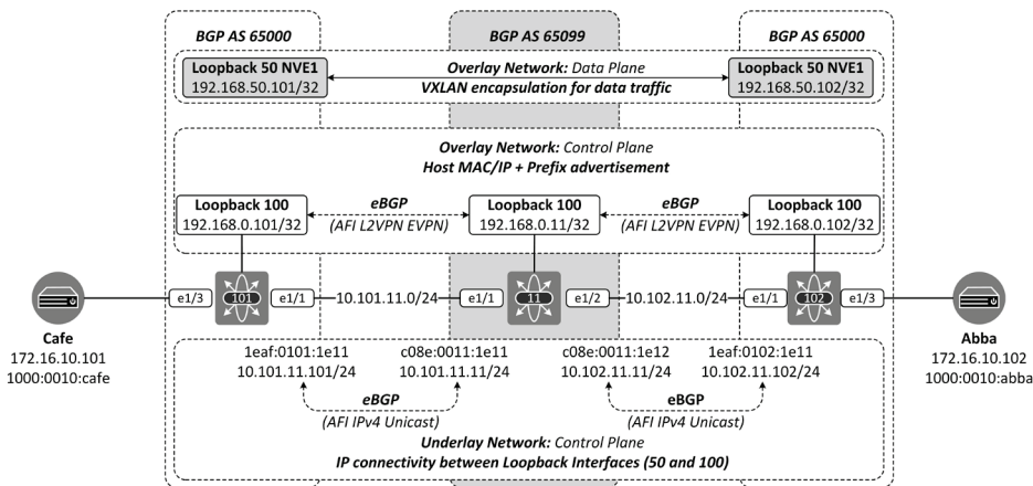
Figure 4-1: Example topology and addressing.
