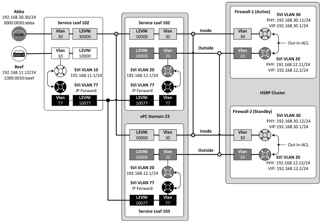
Figure 14-5: Complete logical view
