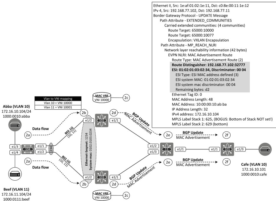
Figure 16-2: BGP EVPN Route-Type 2 MAC/IP advertisement.
