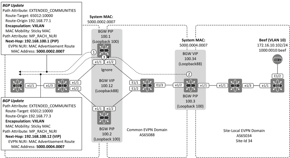
Figure 18-4: NVE peer learning process.
