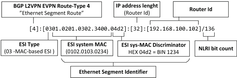
Figure 15-3: The VXLAN EVPN Multi-homing topology and addressing scheme.
