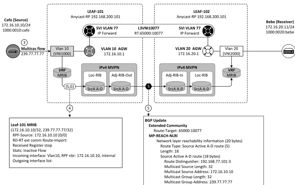
Figure 19-14: Source-Active Auto-Discovery by Leaf-101.
