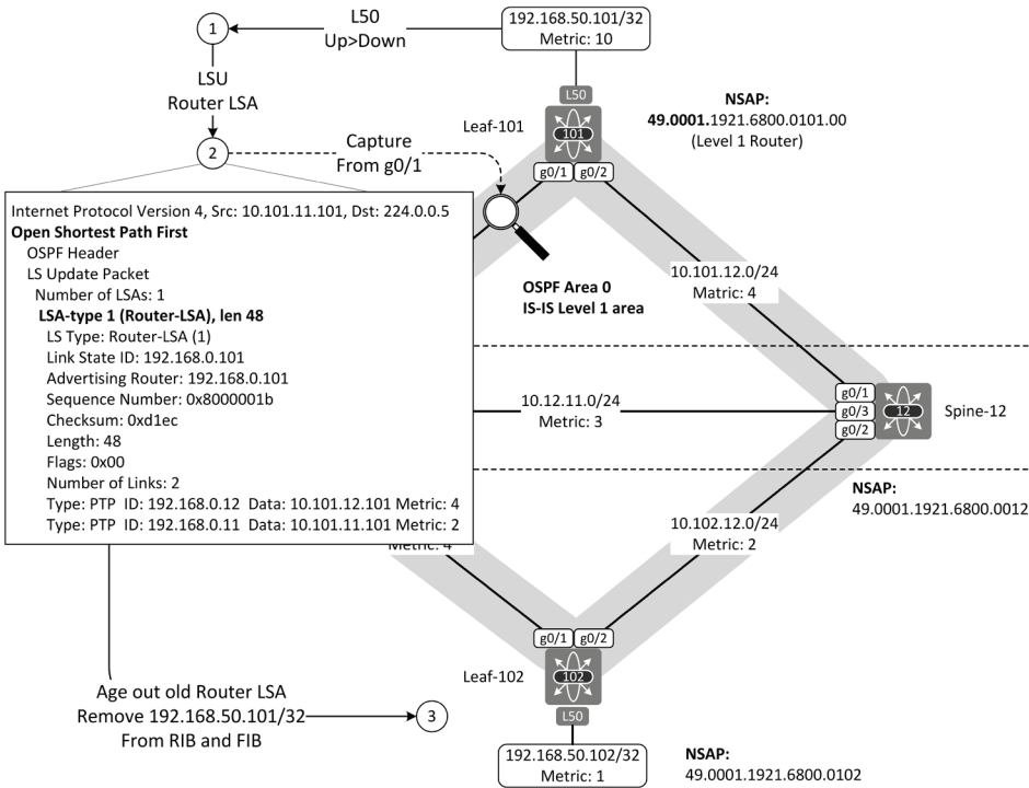
Figure 2-4: Interface Loopback 50 DOWN on Leaf-101 (OSPF).
