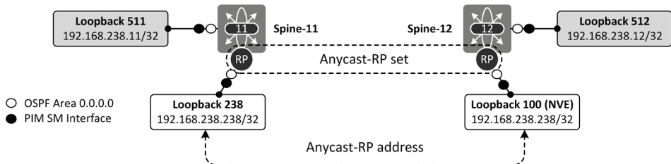
Figure 6-3: Anycast-RP Cluster Members.
