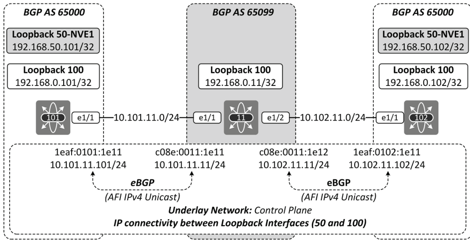
Figure 4-2: VXLAN Fabric Underlay Network eBGP IPv4 peering.
