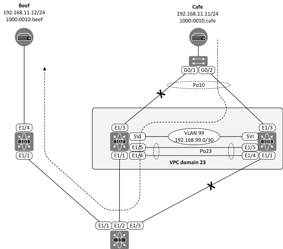
Figure 13-3: Backup path over vPC Peer Link
