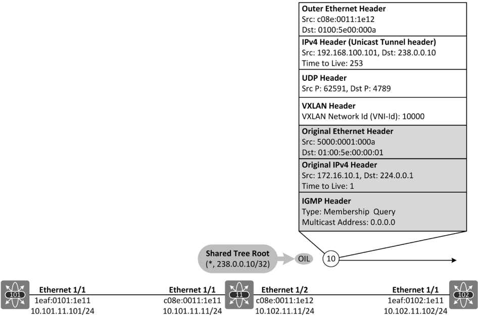
Figure 19-10: IGMP Membership Query forwarded by Spine-11.
