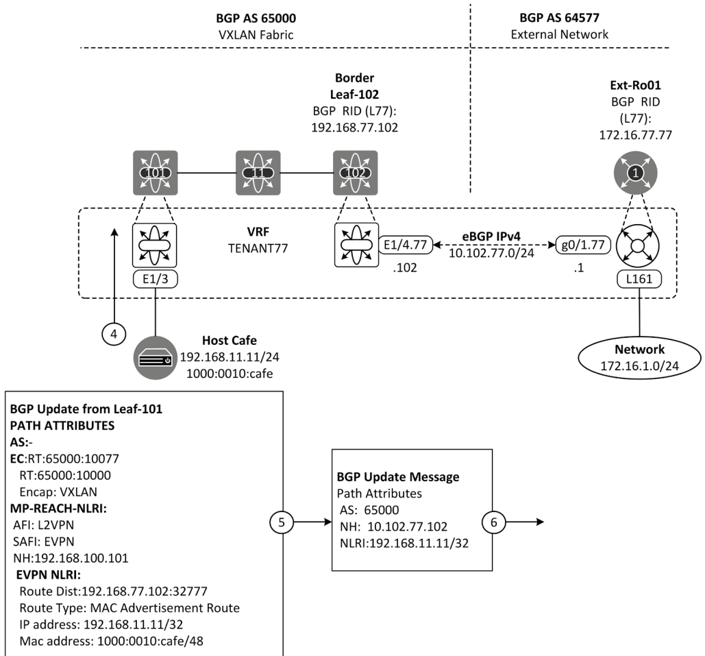
Figure 10-6: BGP Update from Border Leaf-102 to Leaf-102 via RR Spine-11.
