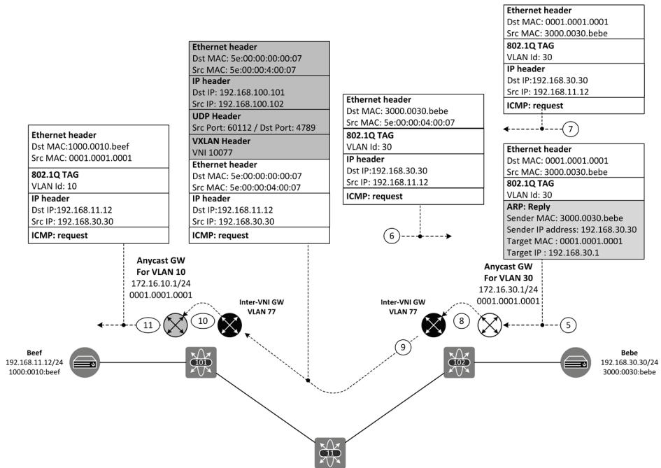
Figure 9-18: Silent host discovery process, Phases 5-11.
