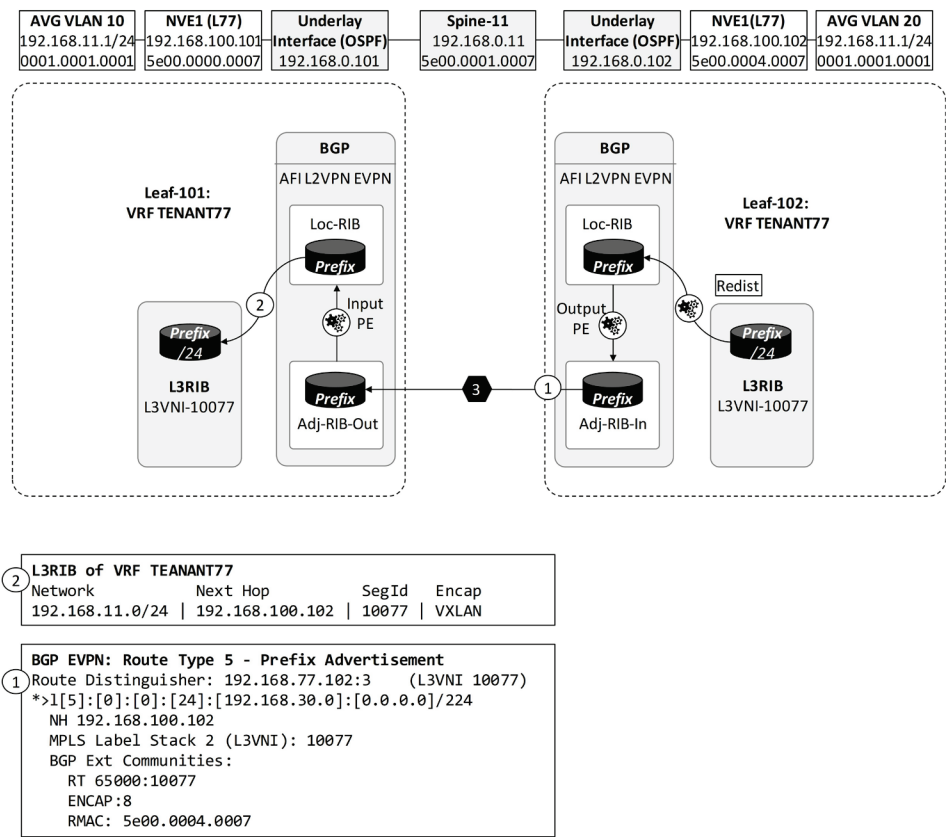
Figure 9-16: BGP EVPN Route type 5 – Prefix advertisement.
