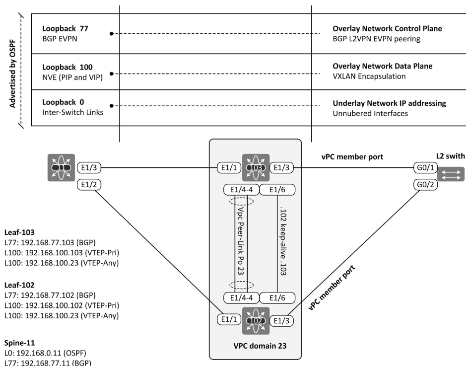
Figure 12-1: VXLAN BGP EVPN Example Topology and IP addressing
