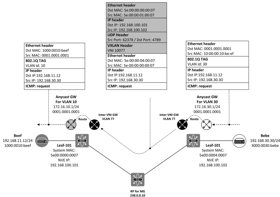
Figure 9-13: Inter-VNI routing process.
