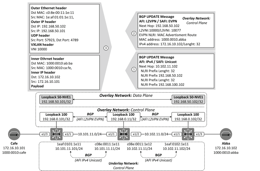
Figure 3-1: High-Level operation of VXLAN Fabric
