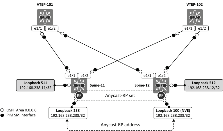
Figure 6-1: Example topology with Anycast-RP - IP addresses.
