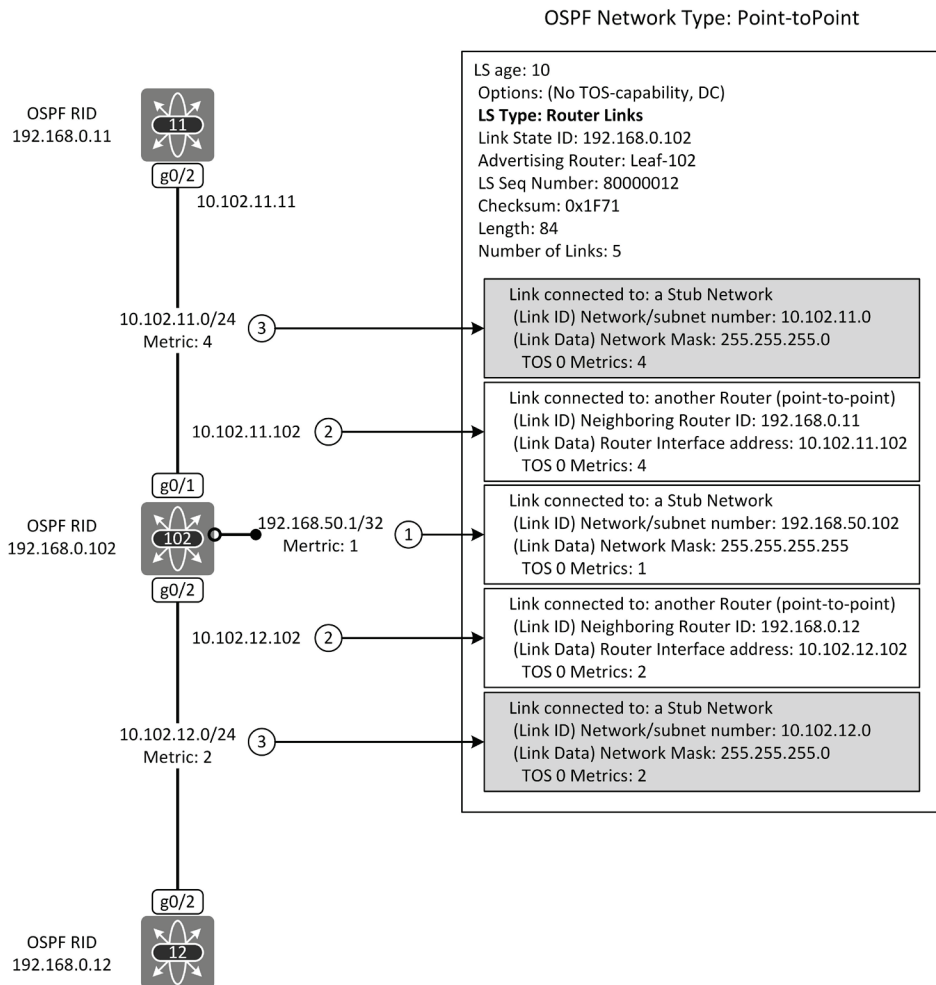
Figure 1-3: Router LSA originated by Leaf-102.
