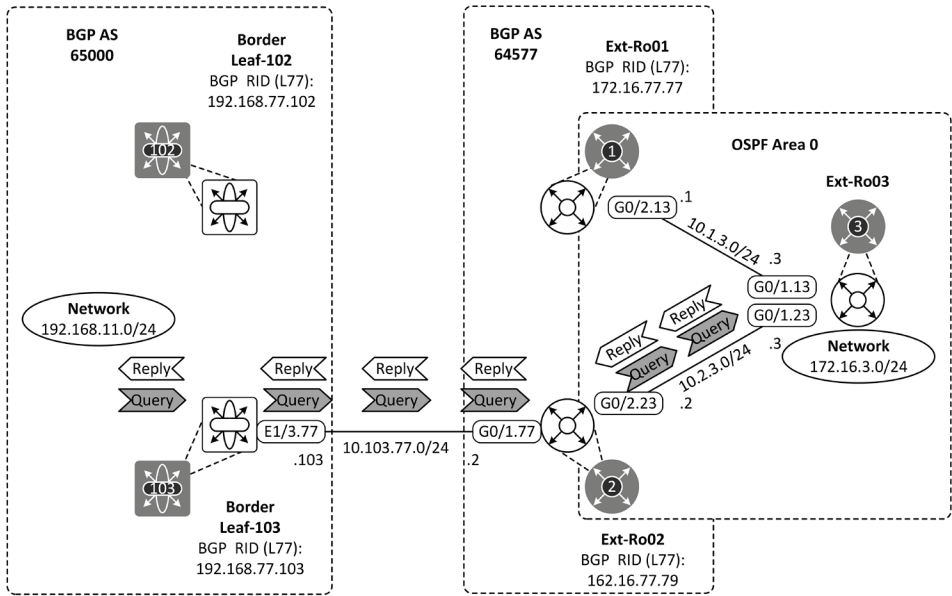
Figure 10-13: trace test#4
