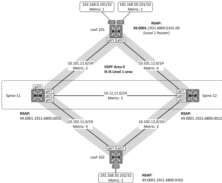
Figure 2-2: Example topology.
