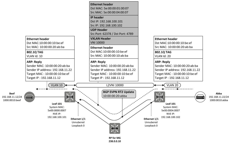
Figure 9-4: ARP reply processing
