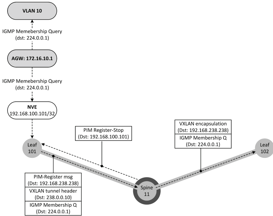
Figure 19-7: PIM-Join to Source-Specific Tree.
