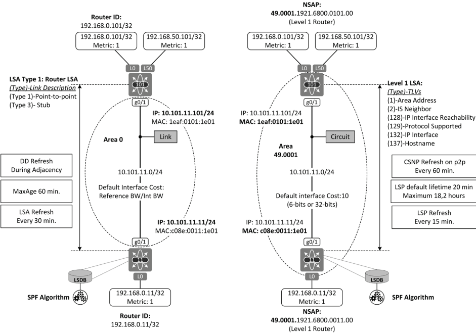
Figure 2-1: Comparison of OSPF and IS-IS.
