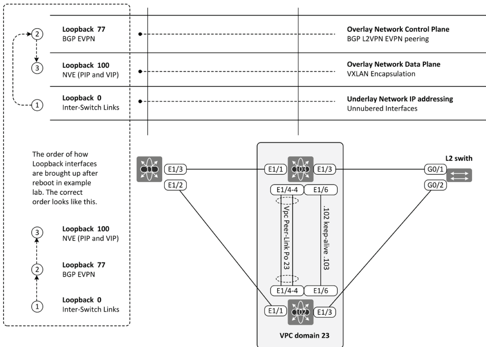
Figure 12-4: Loopback interface “enabling” order during device boot.
