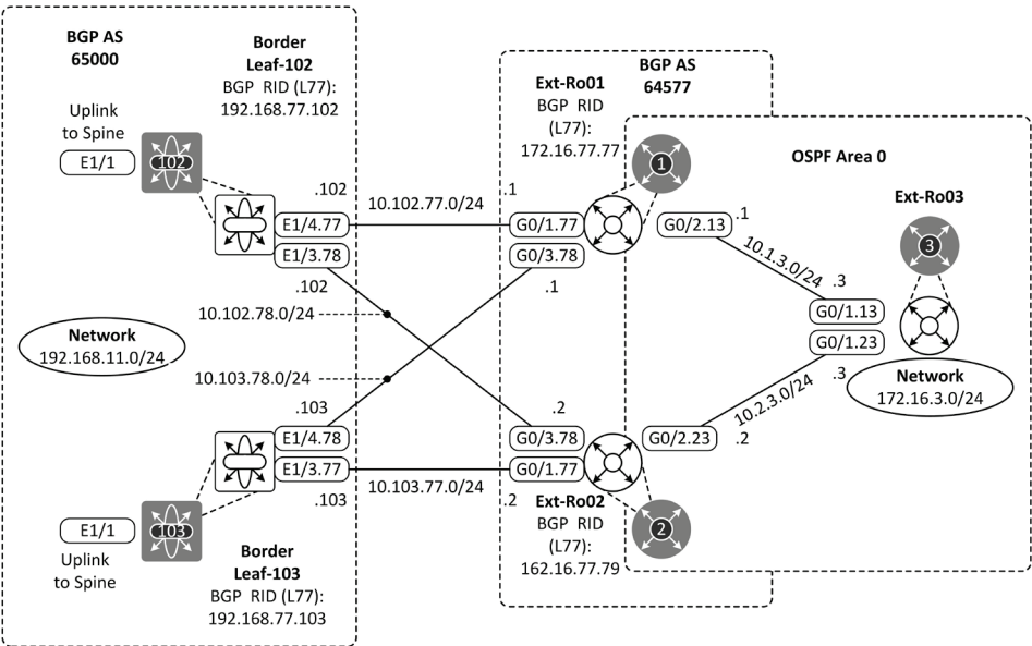
Figure 10-1: VXLAN Fabric external connection basic setup.
