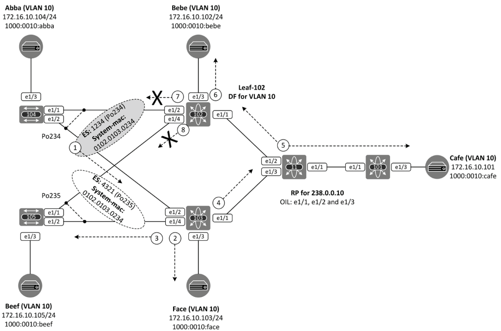
Figure 17-5: BUM from non-DF perspective.
