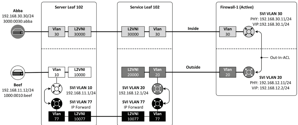
Figure 14-4: Logical view
