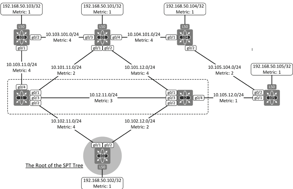
Figure 1-5: Shortest-Path Tree calculation: Starting Point
