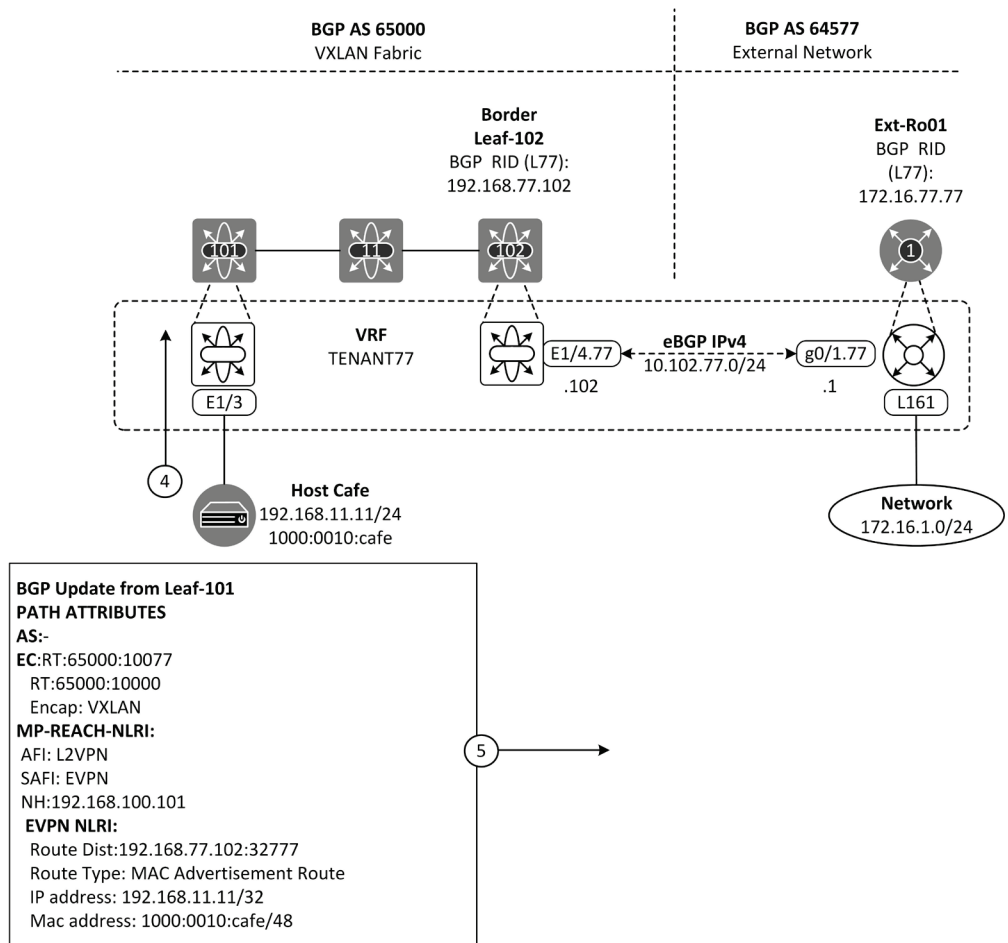
Figure 10-5: BGP Update from Leaf-101 to Border Leaf-102 via RR Spine-11.
