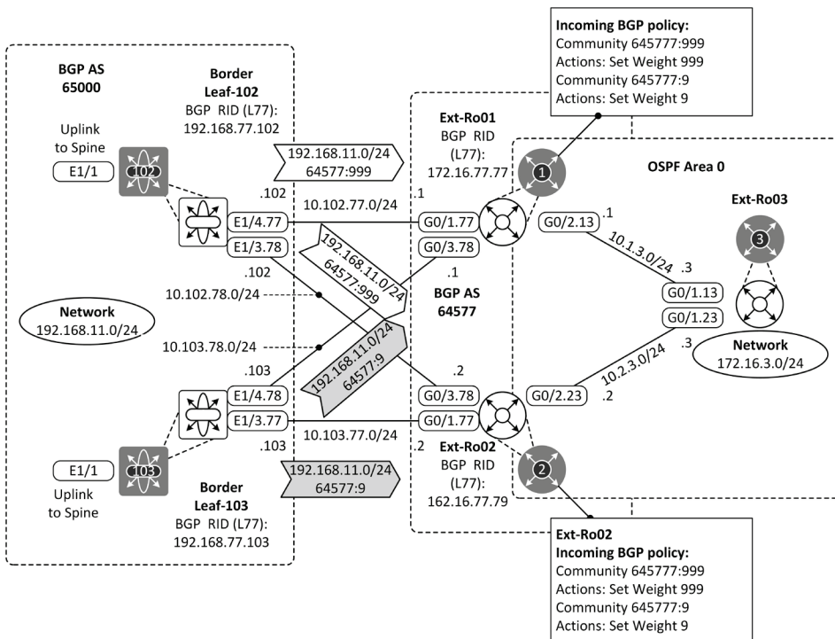
Figure 10-9: BGP policy concerning network 192.168.11.0/24.
