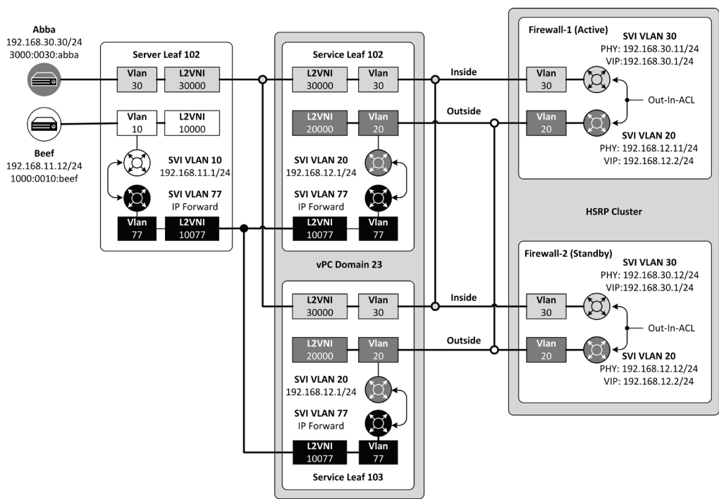
Figure 14-1: Example Topology and IP addressing
