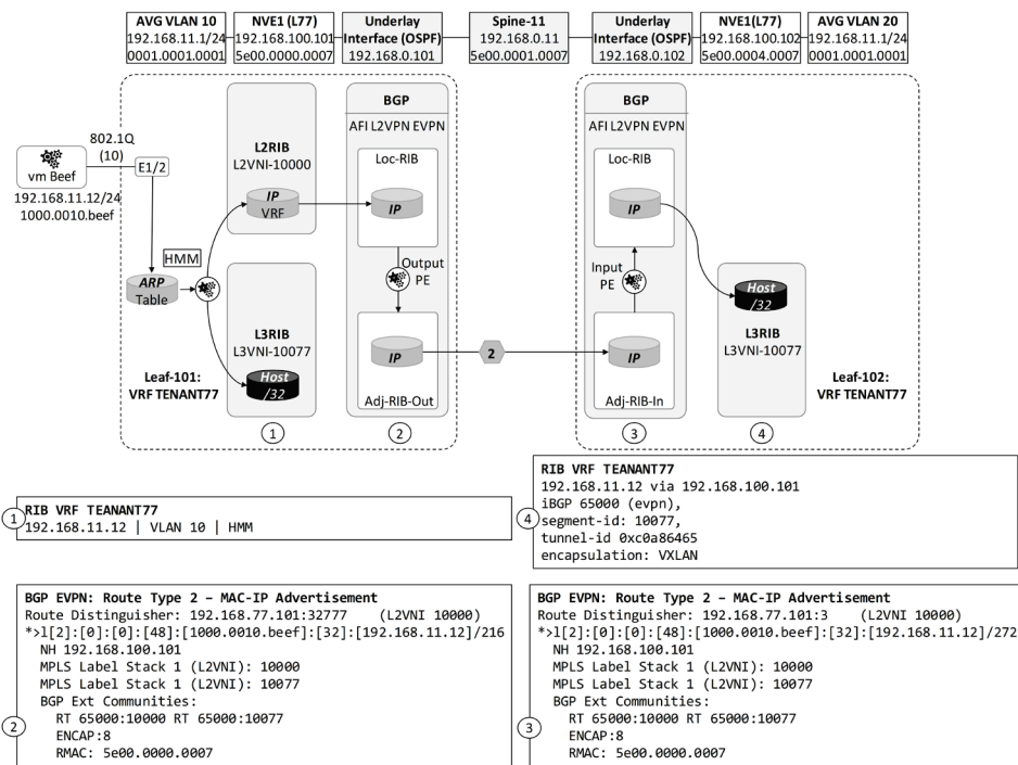
Figure 9-11: Host route propagation over VXLAN Fabric.
