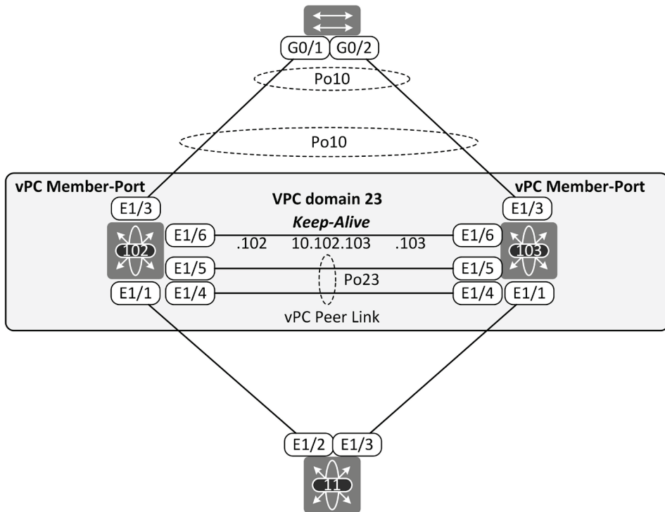
Figure 11-2: vPC domain
