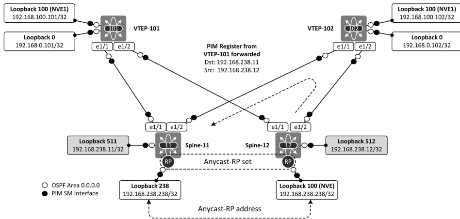
Figure 6-9: PIM Register-Stop message from Spine-12 to Spine-11.
