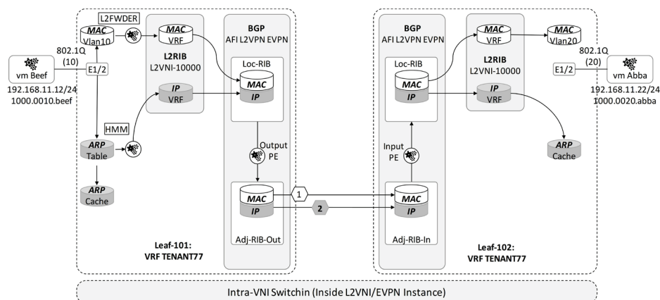
Figure 9-10: MAC-IP information in ARP table and ARP Suppress Cache.
