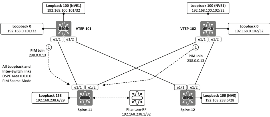
Figure 7-2: Example topology with Anycast-RP - IP addresses.
