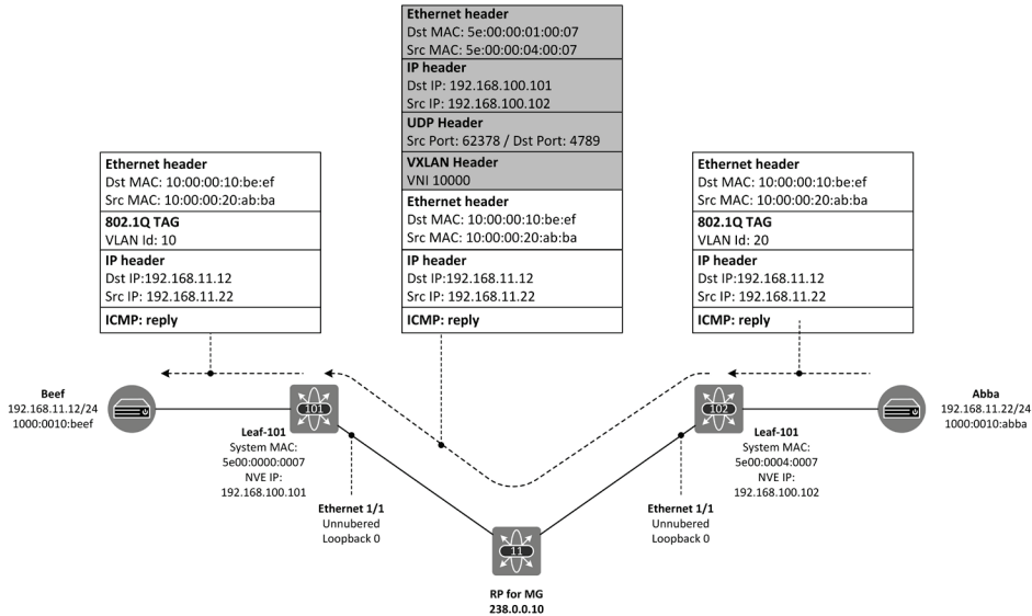
Figure 9-6: ICMP Reply from vmAbba to vmBeef.
