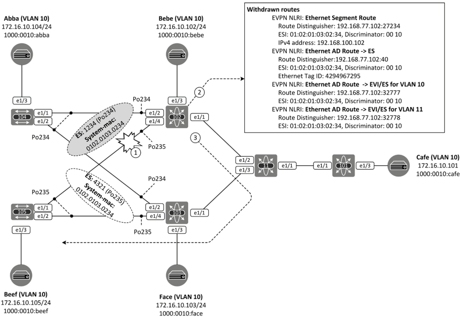
Figure 17-2: Link failure on Leaf-102.
