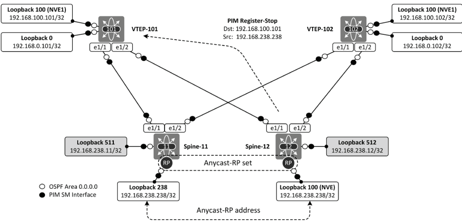
Figure 6-8: PIM Register-Stop message from Spine-12 to VTEP-101.
