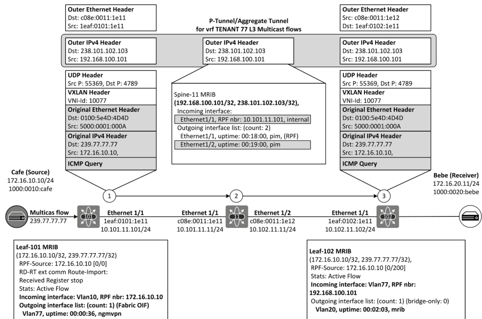
Figure 19-16: TRM Data Plane operation.
