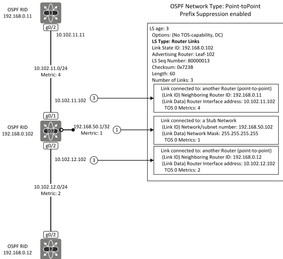
Figure 1-4: Router LSA originated by Switch 102.
