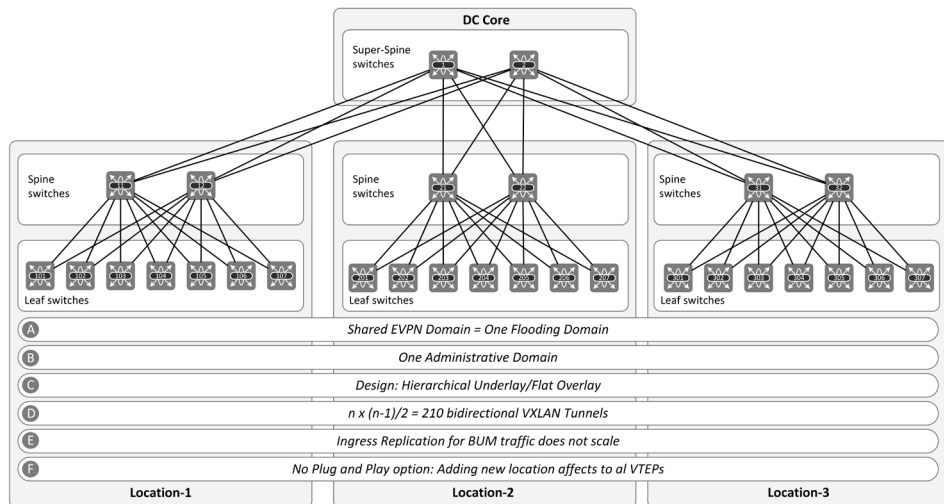
Figure 18-1: Characteristics of Super-Spine VXLAN fabric.
