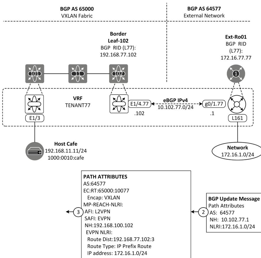
Figure 10-4: BGP Update from Border Leaf-102 to Leaf-101 via RR Spine-11.
