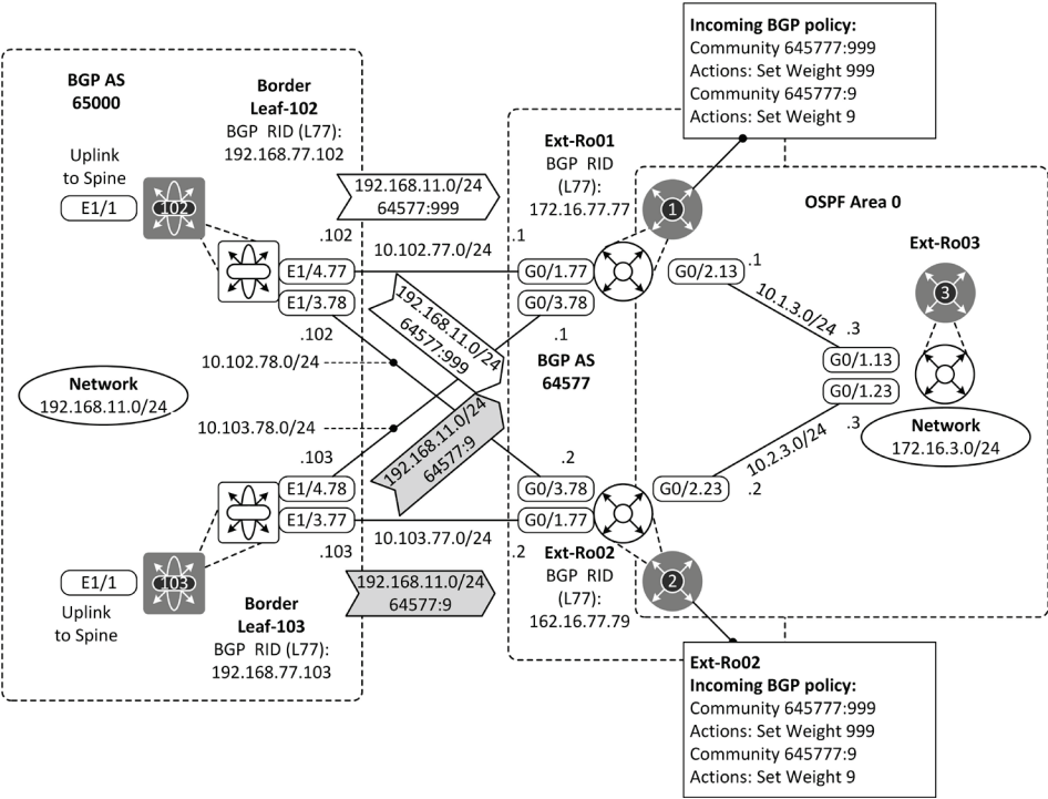
Figure 10-8: BGP Update from Border Leaf-102 and 103 to External routers.
