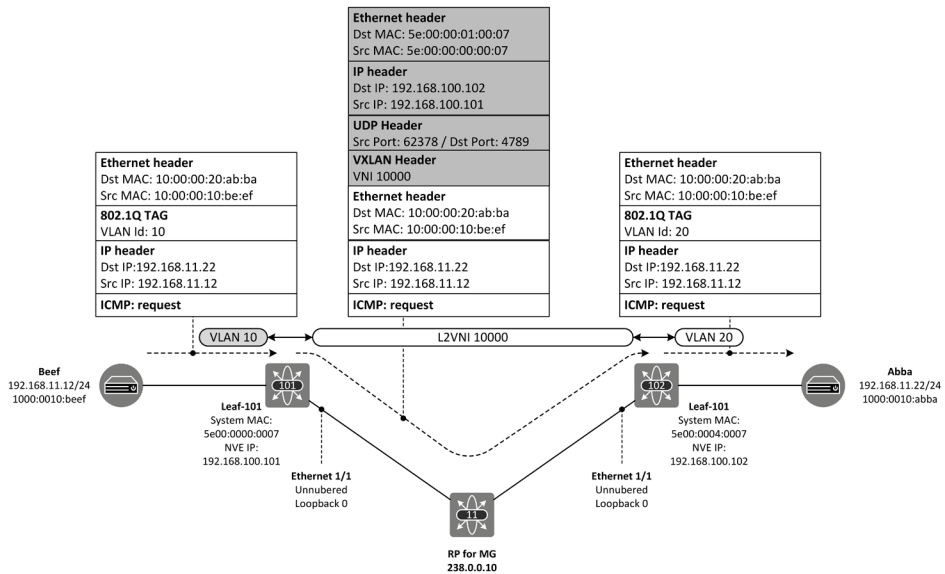
Figure 9-5: ICMP request from vmBeef to Abba.
