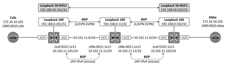
Figure 3-3: Underlay/Overlay BGP peering and NVE peering.
