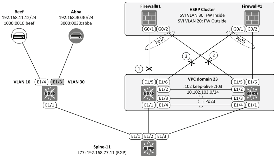
Figure 14-8: Test scenarios
