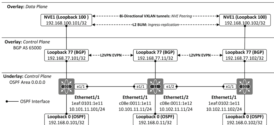
Figure 8-1: Example topology and addressing scheme.
