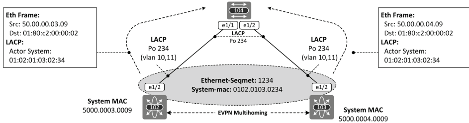
Figure 15-2: EVPN ESI Multihoming:
