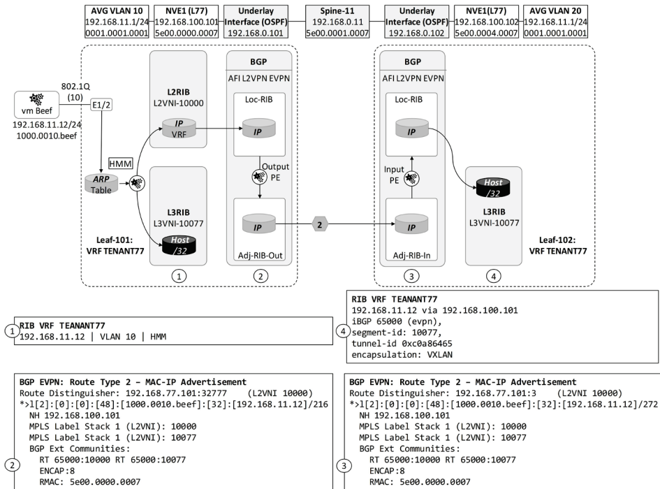
Figure 9-12: Host route propagation over VXLAN Fabric.
