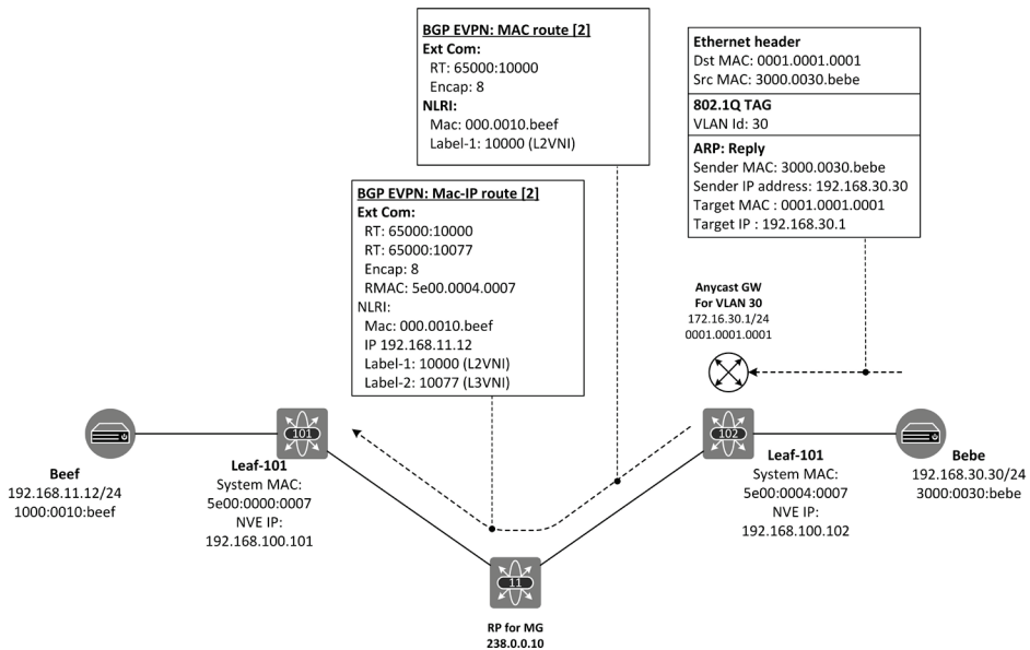
Figure 9-15: Silent host discovery process, Phases 4-6
