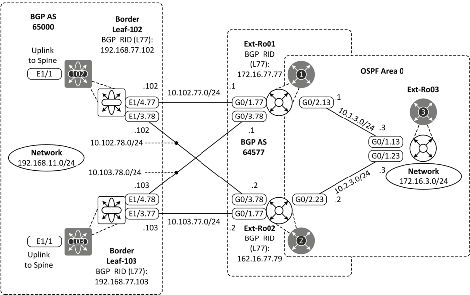
Figure 10-7: full-mesh external BGP peering topology.
