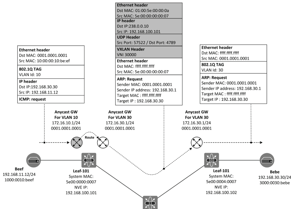
Figure 9-14: Silent host discovery process, Phases 1-3
