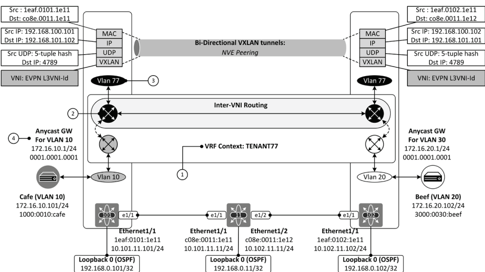
Figure 8-4: Inter-VNI Routing model.
