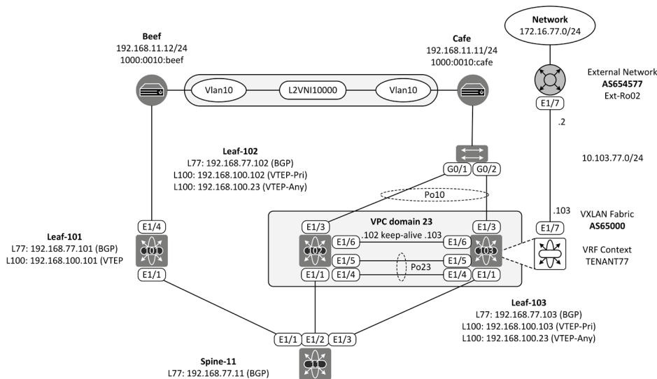
Figure 11-1: VXLAN BGP EVPN vPC Example Topology and IP addressing
