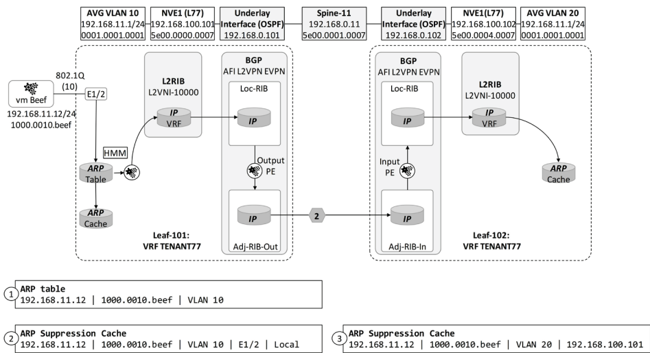
Figure 9-8: MAC-IP information in ARP table and ARP Suppress Cache.
