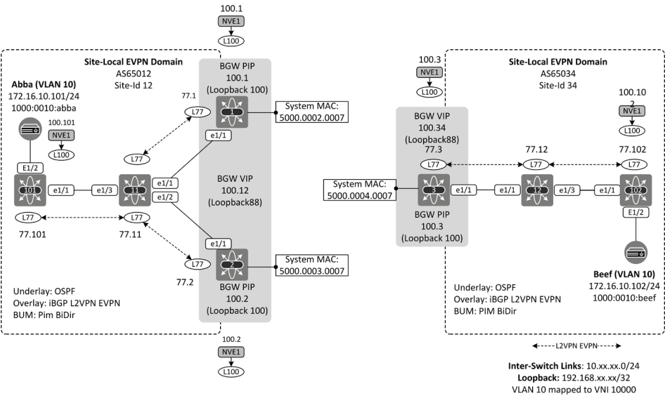
Figure 18-3: Example EVPN Multi-Site topology.
