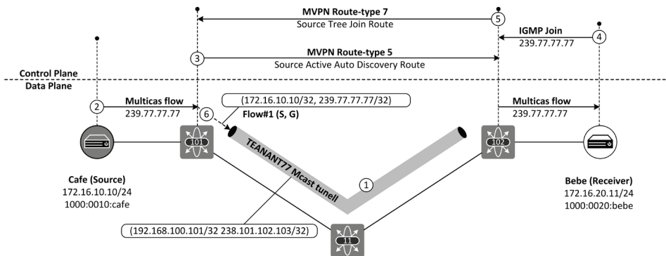
Figure-19-1: Tenant Routed Multicast (TRM) Topology.
