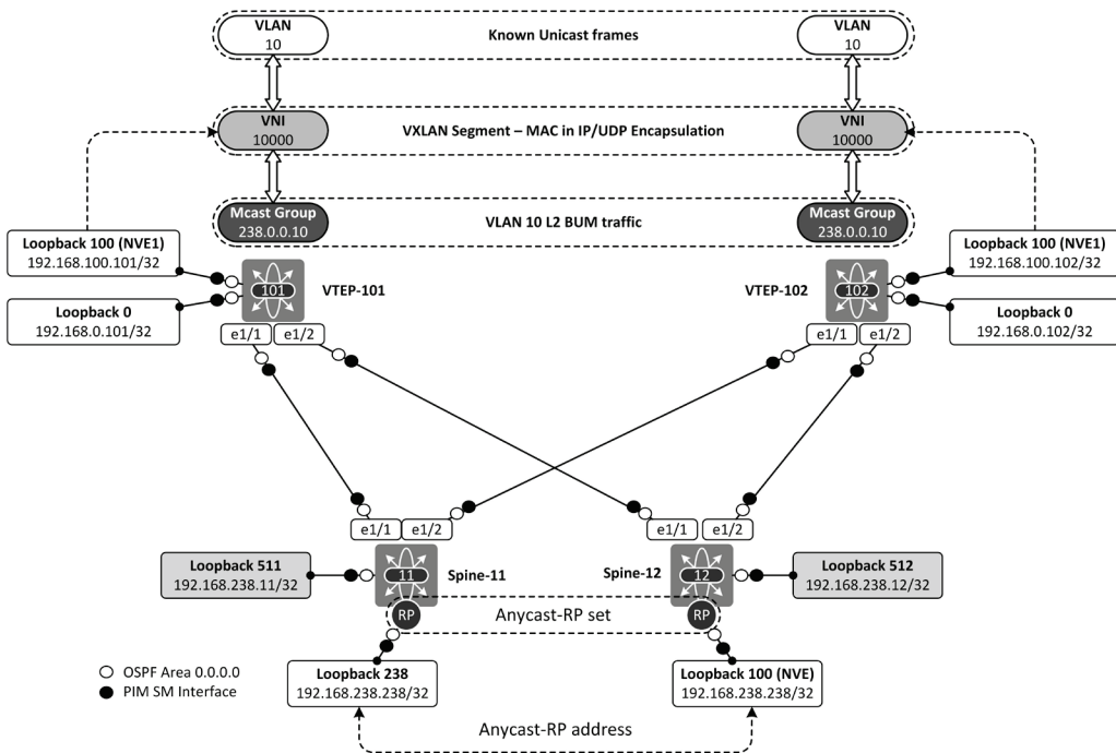
Figure 6-5: VLAN-to-VNI-to-Multicast Group
