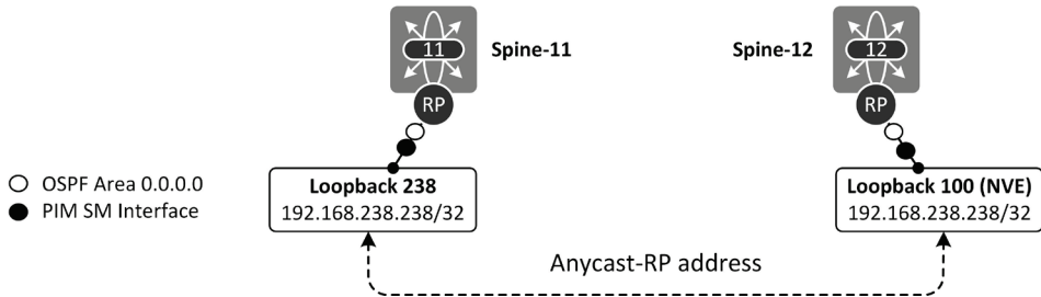
Figure 6-2: Anycast-RP Cluster Members.
