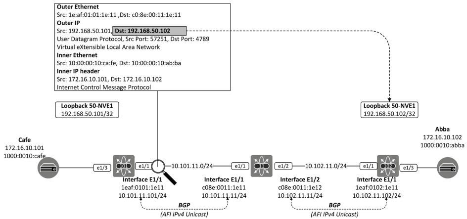
Figure 3-4: Spine-11 change the next-hop from 10.102.11.102 to 10.101.11.11.
