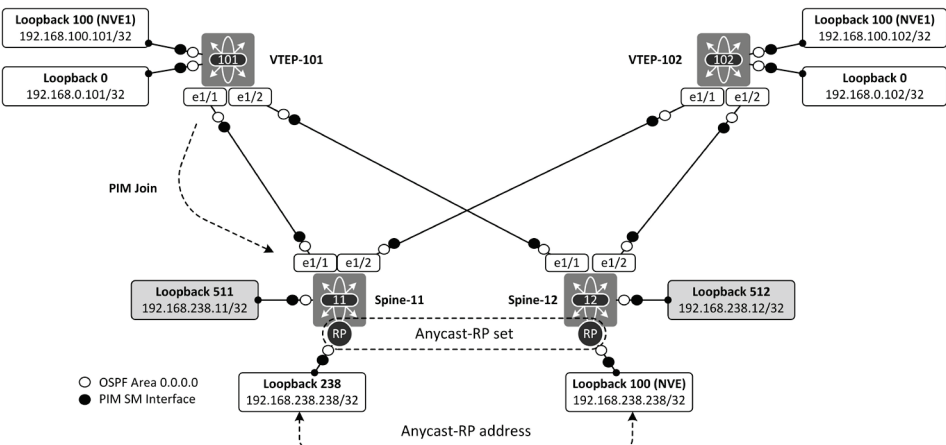
Figure 6-6: PIM Join message from VTEP-101 to MC 238.0.0.10.
