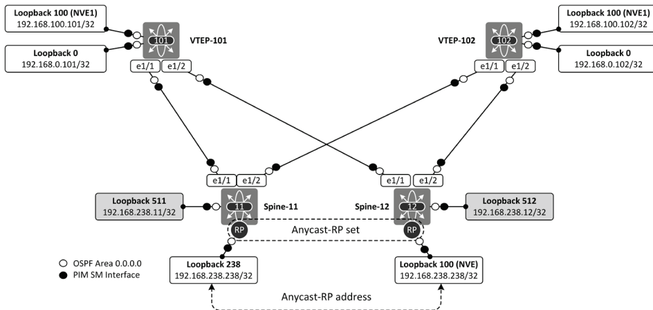
Figure 6-4: Anycast-RP Cluster Members.
