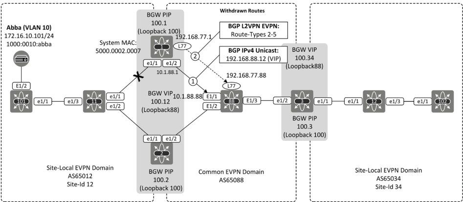
Figure 18-9: Intra-site fabric-link failure on BGW-1.
