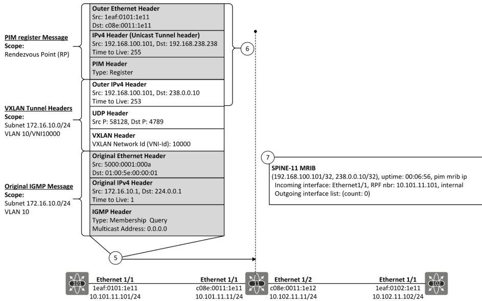
Figure 19-8: IGMP Membership Query/PIM-Register originated by Leaf-101.
