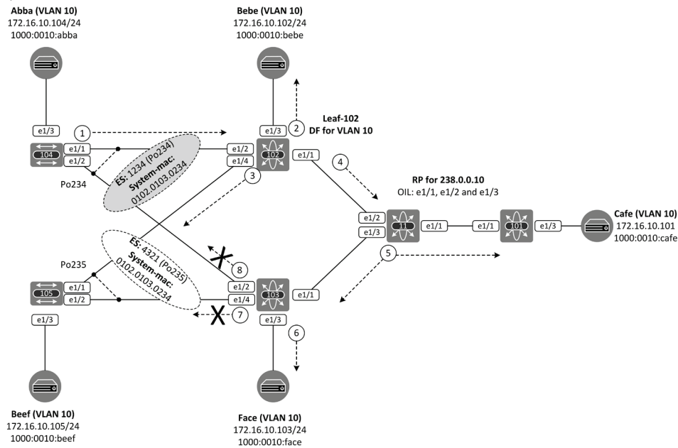
Figure 17-4: BUM from DF perspective.
