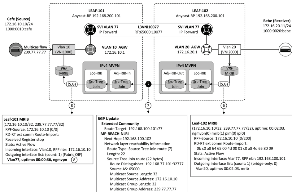
Figure 19-15: Source-Tree Join Route by Leaf-102.
