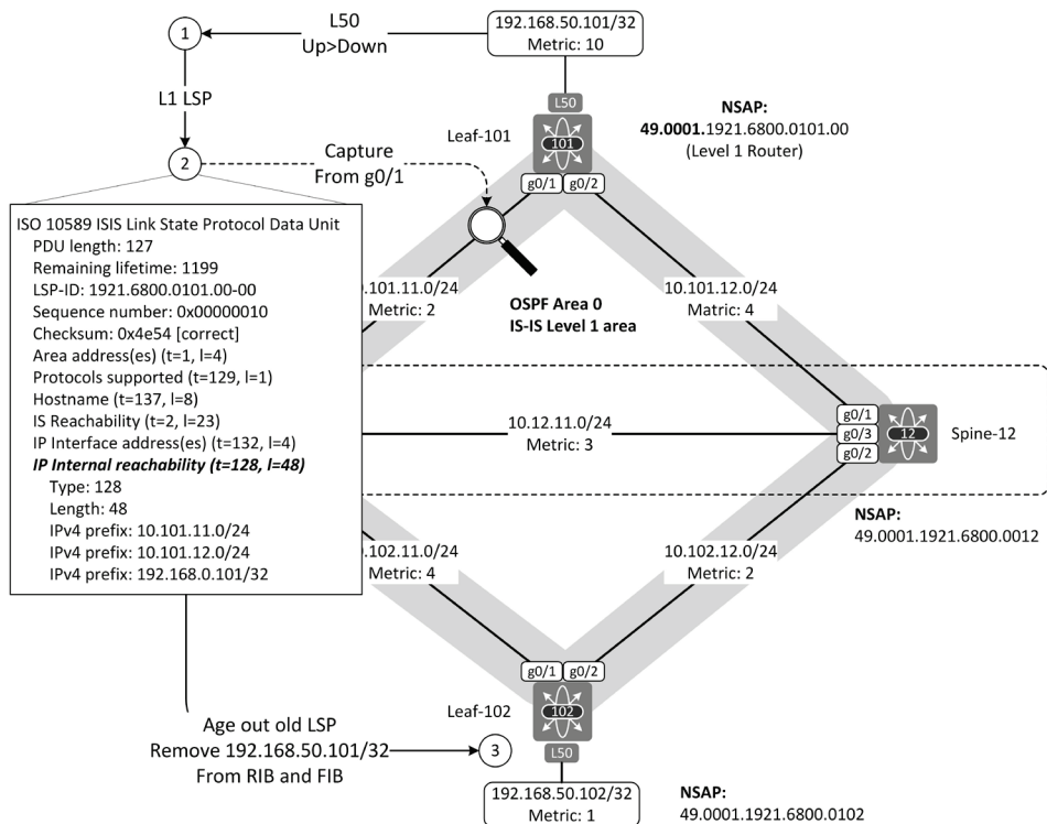
Figure 2-3: Interface Loopback 50 DOWN on Leaf-101 (IS-IS).
