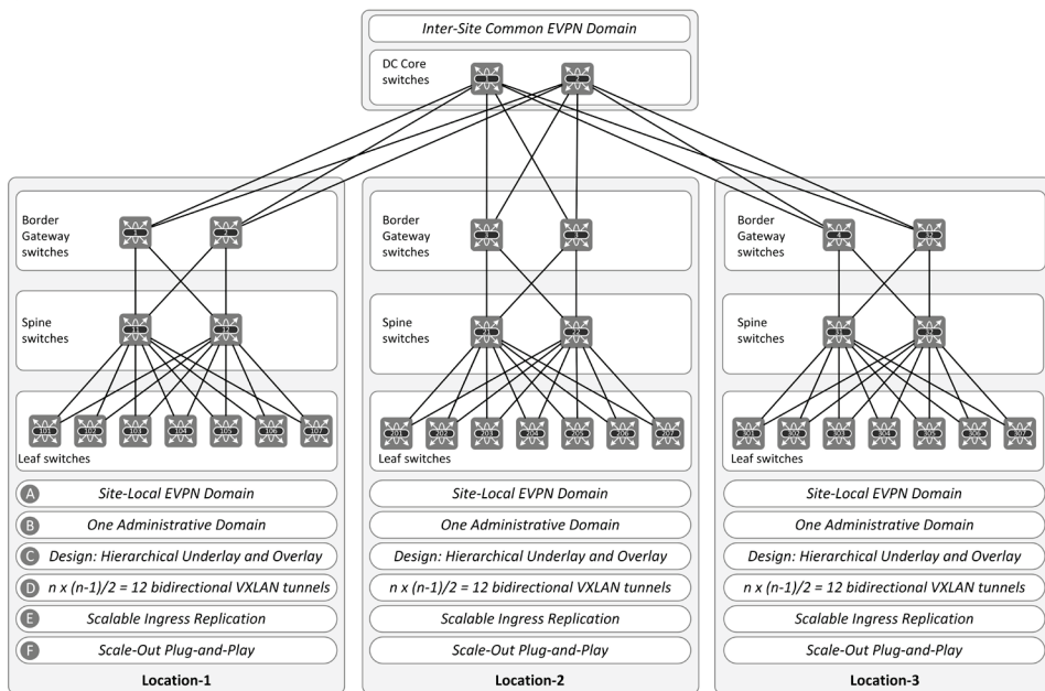
Figure 18-2: Characteristics of Super-Spine VXLAN fabric.
