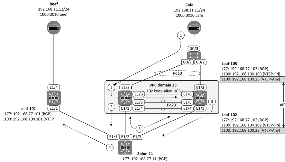
Figure 11-5: BGP EVPN Update
