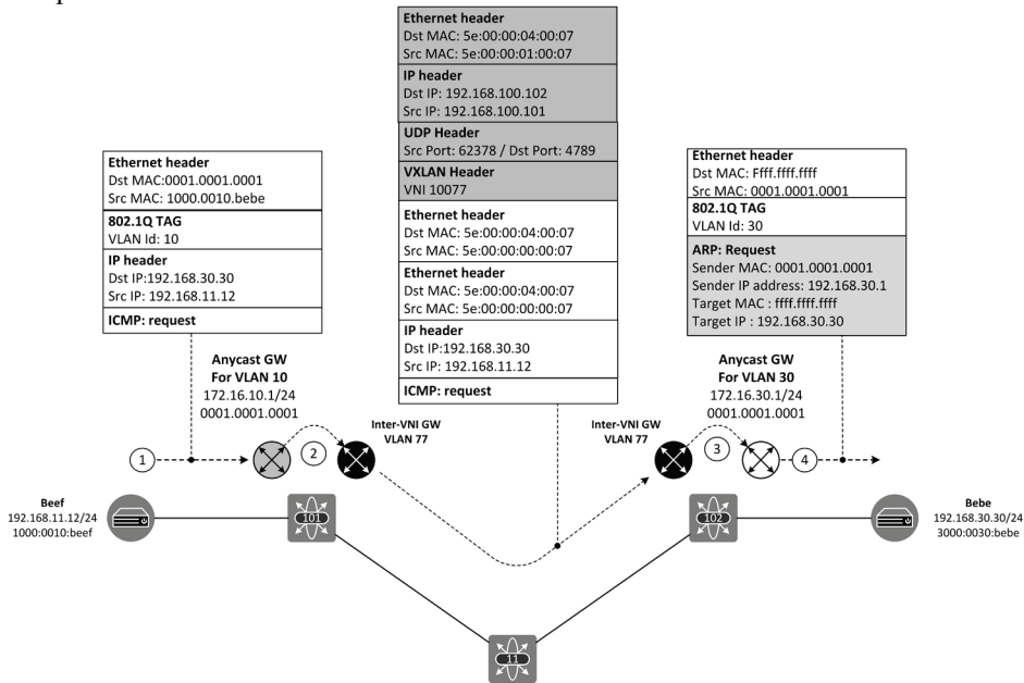
Figure 9-17: Silent host discovery process, Phases 1-4.
