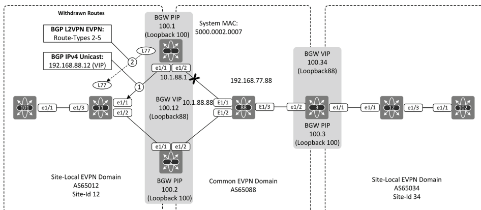
Figure 18-10: Inter-Site DCI-link failure on BGW-1.
