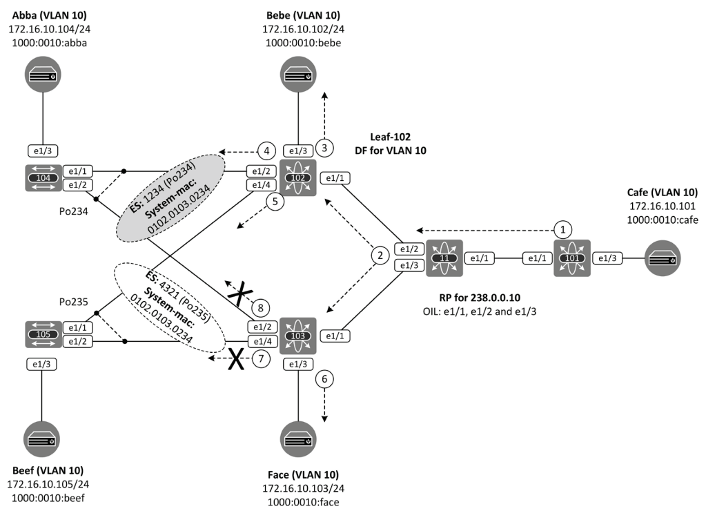
Figure 17-6: BUM from remote leaf perspective.
