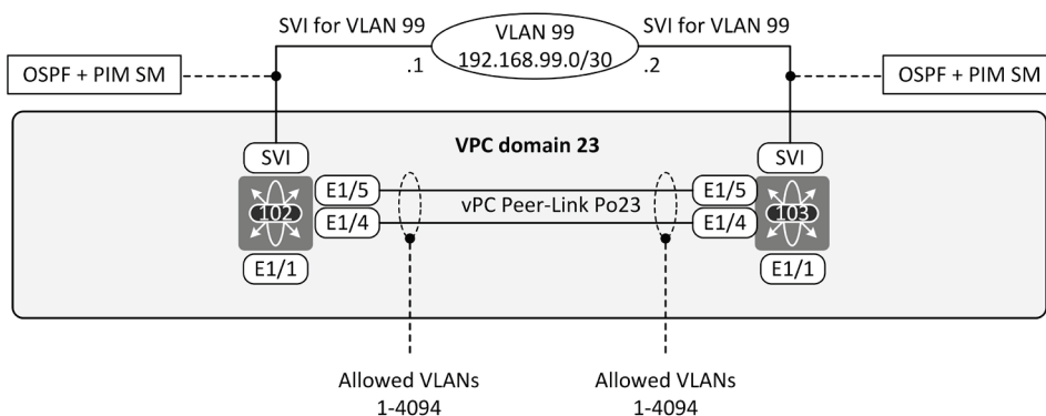
Figure 13-2: SVI for vPC Backup.
