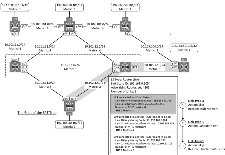
Figure 1-8: Shortest-Path Tree calculation: Third iteration round on Leaf-102.
