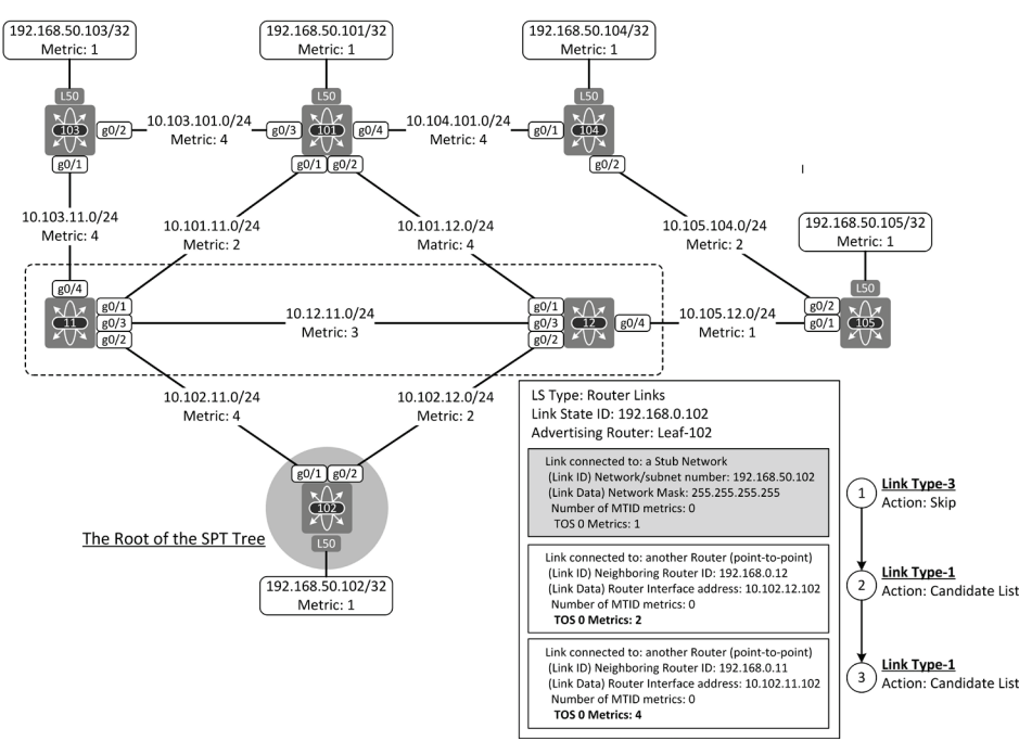
Figure 1-6: Shortest-Path Tree calculation: First iteration round on Leaf-102.
