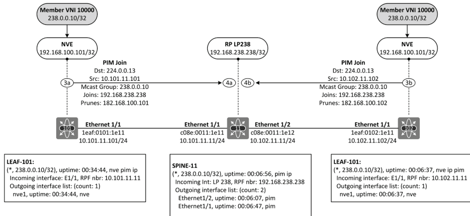
Figure 19-6: PIM-Join to Shared Tree.
