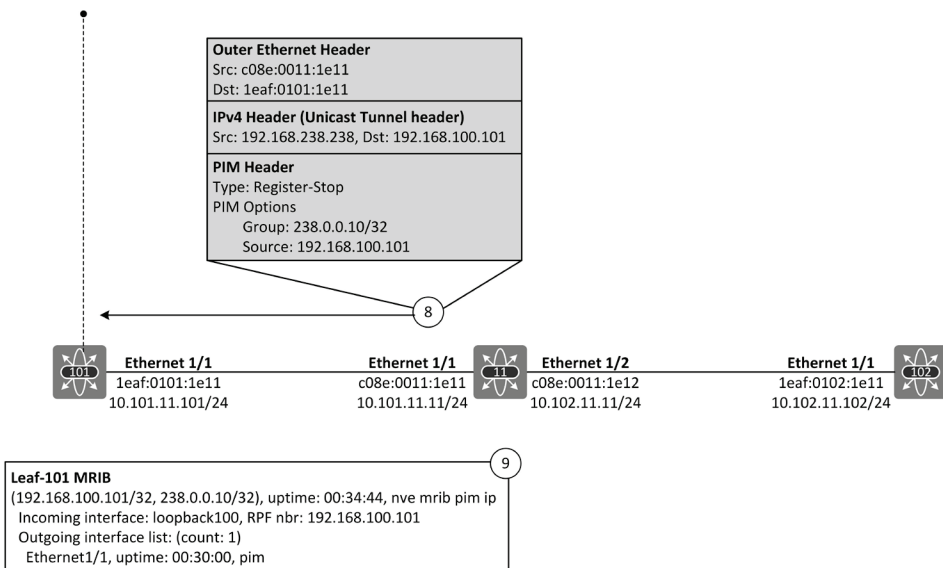
Figure 19-9: PIM Register-Stop sent by Spine-11.
