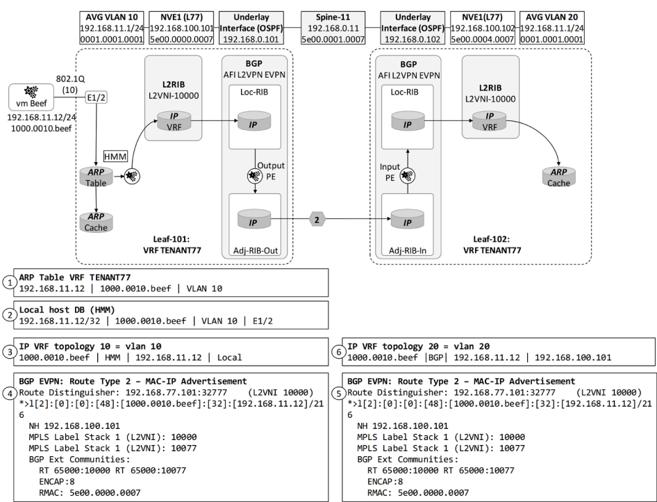
Figure 9-7: MAC-IP learning process.
