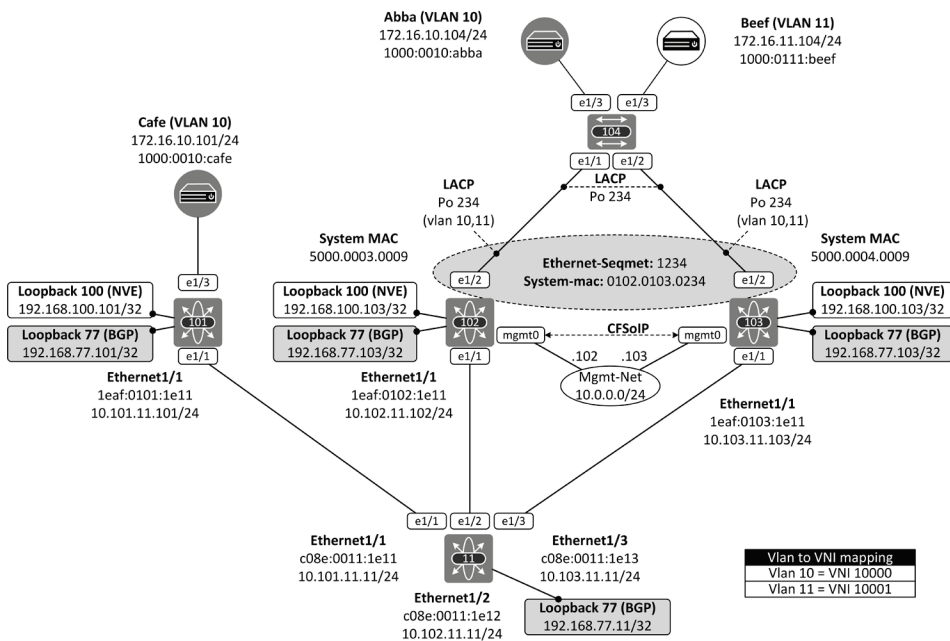
Figure 15-1: The VXLAN EVPN Multi-homing topology and addressing scheme.
