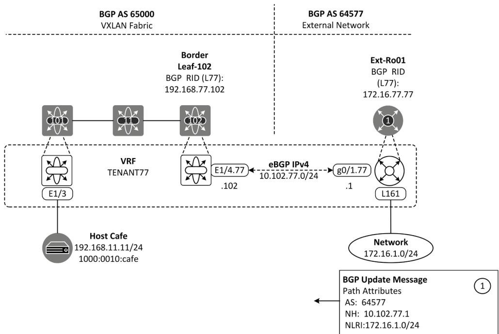
Figure 10-3: BGP Update from Ext-Ro01
