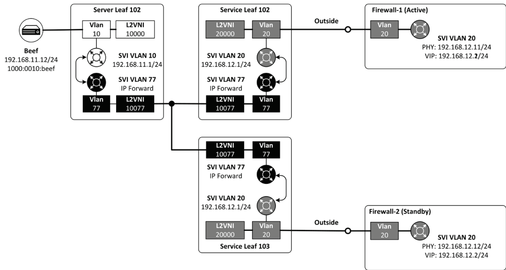
Figure 14-3: Non-protected network
