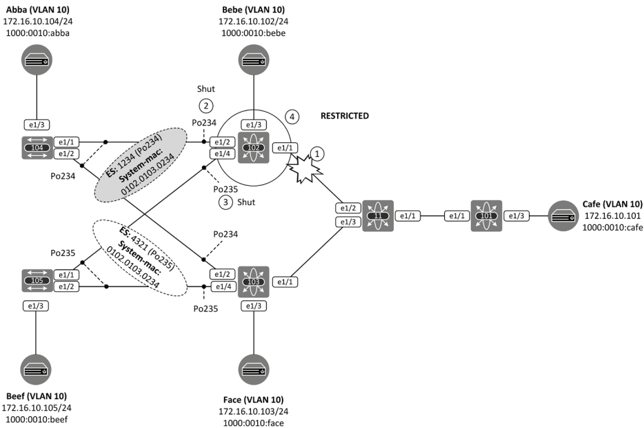
Figure 17-3: Core Link failure of Leaf-102.
