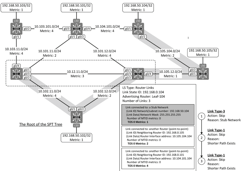
Figure 1-10: Shortest-Path Tree calculation: Fifth iteration round on Leaf-102.
