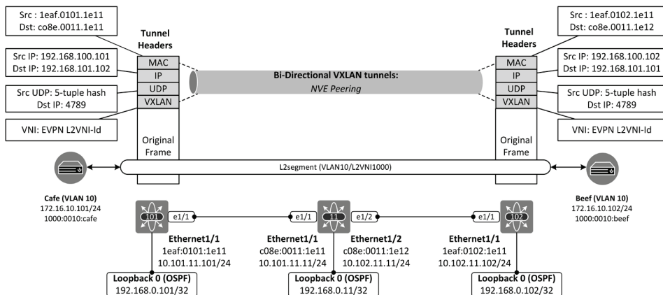
Figure 8-3: Bi-directional VXLAN tunnel.
