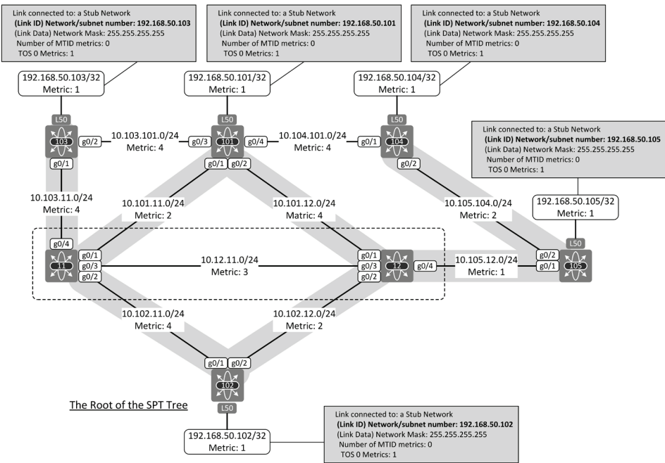
Figure 1-13: Adding leafs to Shortest-Path Tree calculation on Leaf-102.
