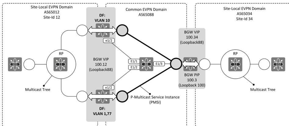
Figure 18-8: Overall Multi-Destination delivery path.
