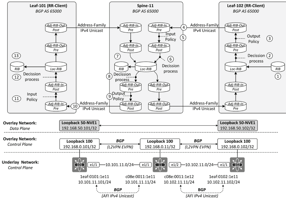
Figure 3-2: Underlay BGP process.
