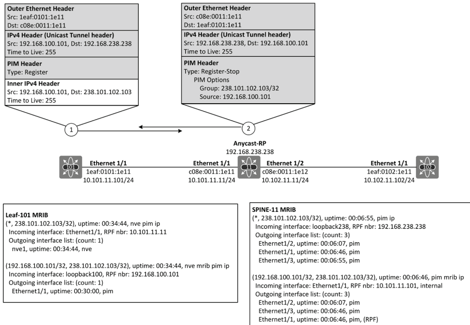
Figure 19-12: The process of building a Source-Specific Tree.
