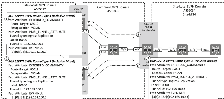
Figure 18-7: BGP L2VPN EVPN Route-Type 3 (Inclusive Multicast Ethernet Tag).
