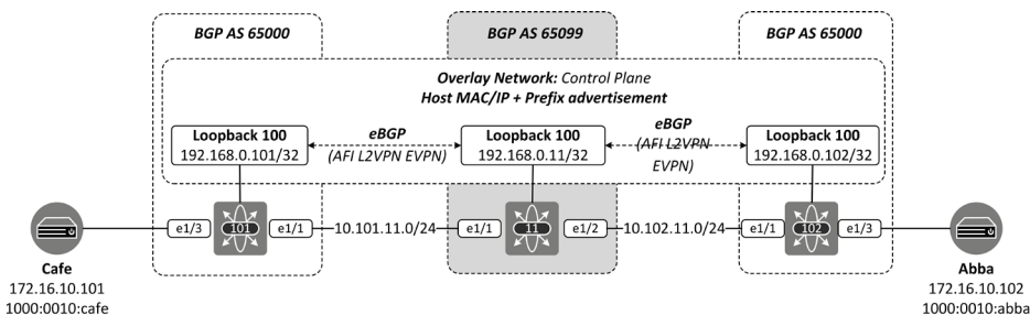
Figure 4-3: VXLAN Fabric Overlay Network eBGP L2VPN EVPN peering.
