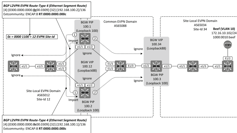
Figure 18-6: Route-Type 4 sent by BGW-1 and BGW-2.
