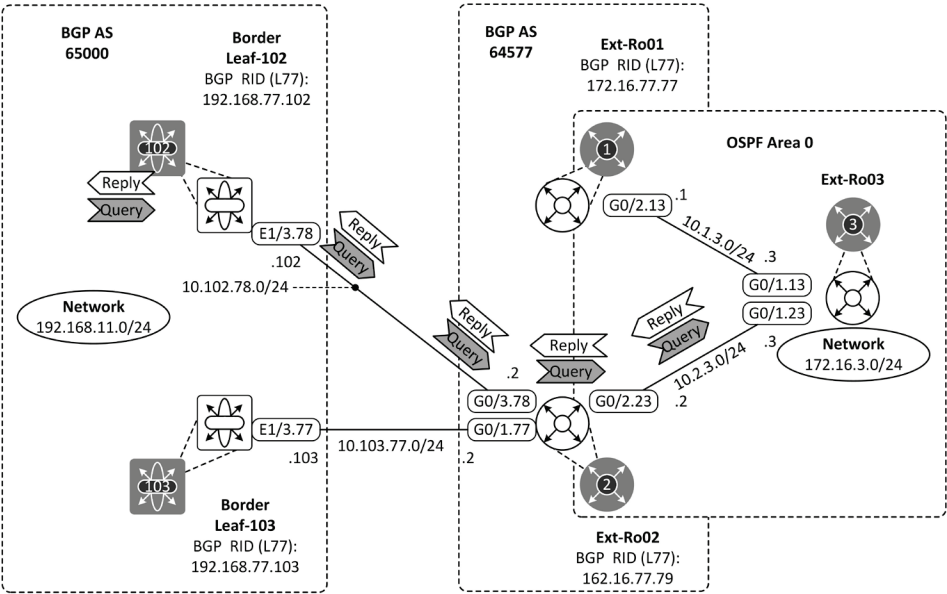
Figure 10-12: trace test#3
