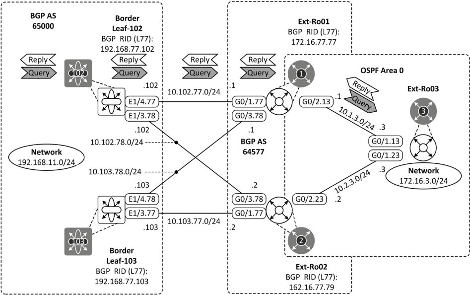
Figure 10-10: trace test#1
