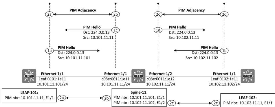
Figure 19-4: PIM neighbor establishment process.
