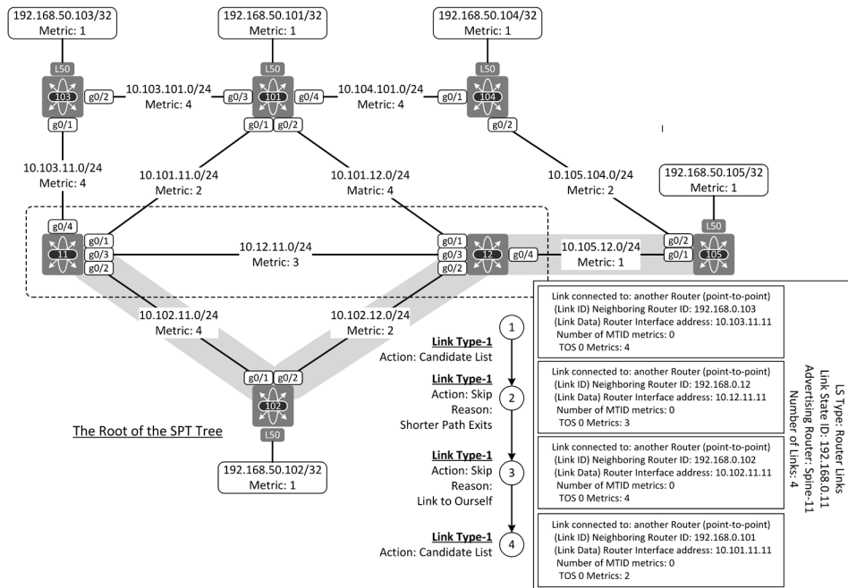
Figure 1-9: Shortest-Path Tree calculation: Fourth iteration round on Leaf-102.
