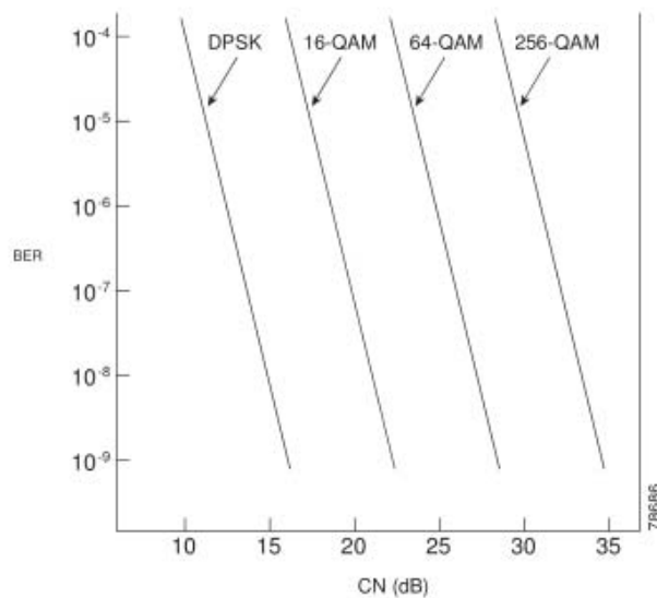
Figure 20-1 Error Rates for PSK and QAM Systems
