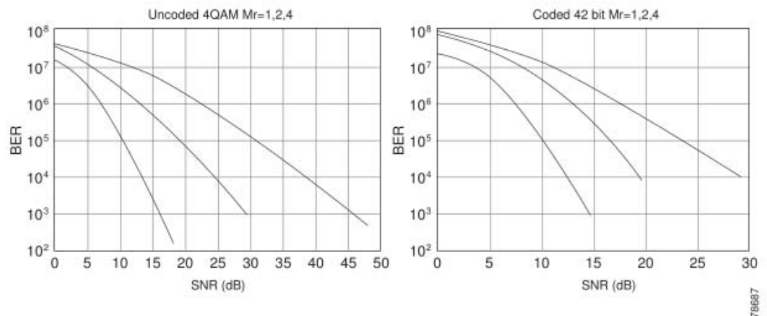
Figure 20-2 BER Against Signal-to-Noise for Coded and Uncoded Data Streams
