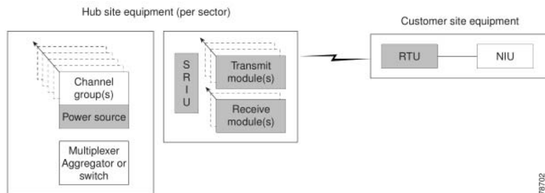
Figure 20-17 Hub Site Equipment (Per Sector)
