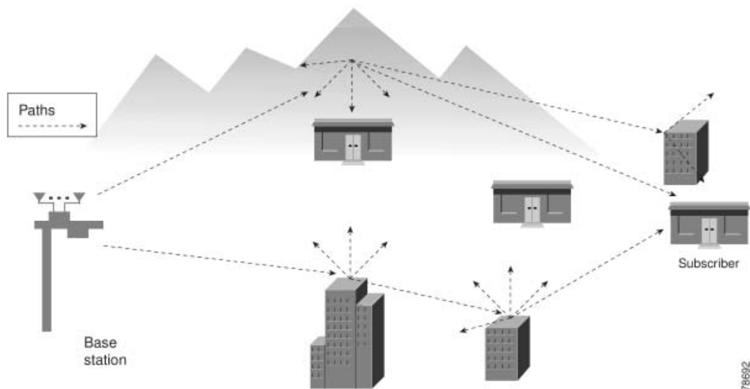
Figure 20-7 Typical Multipath Example
