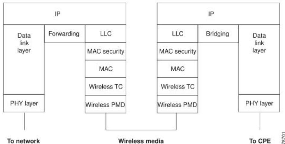
Figure 20-16 Wireless Protocol Stack for Network Management and Operation
