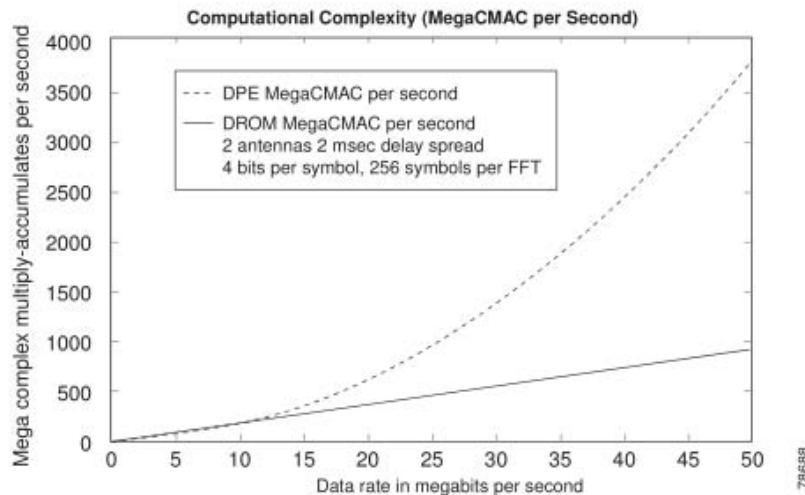
Figure 20-3 Computational Complexity of QAM Versus OFDM
