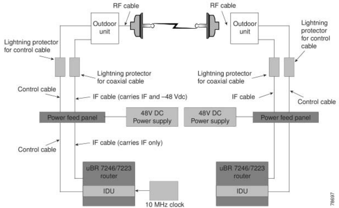
Figure 20-13 Open Standard Wireless Architecture
