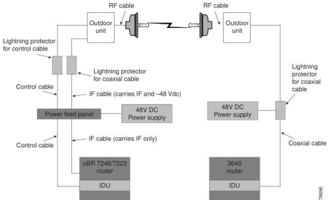
Figure 20-11 Hardware Components of the Point-to-Point System (Only One of Four Possible Sectors Shown on HE Equipment)
