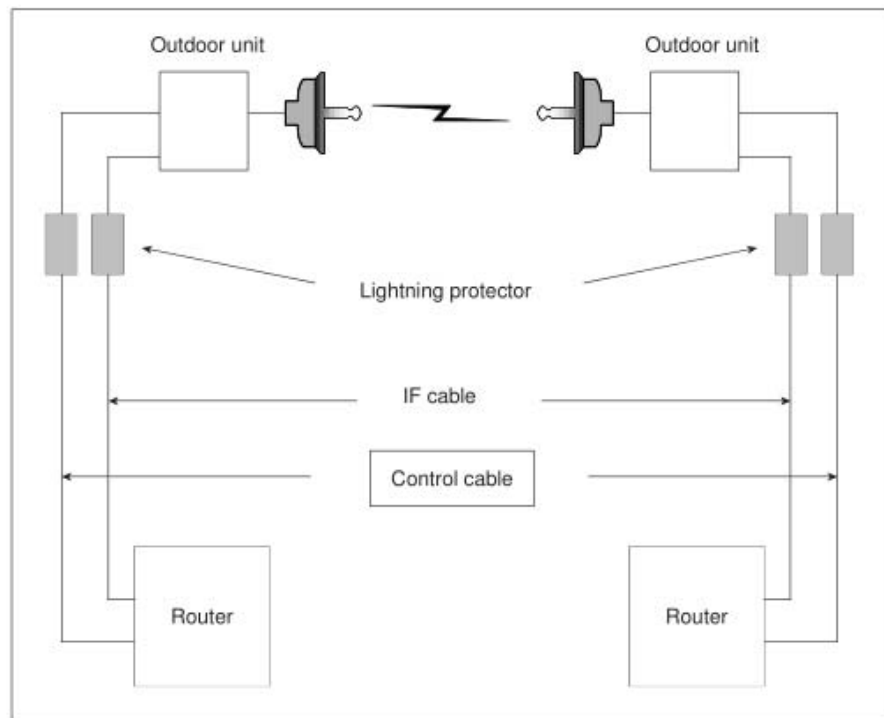
Figure 20-5 Spectrum Technology
