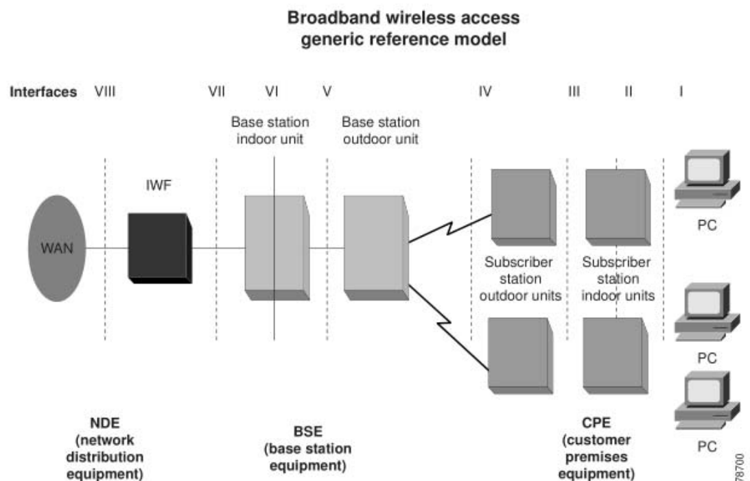
Figure 20-15 Generic Reference Model for Broadband Wireless Access
