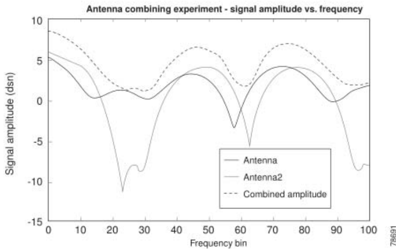
Figure 20-6 Multipath Reception
