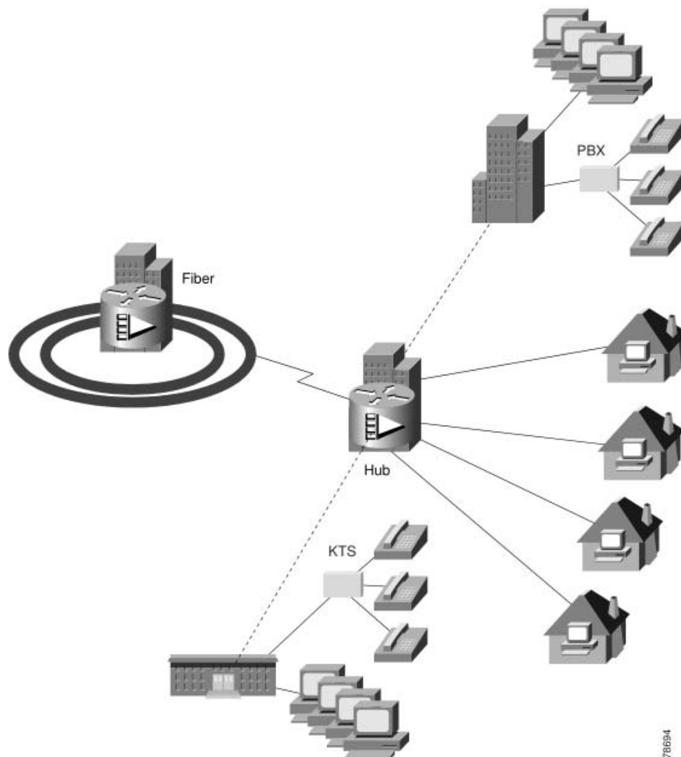
Figure 20-9 Basic Components of the P2MP Base Station (Head End, Hub)
