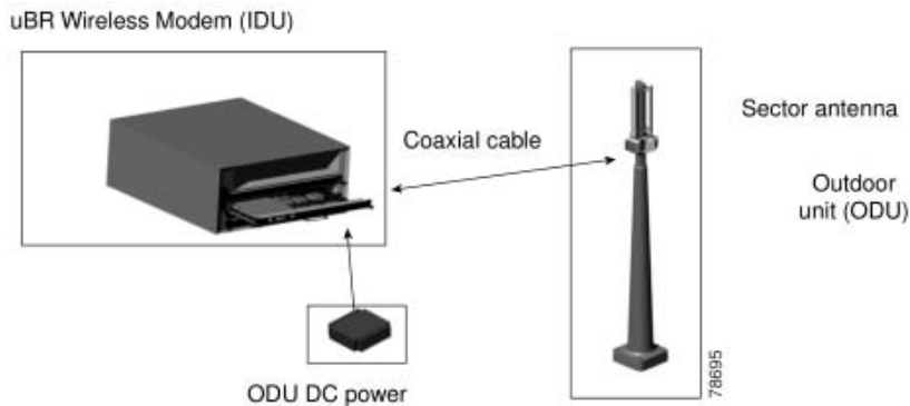
Figure 20-10 The Cisco MMDS Broadband Wireless Access System
